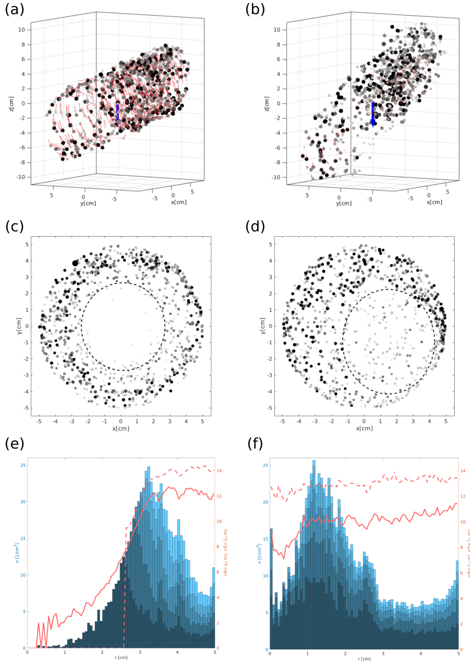
Figure 6. Positions of droplets in simulations 1) (left side) and 2) (right side) as described in Table 5 in perspective view (panels a and b) and in 4 cm-thick central slice projected on a plane perpendicular to the vortex axis (panels c and d). The blue arrow shows the direction of gravity. In panels a-d, droplet size and colour are scaled respectively to the rules described in Sec.5. The red tracks behind the particles in panels a and b reflect the last \Delta t = 0.0055 s of the droplet trajectory (for clarity every 10th droplet is drawn). The dashed circles in panels c and d reflect the approximate shape and size of the visible void in the droplet field. Panels e and f present: the number concentration of droplets n with different blue shading colors representing the contribution from different size groups - left axis, droplet mean real radius (solid red line) and mean visible radius (dashed red line) - right axis, all with respect to the distance from the vortex axis r .
