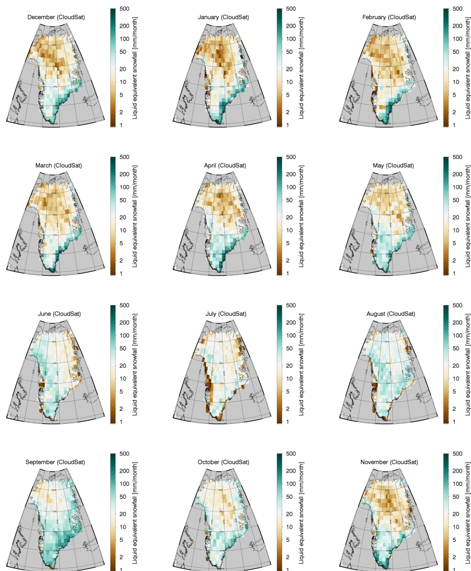
Figure 16: CloudSat-derived monthly mean snowfall rates.
