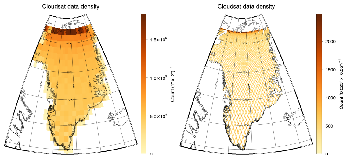
Figure 2: CloudSat data density over Greenland at 1x2 degrees (left, approximately 100 km x 100 km) and 0.025 x 0.05 degrees (right, approximately 2.5 km x 2.5 km). Shown is the total number of observations per grid box over the time period from 2006 to 2016.
