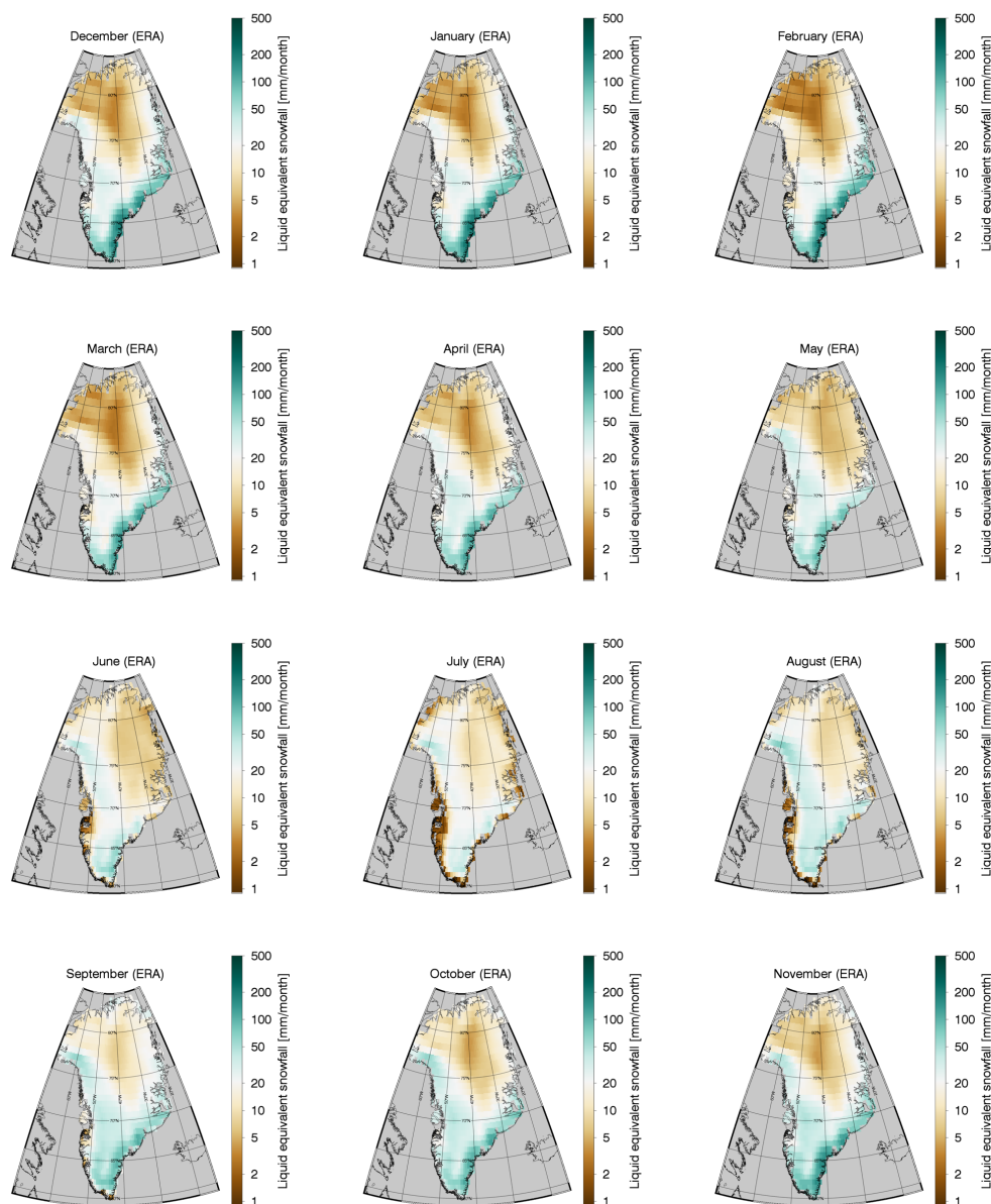
Figure 17: Same as Figure 16 but for ERA-Interim.
