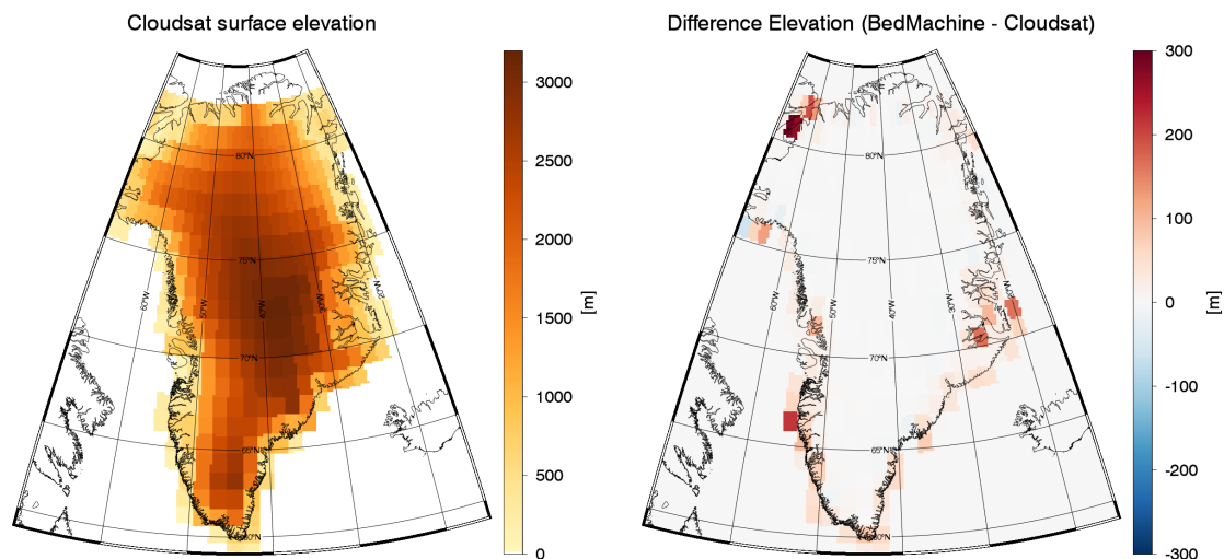
Figure 3: The left panel shows the mean elevation reported from CloudSat binned to 1 \times 2 degrees. The right panel shows the difference between the elevation difference between IceBridge BedMachine v3 (Morlighem et al., 2017) and CloudSat. Note, that open water and sea ice observations are excluded from the dataset, so that differences observed near the coast only stem from ice-free land or GrIS observations within each grid box.
