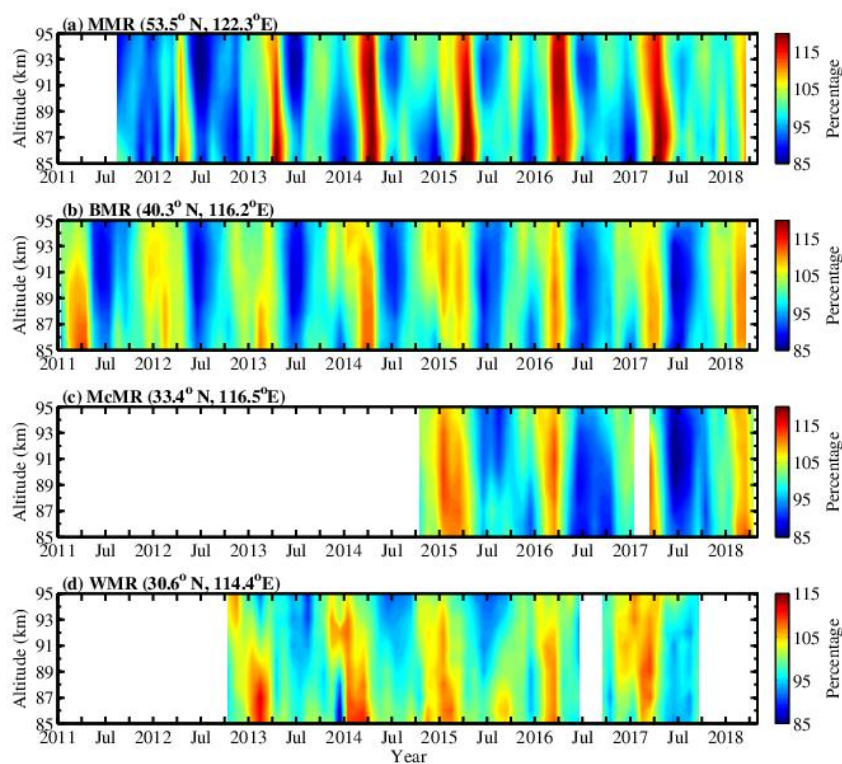
Figure 5. Same as Figure 3, but for the MMR, BMR, McMR and WMR monthly mean densities.
