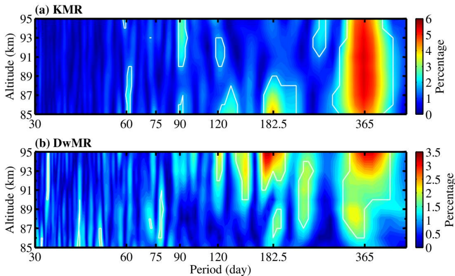
Figure 8. Same as Figure 4, but for the KMR and DwMR, daily mean relative densities at low latitudes.
