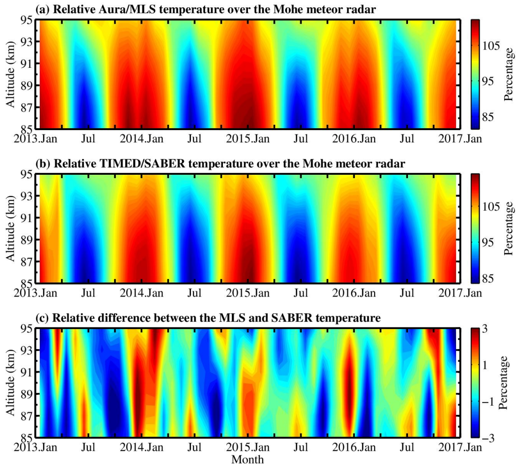
Figure R1. Variations in the monthly mean relative the (a) MLS and (b) SABER temperatures from 85 to 95 km over the Mohe meteor radar, (c) the relative difference between the MLS and SABER temperatures.
