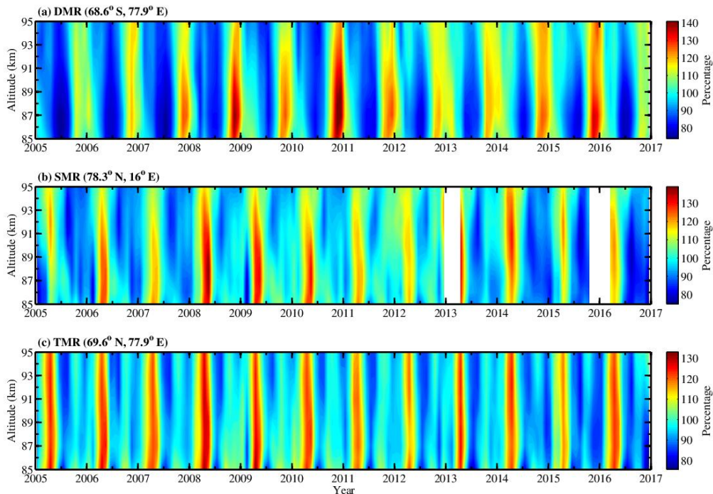
Figure 3. Variations in the monthly mean relative densities at altitudes from 85 to 95 km obtained from the DMR, SMR, and TMR between 2005 and 2016. The colour
