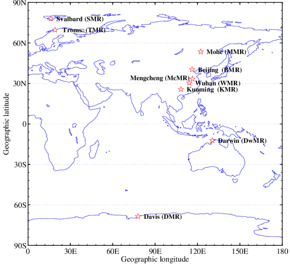
5 Figure 1. The locations of the meteor radars used in this study.
