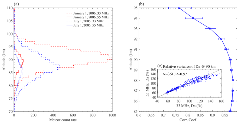
15 Figure 2. (a) The height distributions of meteor detections in 1 km bins on January 1 and July 1 in 2006 from the 33 MHz and 55 MHz meteor radars at Davis Station. (b) Height variation in the correlation coefficient between the D_a observed simultaneously by the 33 MHz and 55 MHz meteor radars at Davis Station in 2006. The error bars indicate the lower and upper bounds of the 95% confidence interval for each coefficient. (c) Comparison of the variations in the daily mean D_a (blue dots) at 20 90 km simultaneously observed from the 33 MHz and 55 MHz meteor radars at Davis
