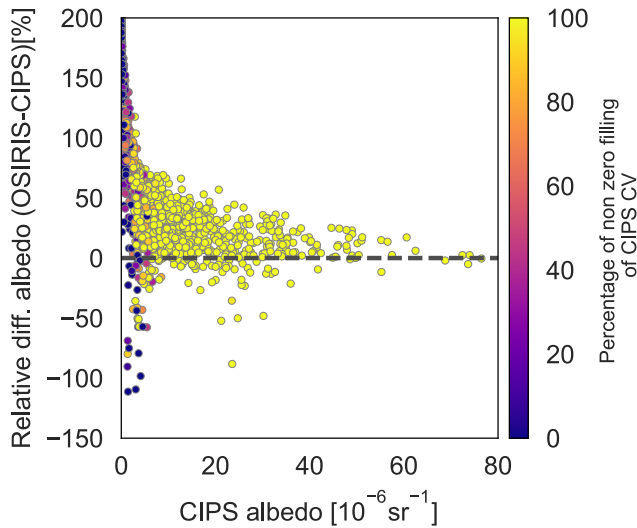
Figure 5: Relative difference in cloud albedo in CV elements 2 \times (\text{OSIRIS} - \text{CIPS}) / (\text{CIPS} + \text{OSIRIS}) vs CIPS albedo. The points are color-coded by the percentage of filling of non-zero pixels in a CIPS CV element.
