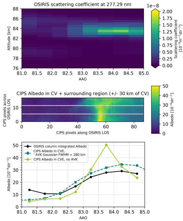
5 Figure 8: Common volume observations of cloud albedo for OSIRIS orbit 51236 and CIPS orbit 17556. The coincidence occur at latitude 78°N and longitude 150° at 15.45 local time. The top panel shows OSIRIS cloud scattering coefficient (vertical plane) for the subset of the orbit that overlaps CIPS orbit strip. The middle panel shows CIPS albedo (horizontal plane) for the subset of pixels that overlap OSIRIS field of view along OSIRIS LOS. The pink lines denote the width of OSIRIS LOS, and consequently the CIPS pixels within the pink lines that are contained in the CV. The region +/-30 km outside the CV is included only for illustrative purposes. The abscissa in the middle panel is given in CIPS pixels along OSIRIS LOS, hence identical with the abscissa in the top panel. The bottom panels shows the resulting albedo in the CV for the integrated signal from each instrument along the abscissa AAO.
