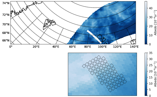
15 Figure 1: Example orbit showing a CIPS/OSIRIS coincidence on a polar map plot for CIPS orbit 50777 and OSIRIS orbit 17098. The top panel shows the CIPS orbit strip. The white line on top of the CIPS orbit strip indicates the overlapping ~660 CIPS pixels in the CV. Each CV is composed of ~10 CV elements. The bottom panel shows an example of only those 66 pixels contained within one CV element.
