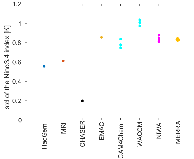
Figure 1. Standard deviation of surface temperature in the Nino3.4 region in the CCM1 models. The multiple dots for NIWA, WACCM and CAM4Chem represent different integrations of the same model. The standard deviations in CHASER is much less than that observed, and hence this model was excluded from further analysis.
