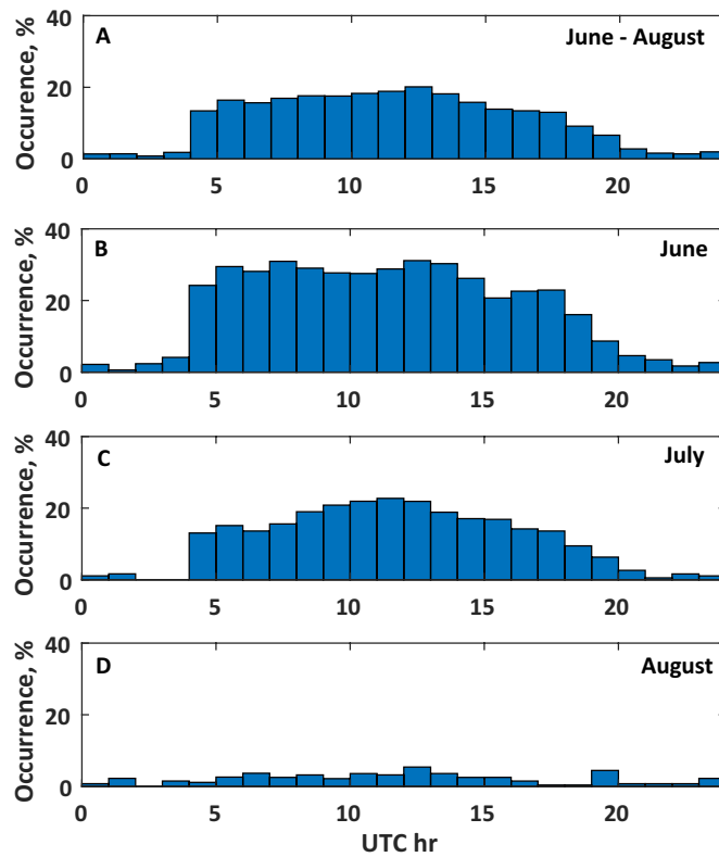
Figure 1. 24-hour composites of MSE occurrences (with respect to 00 UTC time) for all days of summer (Panel A), and the days of June, July, and August (Panels B, C, and D, respectively).
