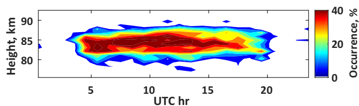
Figure 3. 24-hour composites of MSE occurrences as function of UTC time and the height of detected echoes.
