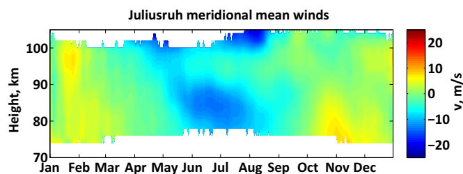
Figure 2. Climatology of meridional mean winds obtained from Juliusruh meteor radar observations over years 2007-2016.
