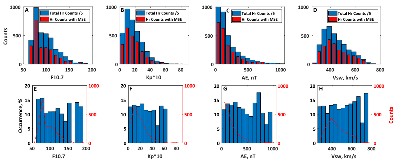
Figure 5. Dependencies of MSEs on solar and geomagnetic activity, manifested by 10.7 cm solar radio flux F_{10.7} in solar flux units (Panels A, E), planetary 3-hour-range index Kp (Panels B, F), auroral electrojet index AE (Panels C, G), and solar wind speed V_{SW} (Panels D, H). In the top row (Panels A–D), the total counts of OSWIN observation hours is shown by blue bars, and the counts of hours with MSEs detected is shown by red bars (note that the number of total counts is divided by a factor of 5). In the bottom row (Panels E–H), the occurrences of MSEs in each bin of solar/geomagnetic indices are shown by blue bars, and the red lines indicate the number of counts with MSEs detected.
