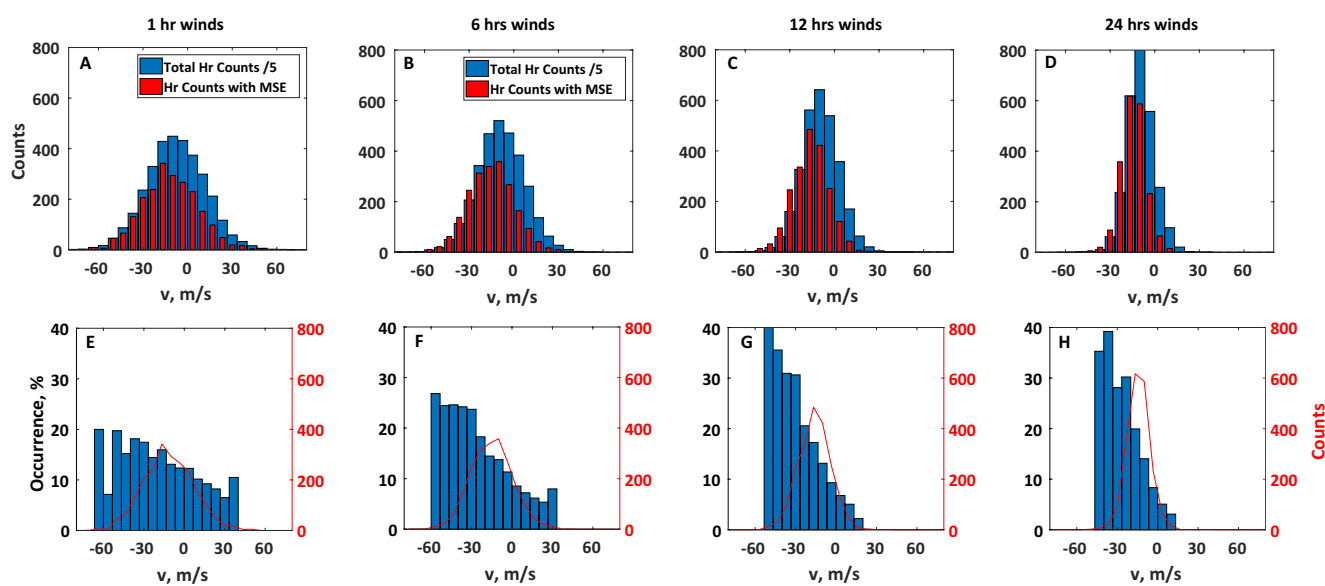
Figure 6. Dependencies of MSEs on meridional wind transport, quantified by the hourly meridional winds obtained by the Juliusruh meteor radar. In the top row (Panels A-D), the total counts of OSWIN observation hours (divided by a factor of 5) are shown by blue bars for each bin of meridional wind speed, and the counts of hours with MSEs detected are shown by red bars. In the bottom row (Panels E-H), the occurrences of MSEs vs meridional wind are shown by blue bars, and the red lines indicate the number of counts with MSEs detected.
