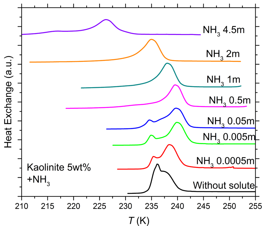
105 Figure 7. DSC thermograms of 5 wt % kaolinite particles suspended in ammonia solution droplets (0 - 4.5 molal; a_w = 1 - 0.922 ). All curves are normalized such that the areas under the heterogeneous and homogeneous freezing curves sum up to the same value.
