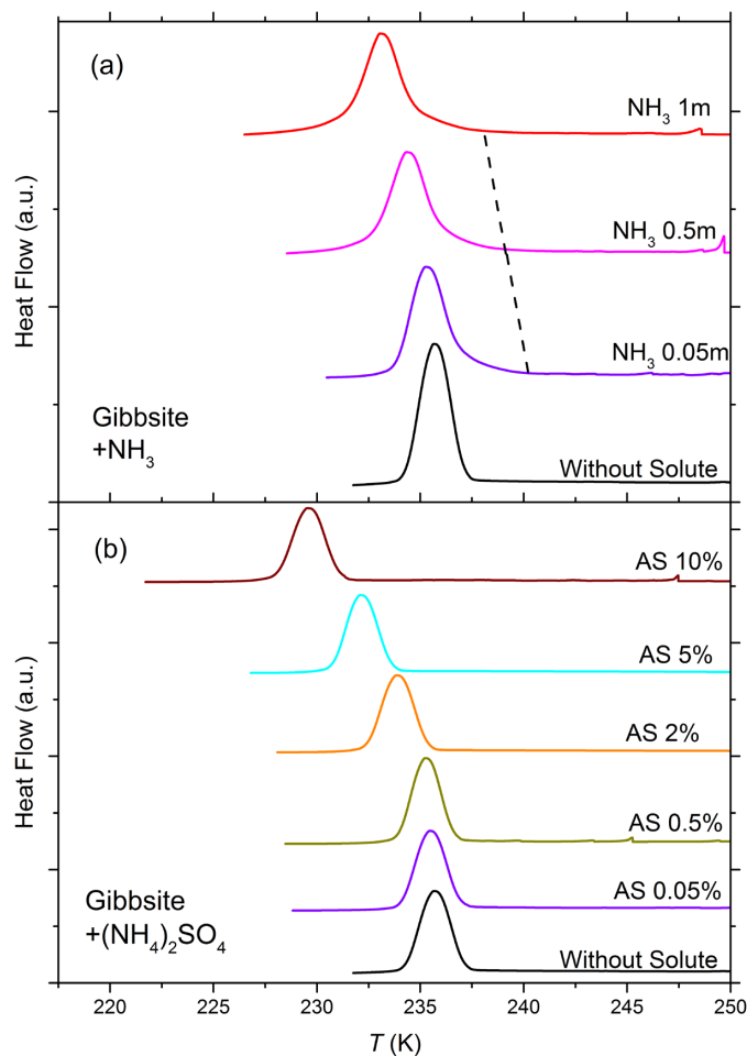
Figure 6. DSC thermograms of 10 wt % gibbsite suspended in ammonia solution droplets (panel a) of concentrations from 0 to 1 molal ( a_w = 1 - 0.981 ) and (\text{NH}_4)_2\text{SO}_4 solution droplets (panel b) from 0 to 10 wt % ( a_w = 1 - 0.961 ). All curves are normalized such that the areas under the heterogeneous and homogeneous freezing curves sum up to the same value. Gibbsite shows no discernible heterogeneous freezing signal in pure water and starts to show a weak heterogeneous freezing signal when suspended in ammonia solution (dashed black line connects the onset of heterogeneous freezing signals), while no heterogeneous IN is observed for gibbsite suspended in (\text{NH}_4)_2\text{SO}_4 .
