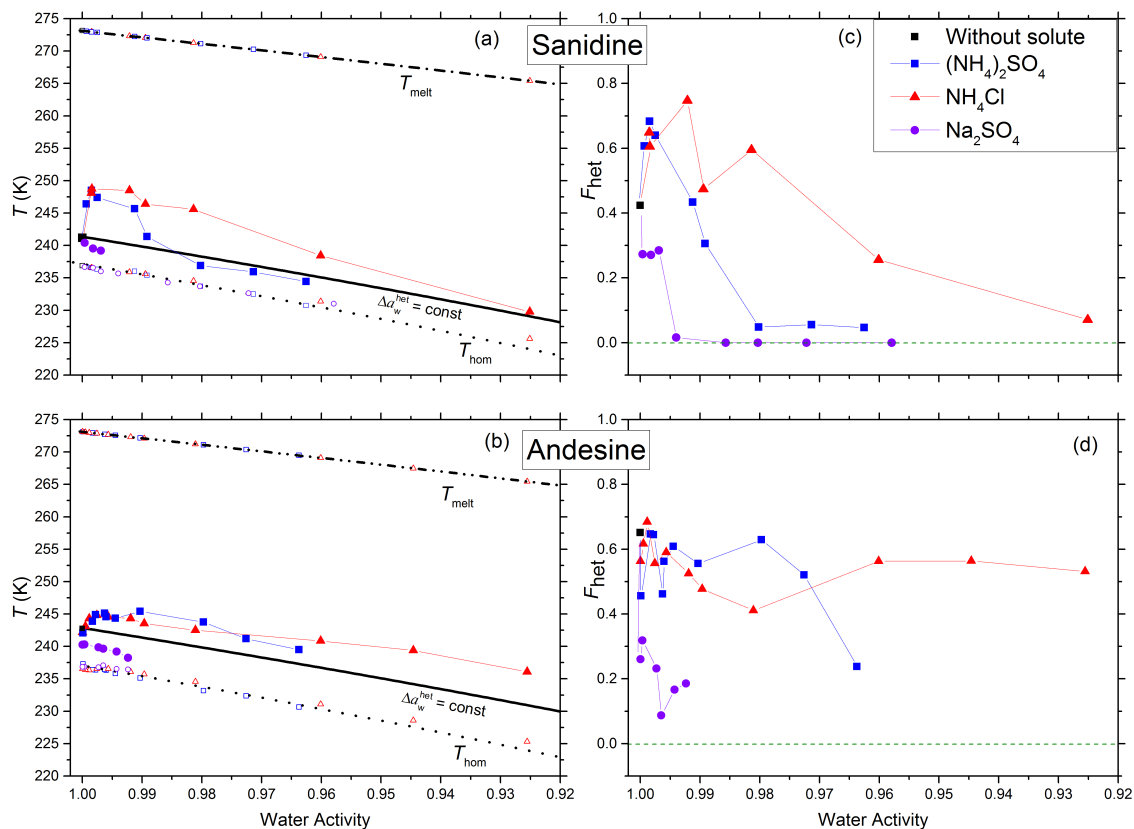
Figure 2. Measured freezing temperatures (left) and heterogeneously frozen fractions (right) of emulsion freezing experiments with 2 wt % feldspar, namely sanidine (panels a and c) and andesine (panels b and d), in various solutions (color-coded). Left: Heterogeneous freezing onset temperatures, T_{\text{het}} (filled solid symbols connected by thin lines to guide the eye), homogeneous freezing onset temperatures, T_{\text{hom}} (open symbols at T < 237 K), and ice melting temperatures, T_{\text{melt}} (open symbols at T > 265 K) as functions of water activity of solutions, a_w , for various solutes (symbols and colors see insert). Dash-dotted black line: ice melting point curve. Dotted black line: homogeneous ice freezing curve for supercooled aqueous solutions obtained by horizontally shifting the ice melting curve by a constant offset \Delta a_w^{\text{het}}(T) = 0.294 . Solid black line: horizontally shifted from the ice melting curve by \Delta a_w^{\text{het}}(T) = 0.264 and 0.254 for sanidine (panel a) and andesine (panel b), respectively, with offsets derived from the heterogeneous freezing temperature of the suspension of the mineral in pure water (filled black square at a_w = 1 ). Symbols are the mean of at least two separate emulsion freezing experiments. Difference between the two measurements plus instrumental uncertainty in T_{\text{het}} and a_w are smaller than the symbol size (see Sect 2.2). Right: Heterogeneously frozen fraction, F_{\text{het}} , as function of a_w , for sanidine (panel c) and andesine (panel d). Measurement difference and uncertainty in F_{\text{het}} do not exceed \pm 0.1 .
