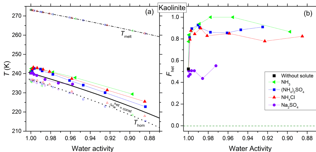
70 Figure 3. Same as Fig. 2, but for kaolinite (5 wt %). (a) Homogeneous ice freezing curve (dotted black line) characterized by a constant offset \Delta a_w^{\text{hom}}(T) = 0.294 . Ice melting curve (dash-dotted black line) and the heterogeneous freezing curve (solid black line) horizontally shifted from the ice melting curve by \Delta a_w^{\text{het}}(T) = 0.272 derived from the heterogeneous freezing temperature of the suspension of the mineral in pure water (filled black square at a_w = 1 ). Measured differences and instrumental uncertainties in T_{\text{het}} and a_w are smaller than the symbol size (see Sect. 2.2). (b) F_{\text{het}} (heterogeneously frozen fraction) as function of water activity of the solutions. Measurement difference and uncertainty in F_{\text{het}} do not exceed \pm 0.1 .
