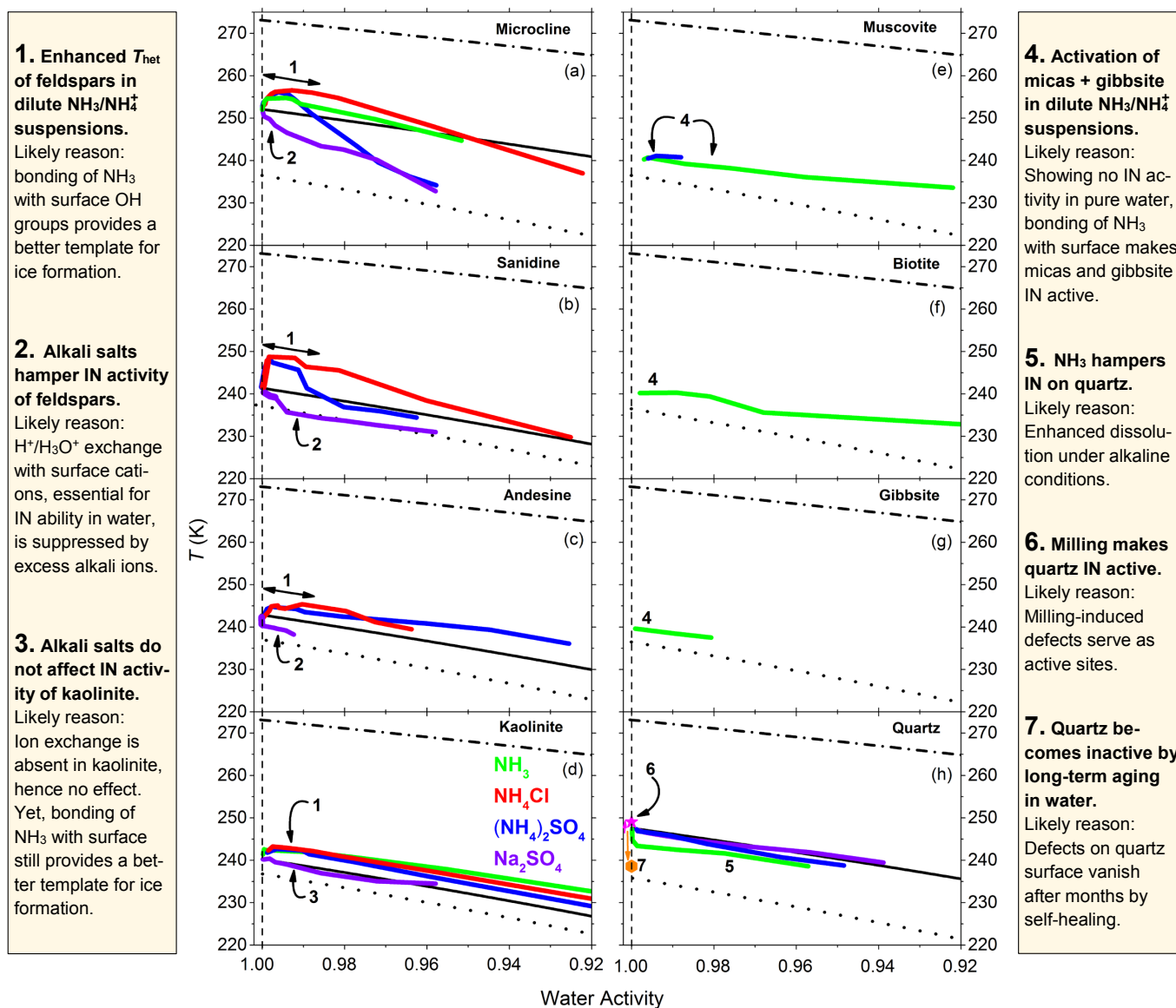
Figure 9. Annotated summary: heterogeneous IN onset temperatures, T_{het} , of various mineral dusts (2 – 10 wt%) as function of water activity in NH_3 , (NH_4)_2SO_4 and Na_2SO_4 solutions (color-coded) for a_w = 1.0 - 0.92 . (a) Results for microcline from Kumar et al. (2018a). (b)-(g) Feldspars, kaolinite, micas and gibbsite investigated in the present study. (h) Results for quartz from Kumar et al. (2018b). Dash-dotted black lines: ice melting point curves. Dotted black lines: homogeneous ice freezing curves for supercooled aqueous solutions. Solid black lines: expected heterogeneous freezing curves, if the presence of solutes did not change the mineral surface properties. Lines result by horizontally shifting from the ice melting curve by a constant \Delta a_w^{het} emanating from the heterogeneous freezing temperatures of the suspensions of the minerals in pure water (at a_w = 1 ). Specifically,
