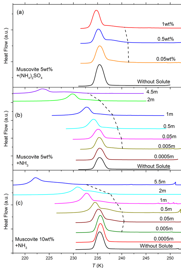
Figure 4. DSC thermograms of 5 wt % (panels a and b) and 10 wt% (panel c) muscovite particles suspended in ammonia (0 - 5.5 molal; a_w = 0.999 - 0.912 ) and ammonium sulfate (0 - 1 wt %; a_w = 0.996 - 0.988 ) droplets of different solution concentrations (given as inserts). All curves are normalized such that the areas under the heterogeneous and homogeneous freezing curves sum up to the same value. The dashed black line connects the heterogeneous freezing onset temperatures ( T_{\text{het}} ) of the emulsions. With increasing ammonia concentration heterogeneous IN efficiency starts to develop, as can be noticed from the appearance of T_{\text{het}} which was absent in pure water. The intensity of the heterogeneous freezing signal, hence F_{\text{het}} becomes more prominent in 10 wt % suspensions (see Table 1).
