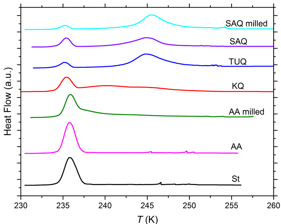
Figure 1. DSC thermograms of various quartz and amorphous silica particles suspended in pure water. St: Stöber silica (10 wt%); AA: Alfa Aesar silica (10 wt%); AA milled: milled Alfa Aesar silica (10 wt%); KQ: quartz sample from Kaufmann et al. (2016) (8–9 wt%); TUQ: TU Vienna quartz (5 wt%); SAQ: Sigma-Aldrich quartz (5 wt%, milled by Sigma-Aldrich); SAQ milled: additionally milled Sigma-Aldrich quartz (5 wt%). All curves are normalized such that the total areas under the heterogeneous plus homogeneous freezing curves sum up to the same value.
