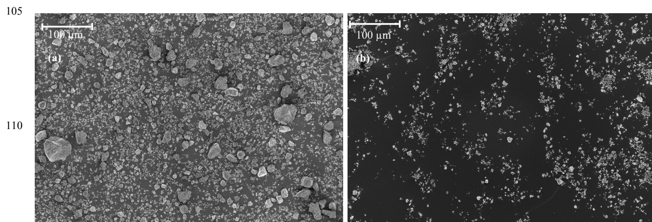
115 Figure A1. SEM images of two different quartz samples at 500X magnification. (a) Quartz sample from Kaufmann et al., (2016); (b) Quartz sample (from Sigma Aldrich) used in this study.
