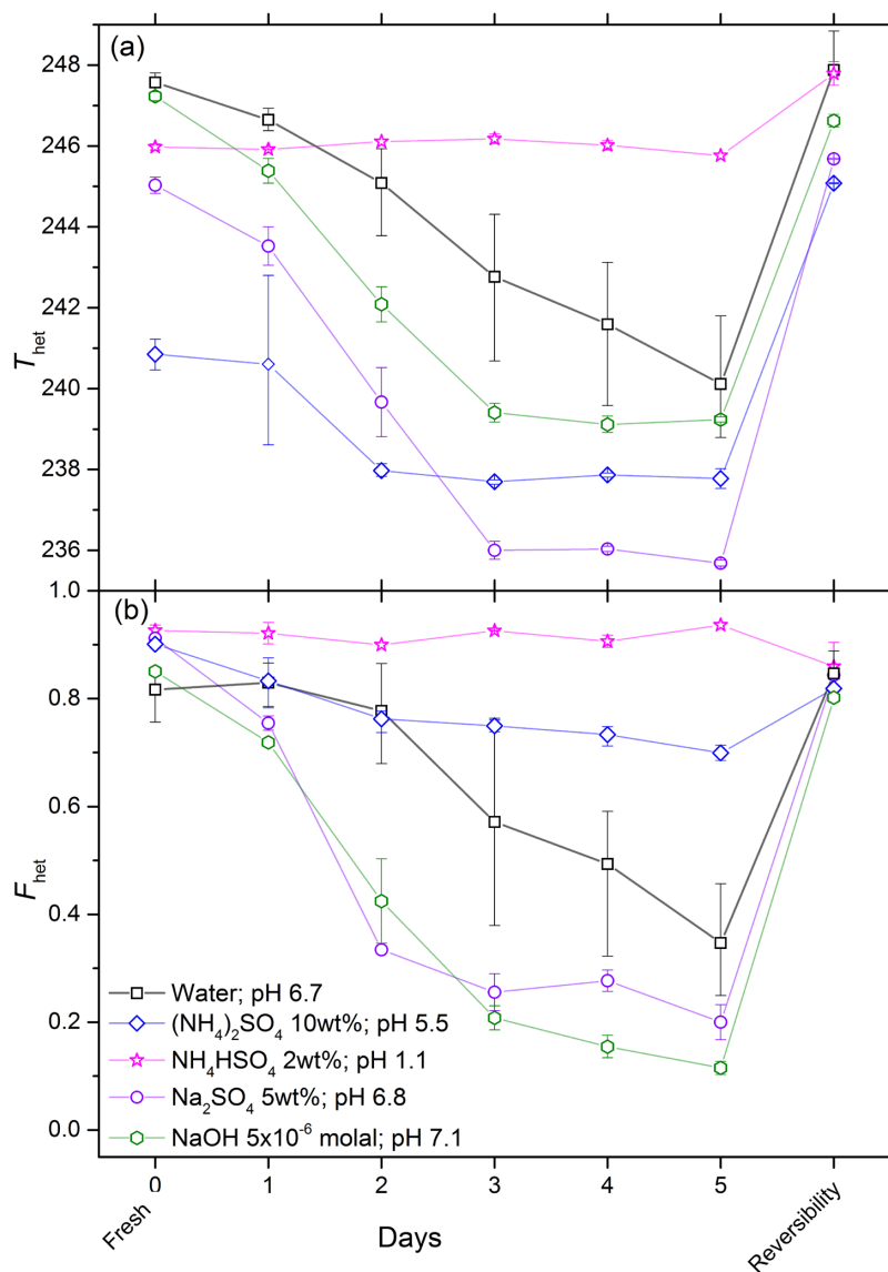
85 Figure 5. Development of T_{het} (panel a) and F_{het} (panel b) for 5 wt% SA quartz suspended in water, (NH_4)_2SO_4 solution (10 wt%), NH_4HSO_4 solution (2 wt %), Na_2SO_4 solution (5 wt %) and NaOH solution ( 5 \times 10^{-6} molal) over a period of five days. All suspensions were prepared and aged in borosilicate glass vials. After five days of aging the reversibility was tested: the suspensions were centrifuged, the supernatant decanted, the aged particles washed several times with pure water, resuspended in pure water, and subjected to an emulsion freezing experiment. All data points are means of at least two separately aged suspensions. The error bars show representative experimental variations (min-to-max).
