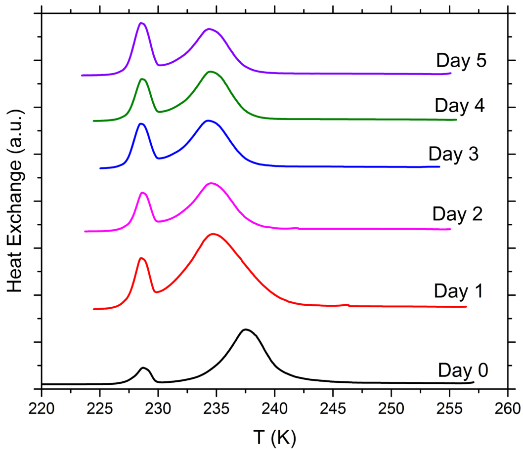
Figure S6. DSC thermograms of aging tests with 5 wt% SA quartz particles suspended in 10 wt% ammonium sulfate solution droplets measured over a period of 5 days. All curves are normalized such that the areas under the heterogeneous and homogeneous freezing curves sum up to the same value.
