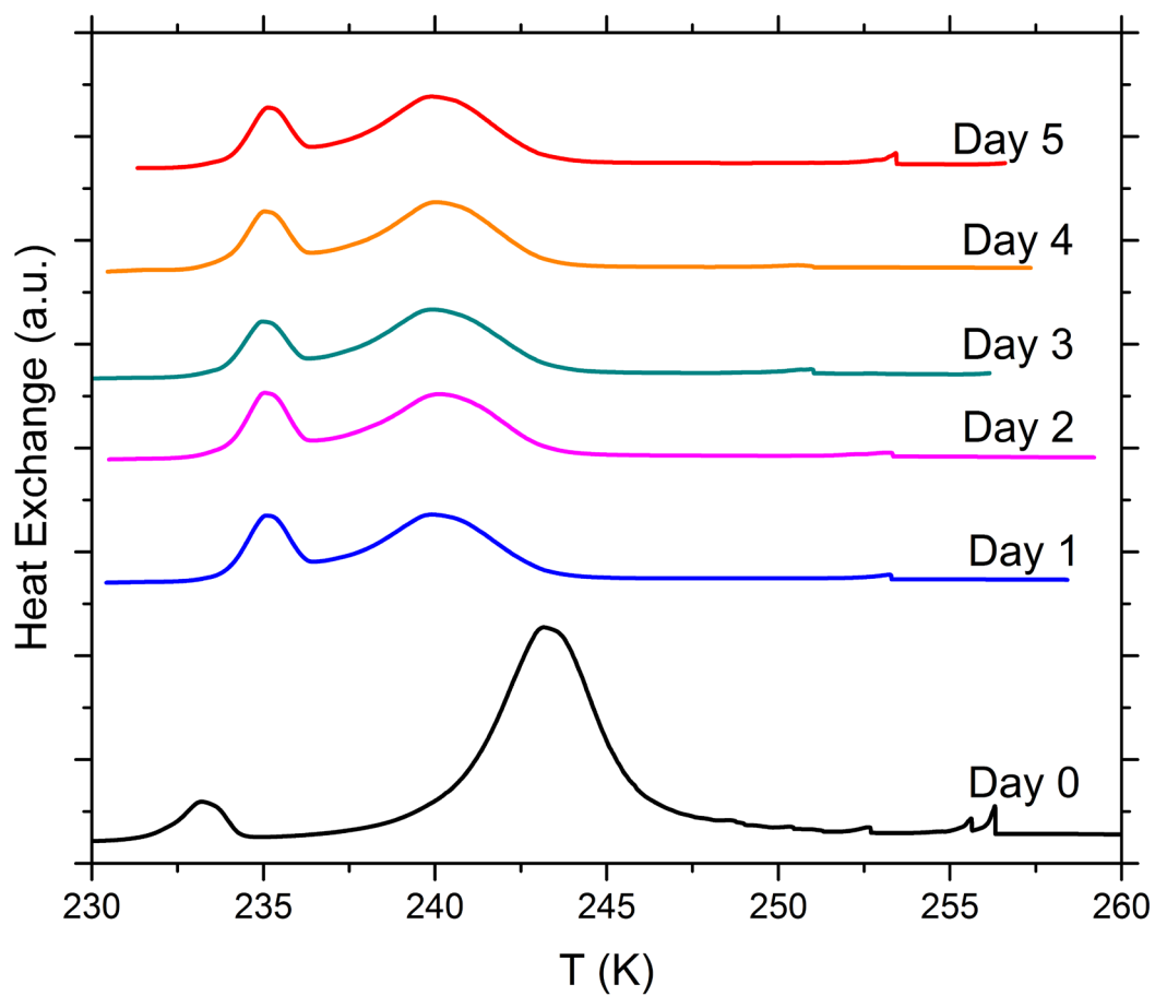
Figure S8. DSC thermograms of aging tests with 5 wt% SA quartz particles suspended in 0.005 molal ammonia solution droplets measured over a period of 5 days. All curves are normalized such that the areas under the heterogeneous and homogeneous freezing curves sum up to the same value.
