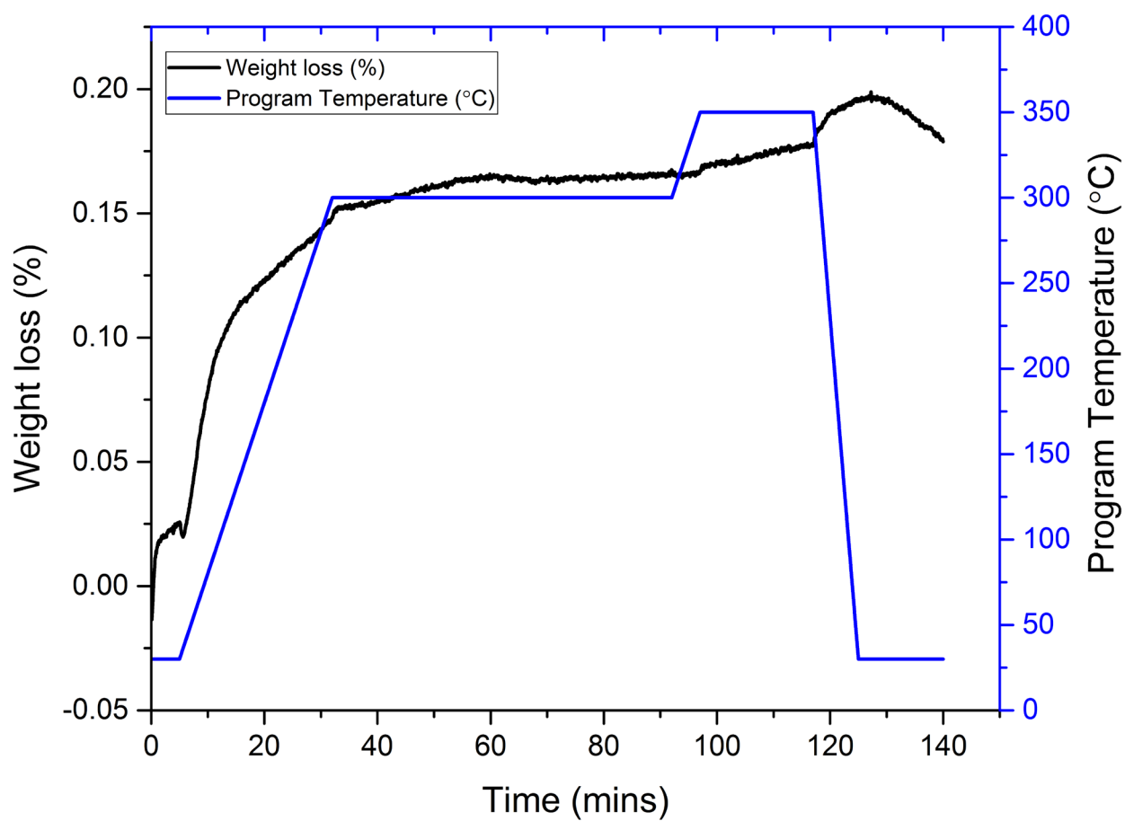
Figure S26. Mass loss of the TU Vienna sample measured by thermogravimetric analysis.. Blue line: temperature (°C); black line: sample weight loss (in %). A minor loss of up to 0.2% in weight was observed.
