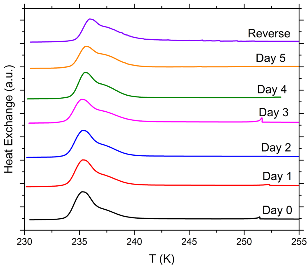
Figure S21. DSC thermograms of aging and reversibility tests on suspensions with 5 wt% SA quartz particles prepared in polypropylene vials and aged for 5 days in sodium hydroxide solution (0.005 molal). Aged particles were collected after aging and resuspended in pure water. All curves are normalized such that the areas under the heterogeneous and homogeneous freezing curves sum up to the same value.
