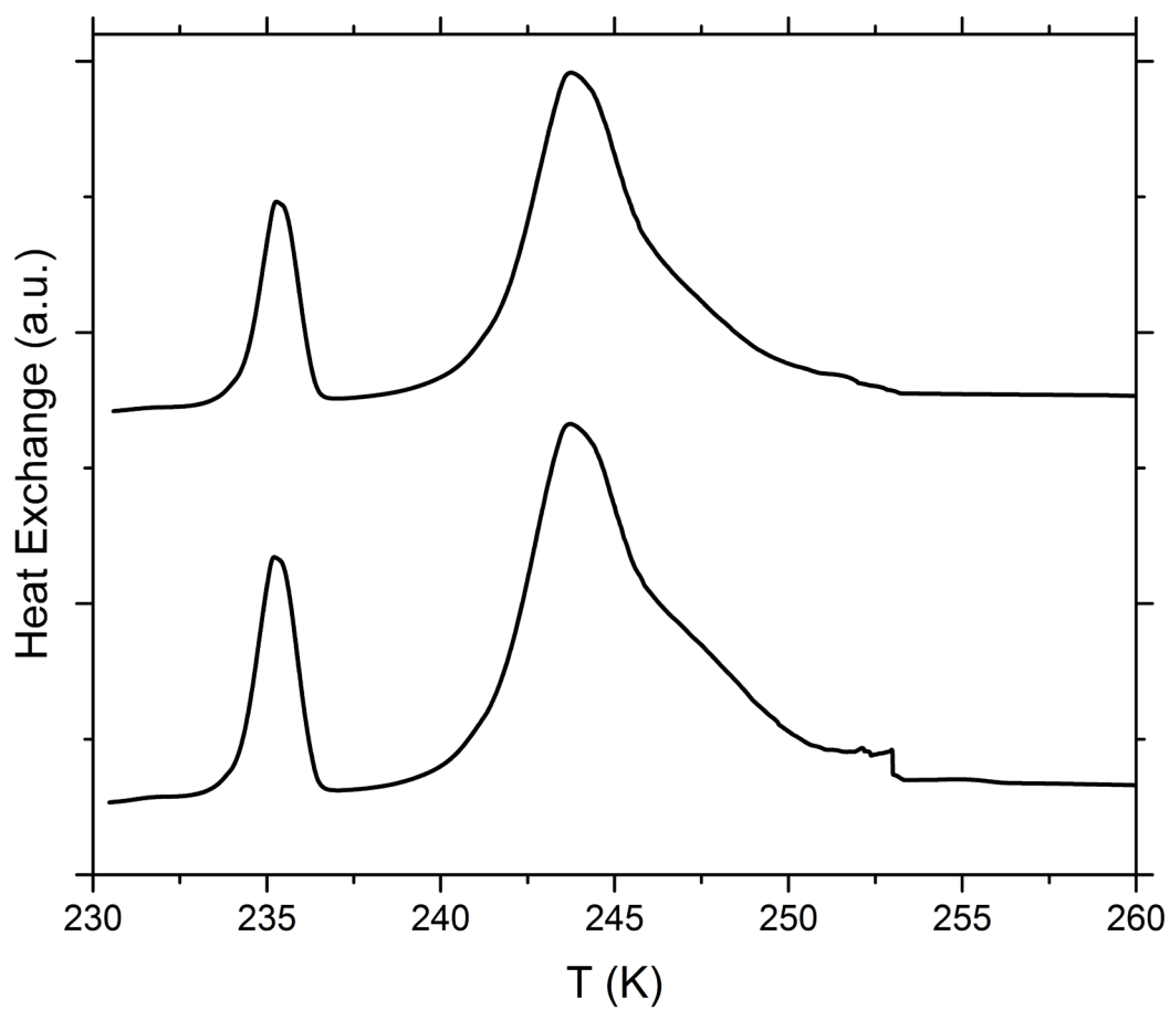
Figure S16. DSC thermograms of reversibility tests on separate suspensions with 5 wt% SA quartz particles aged for 5 days in 5 wt% sodium sulfate solution. Aged particles were collected after aging and resuspended in pure water. All curves are normalized such that the areas under the heterogeneous and homogeneous freezing curves sum up to the same value.
