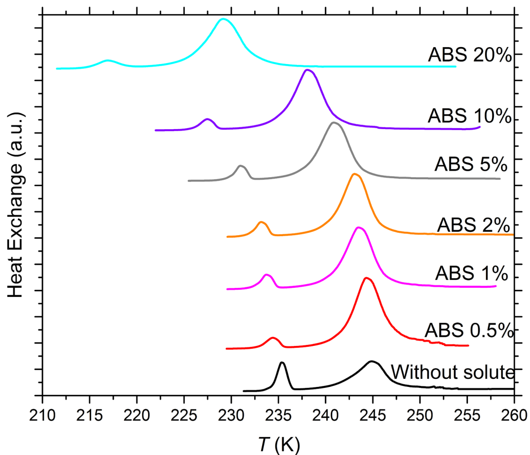
Figure S1. DSC thermograms of 5 wt% of SA quartz particles suspended in ammonium bisulfate (ABS) solution droplets of varying concentration. All curves are normalized such that the areas under the heterogeneous and homogeneous freezing curves sum up to the same value. Numbers next to each curve: Solute concentration in wt%.
