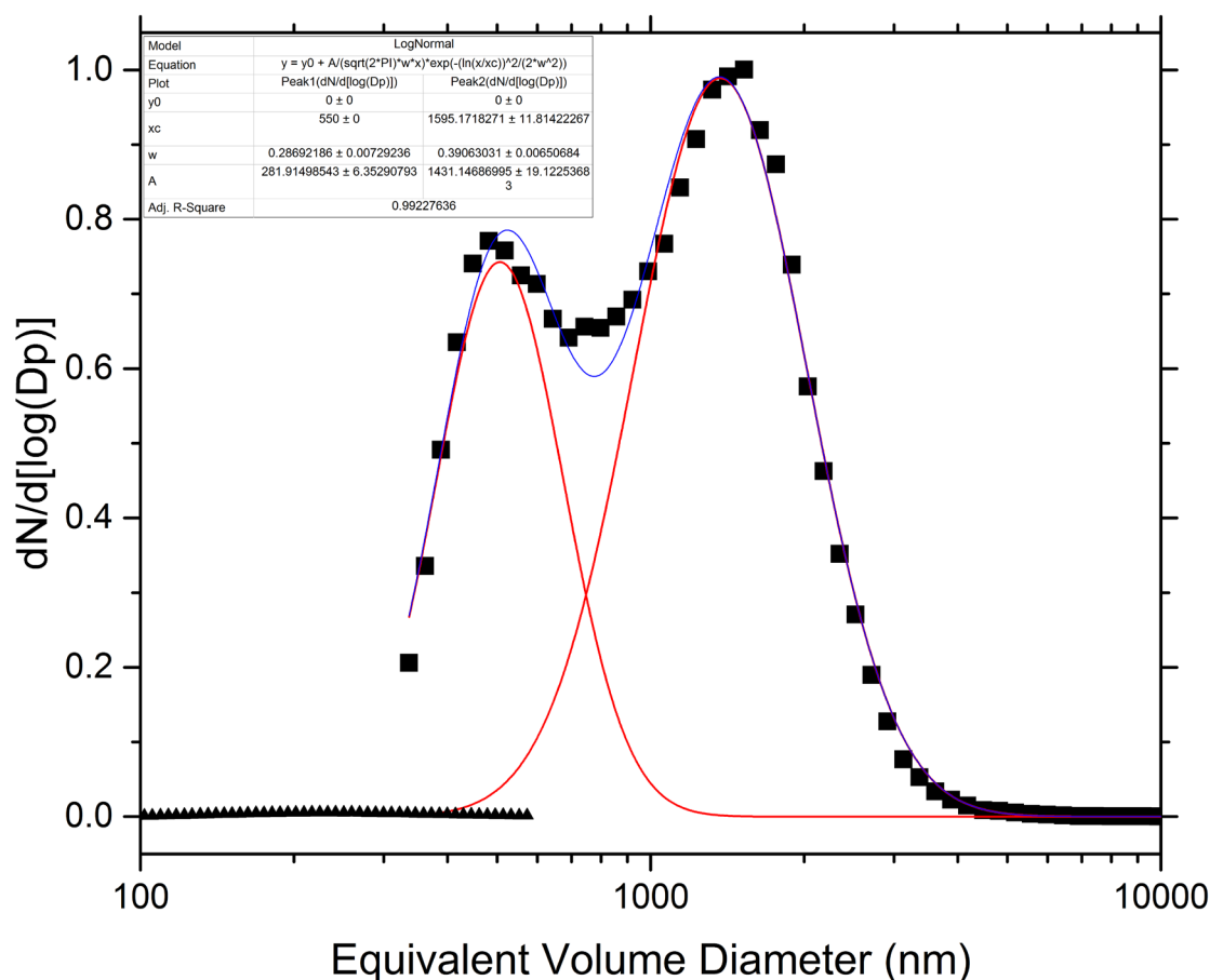
Figure S29. Particle size distribution of SA quartz sample. Solid black squares: APS; solid black triangles: SMPS; red lines: two lognormal fits to data obtained from APS and SMPS; blue line: resultant bimodal lognormal fit to the observed dataset.
