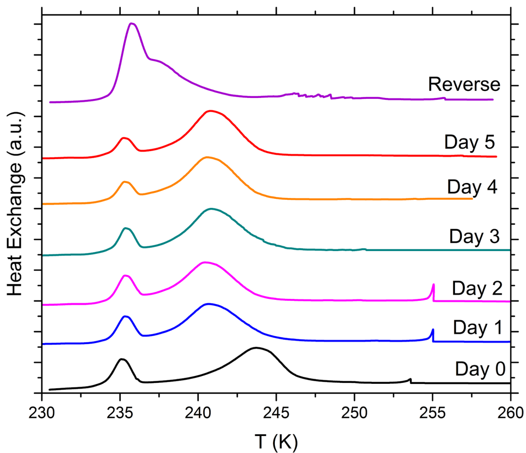
Figure S20. DSC thermograms of aging and reversibility tests on suspensions with 5 wt% SA quartz particles prepared in polypropylene tubes and aged for 5 days in ammonia solution (0.005 molal). Aged particles were collected after aging and resuspended in pure water. All curves are normalized such that the areas under the heterogeneous and homogeneous freezing curves sum up to the same value.
