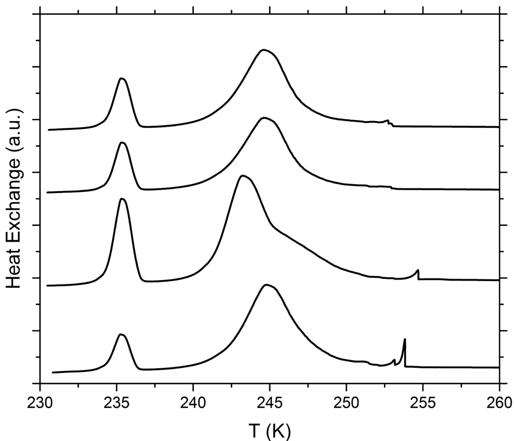
Figure S12. DSC thermograms of reversibility tests on four separate suspensions with 5 wt% SA quartz particles aged for 5 days in pure water. Aged particles were collected after aging and resuspended in pure water. All curves are normalized such that the areas under the heterogeneous and homogeneous freezing curves sum up to the same value.
