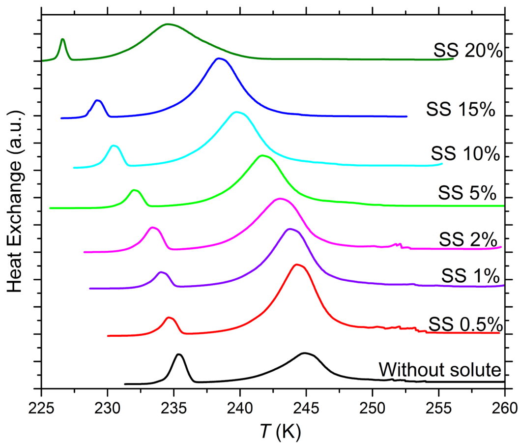
Figure S3. DSC thermograms of 5 wt% SA quartz particles suspended in sodium sulfate (SS) solution droplets of varying concentration. All curves are normalized such that the areas under the heterogeneous and homogeneous freezing curves sum up to the same value. Numbers next to each curve: Solute concentration in wt%.
