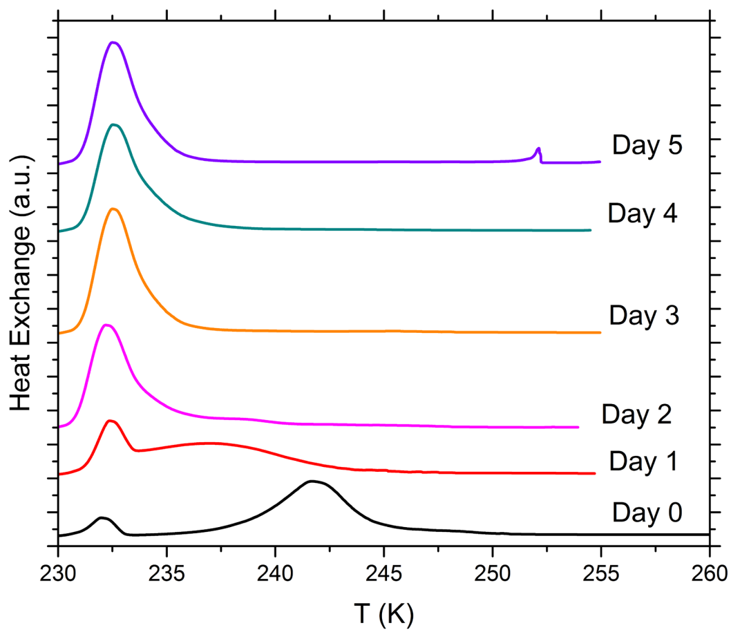
Figure S9. DSC thermograms of aging tests with 5 wt% SA quartz particles suspended in 5 wt% sodium sulfate solution droplets measured over a period of 5 days. All curves are normalized such that the areas under the heterogeneous and homogeneous freezing curves sum up to the same value.
