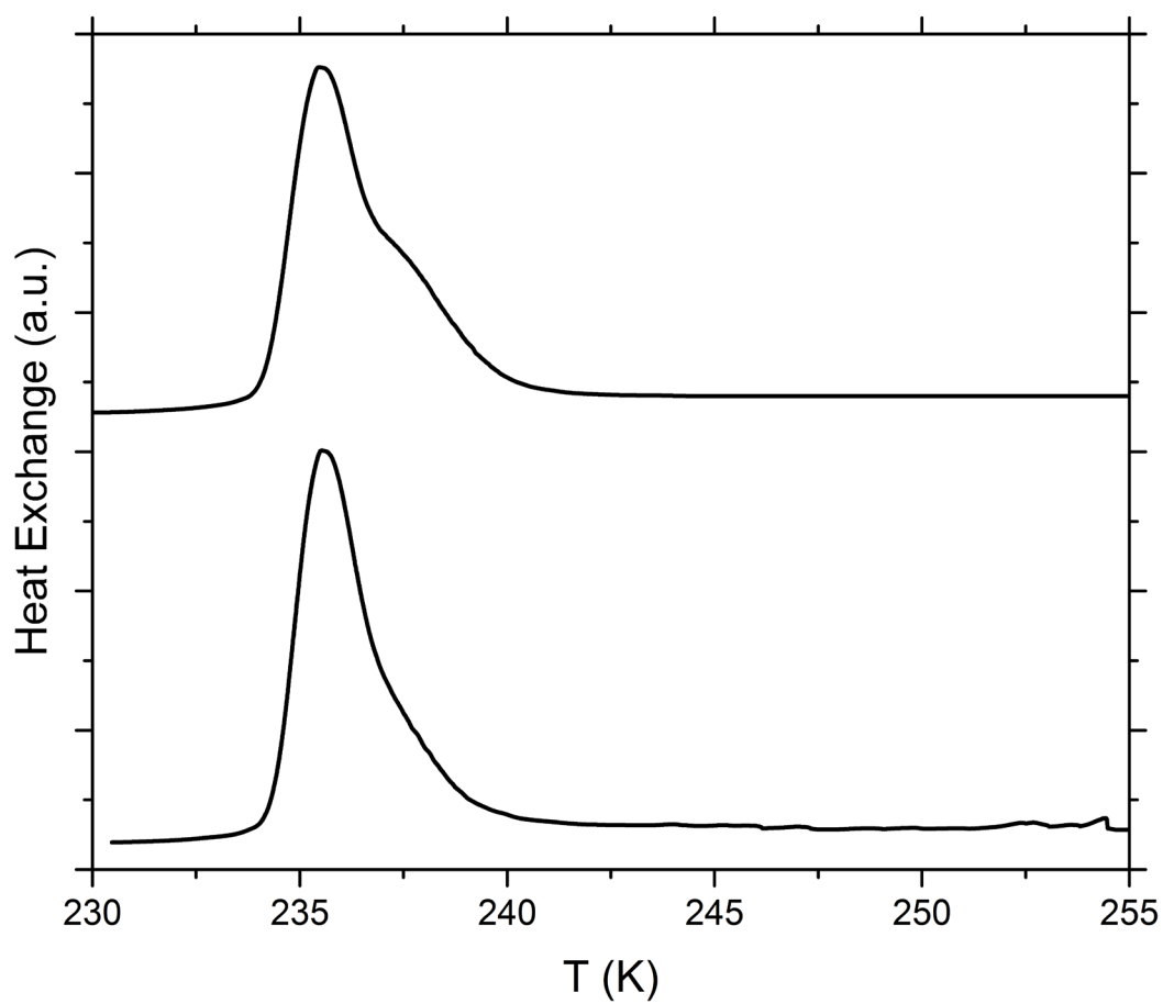
Figure S18. DSC thermograms of reversibility tests on separate suspensions with 5 wt% SA quartz particles aged for 5 days in 5 \times 10^{-3} molal sodium hydroxide solution. Aged particles were collected after aging and resuspended in pure water. All curves are normalized such that the areas under the heterogeneous and homogeneous freezing curves sum up to the same value.
