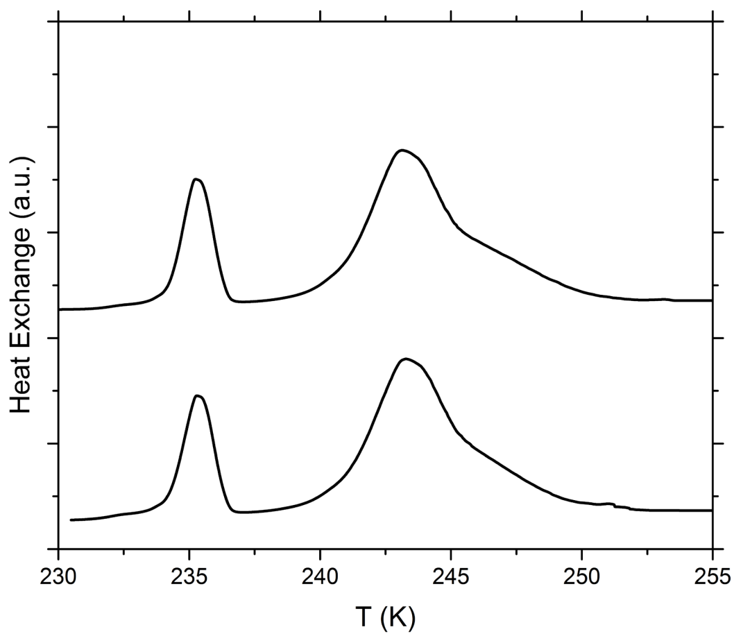
Figure S17. DSC thermograms of reversibility tests on separate suspensions with 5 wt% SA quartz particles aged for 5 days in 5 \times 10^{-6} molal sodium hydroxide solution. Aged particles were collected after aging and resuspended in pure water. All curves are normalized such that the areas under the heterogeneous and homogeneous freezing curves sum up to the same value.
