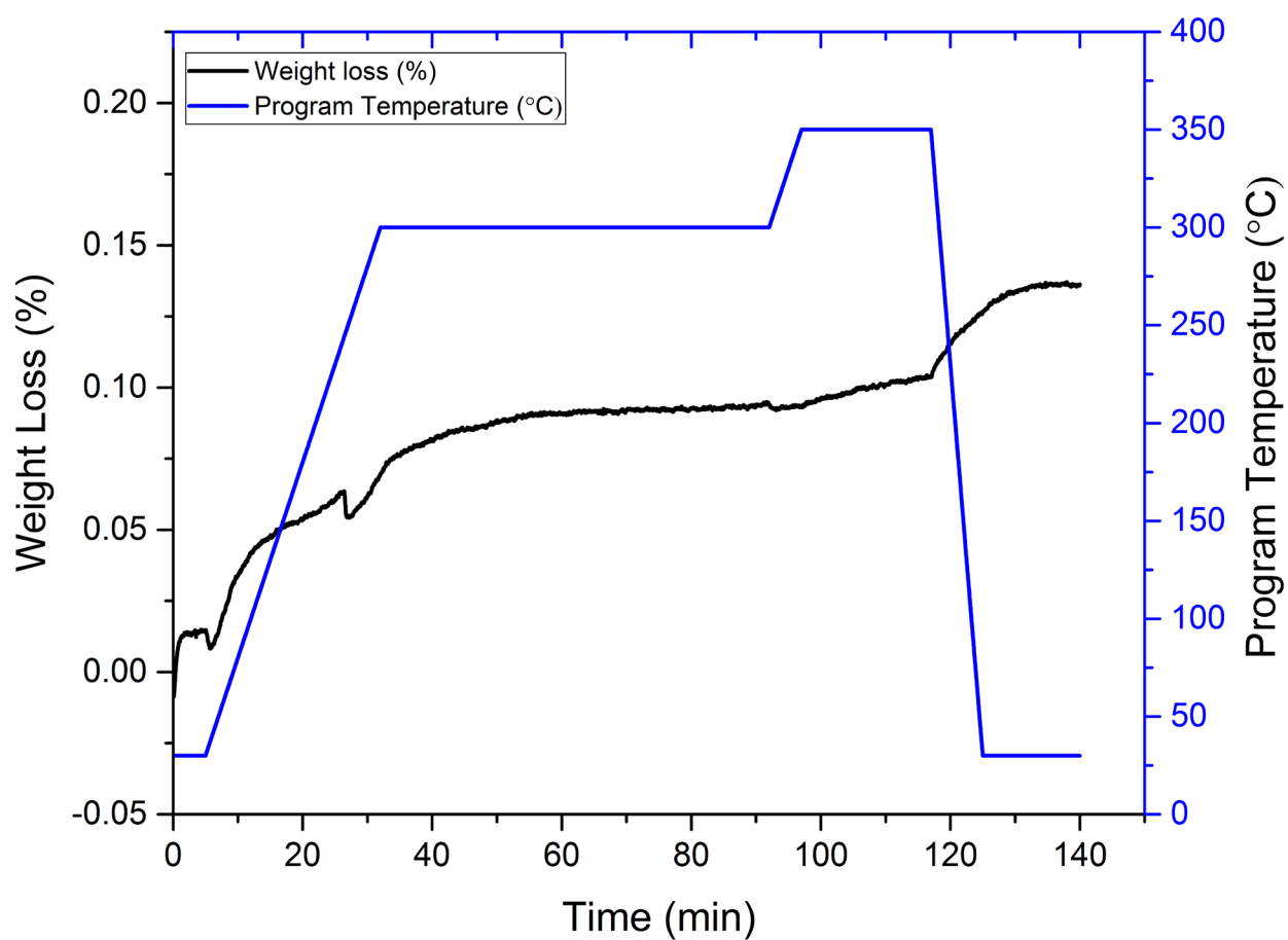
Figure S25. Mass loss of the Kaufmann quartz sample measured by thermogravimetric analysis. Blue line: temperature (°C); black line: sample weight loss (in %). A minor loss of up to 0.14% in weight was observed.
