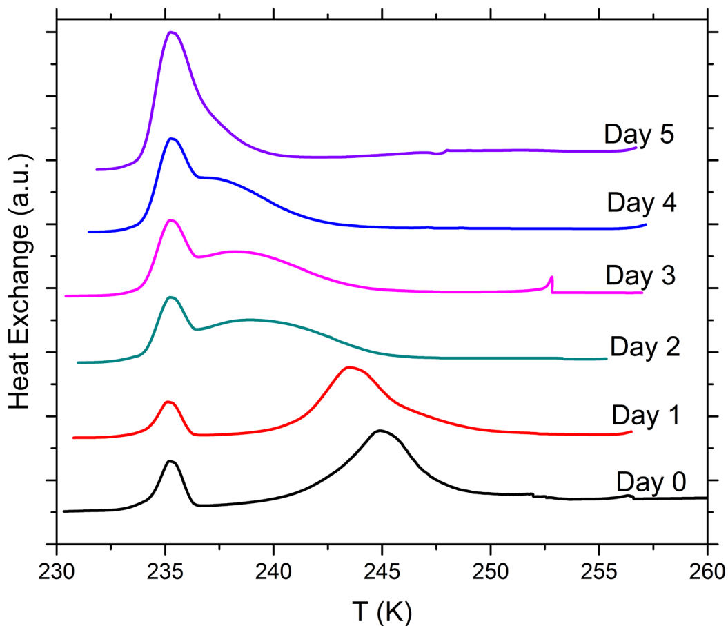
Figure S5. DSC thermograms of aging tests with 5 wt% SA quartz particles suspended in pure water droplets measured over a period of 5 days. All curves are normalized such that the areas under the heterogeneous and homogeneous freezing curves sum up to the same value.
