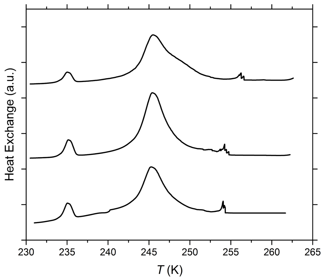
Figure S23. DSC thermograms of freezing experiments on separate suspensions with 5 wt% milled SA quartz particles in pure water. All curves are normalized such that the areas under the heterogeneous and homogeneous freezing curves sum up to the same value.
