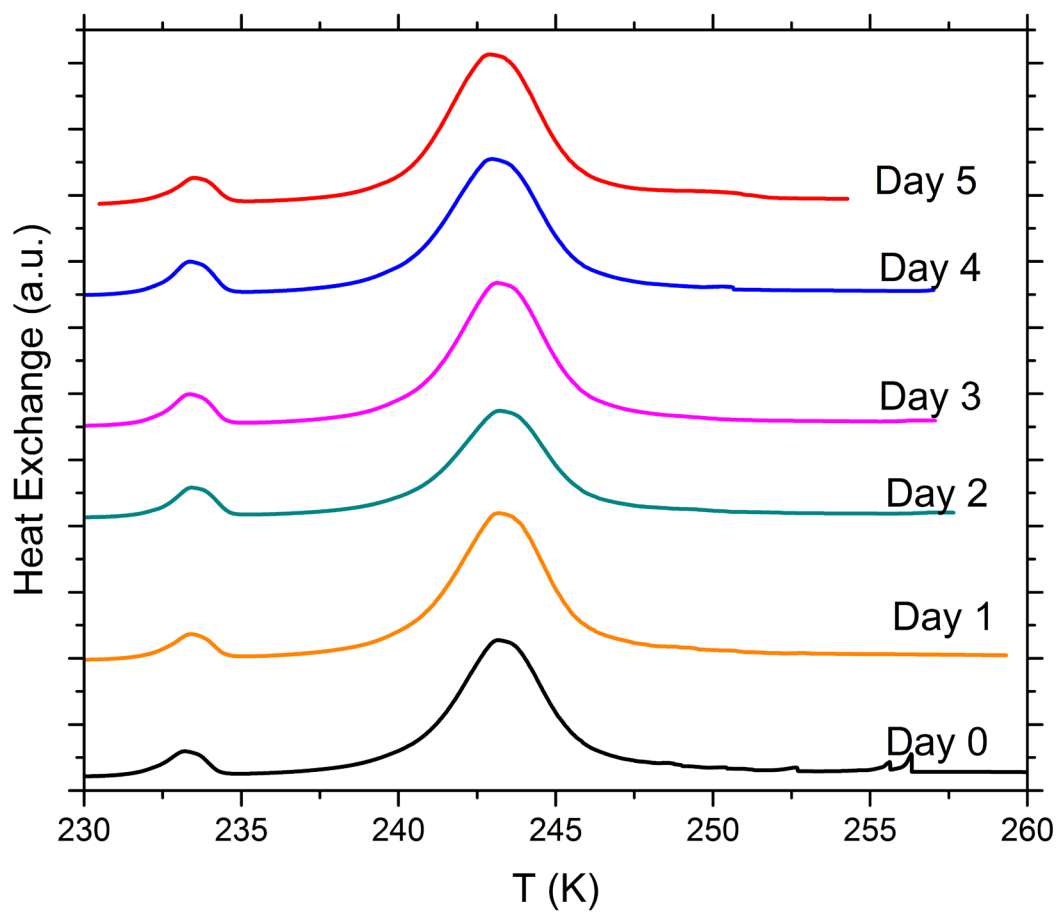
Figure S7. DSC thermograms of aging tests with 5 wt% SA quartz particles suspended in 2 wt% ammonium bisulfate solution droplets measured over a period of 5 days. All curves are normalized such that the areas under the heterogeneous and homogeneous freezing curves sum up to the same value.
