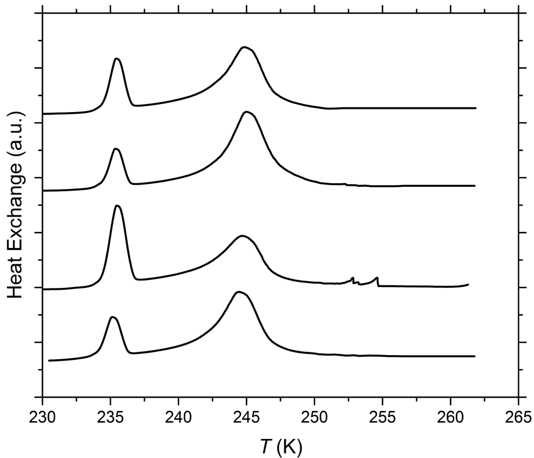
Figure S22. DSC thermograms of freezing experiments on separate suspensions with 1 wt% milled SA quartz particles in pure water. All curves are normalized such that the areas under the heterogeneous and homogeneous freezing curves sum up to the same value.
