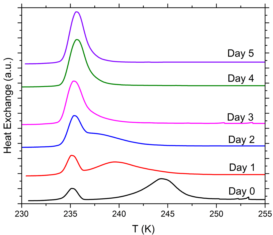
Figure S11. DSC thermograms of aging tests with 5 wt% SA quartz particles suspended in 5 \times 10^{-6} molal sodium hydroxide solution droplets measured over a period of 5 days. All curves are normalized such that the areas under the heterogeneous and homogeneous freezing curves sum up to the same value.
