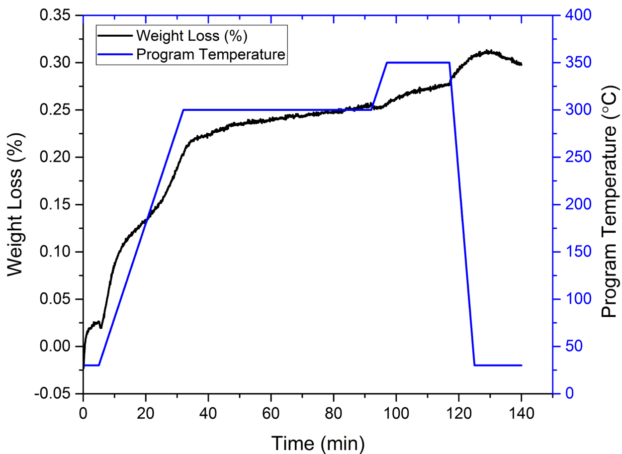
Figure S24. Mass loss of the SA quartz sample measured by thermogravimetric analysis. Blue line: temperature ( ^{\circ}\text{C} ); black line: sample weight loss (in %). A minor loss of up to 0.30% in weight was observed.
