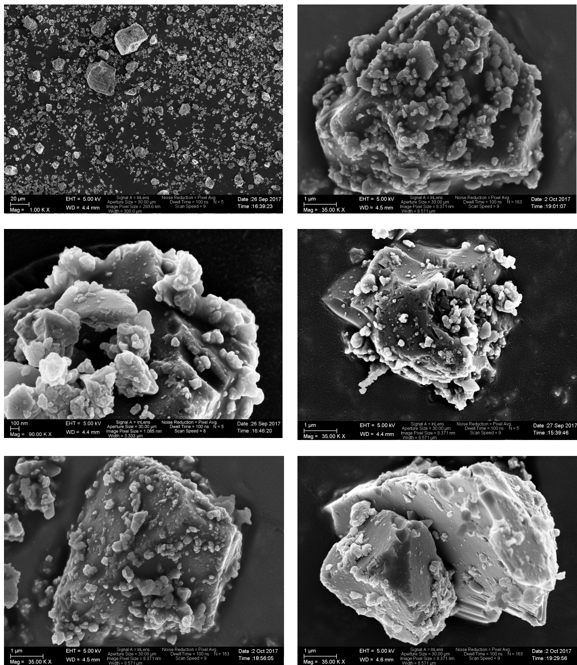
Figure S28. SEM images of Kaufmann quartz at various magnifications.
