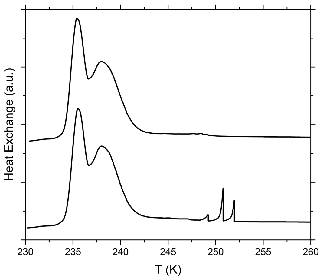
Figure S15. DSC thermograms of reversibility tests on separate suspensions with 5 wt% SA quartz particles aged for 5 days in 0.005 molal ammonia solution. Aged particles were collected after aging and resuspended in pure water. All curves are normalized such that the areas under the heterogeneous and homogeneous freezing curves sum up to the same value.
