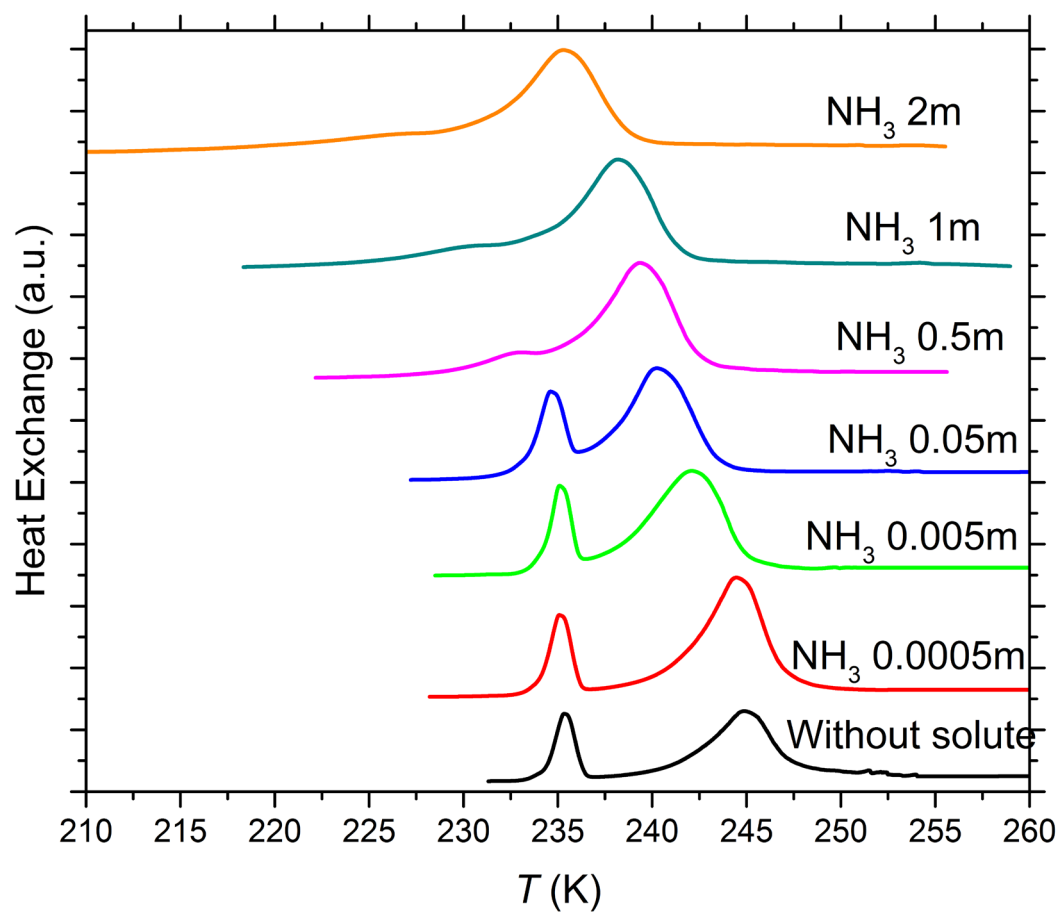
Figure S2. DSC thermograms of 5 wt% SA quartz particles suspended in ammonia ( \text{NH}_3 ) solution droplets of varying concentration. All curves are normalized such that the areas under the heterogeneous and homogeneous freezing curves sum up to the same value. Numbers next to each curve: Solute concentration in molality.
