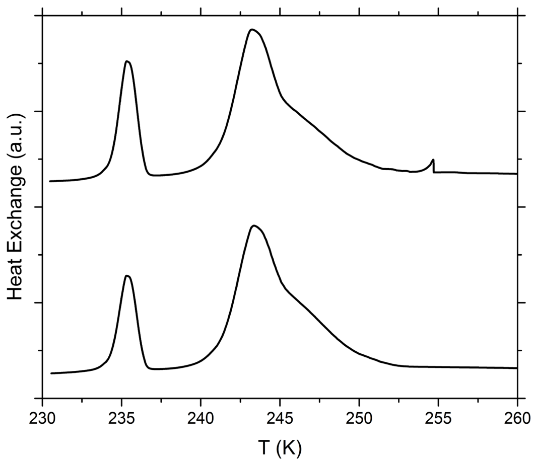
Figure S13. DSC thermograms of reversibility tests on separate suspensions with 5 wt% SA quartz particles aged for 5 days in 10 wt% ammonium sulfate solution. Aged particles were collected after aging and resuspended in pure water. All curves are normalized such that the areas under the heterogeneous and homogeneous freezing curves sum up to the same value.
