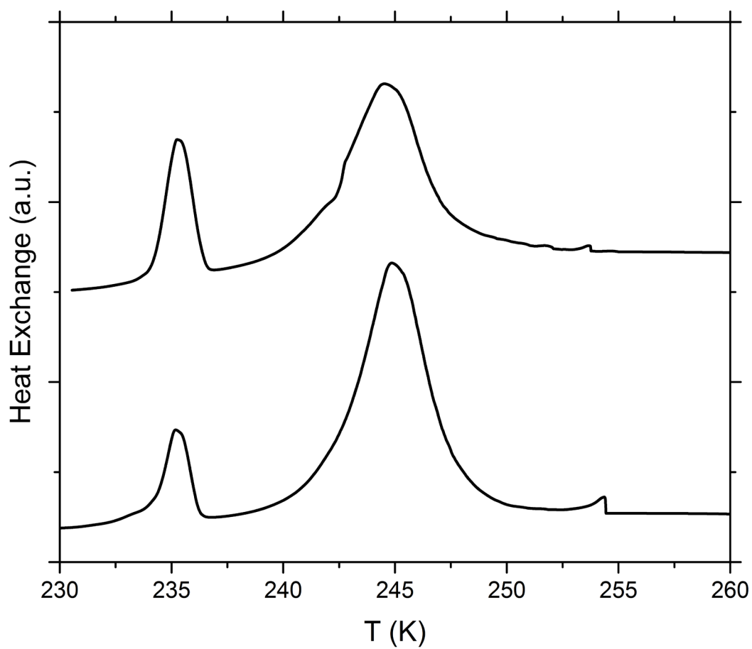
Figure S14. DSC thermograms of reversibility tests on separate suspensions with 5 wt% SA quartz particles aged for 5 days in 2 wt% ammonium bisulfate solution. Aged particles were collected after aging and resuspended in pure water. All curves are normalized such that the areas under the heterogeneous and homogeneous freezing curves sum up to the same value.
