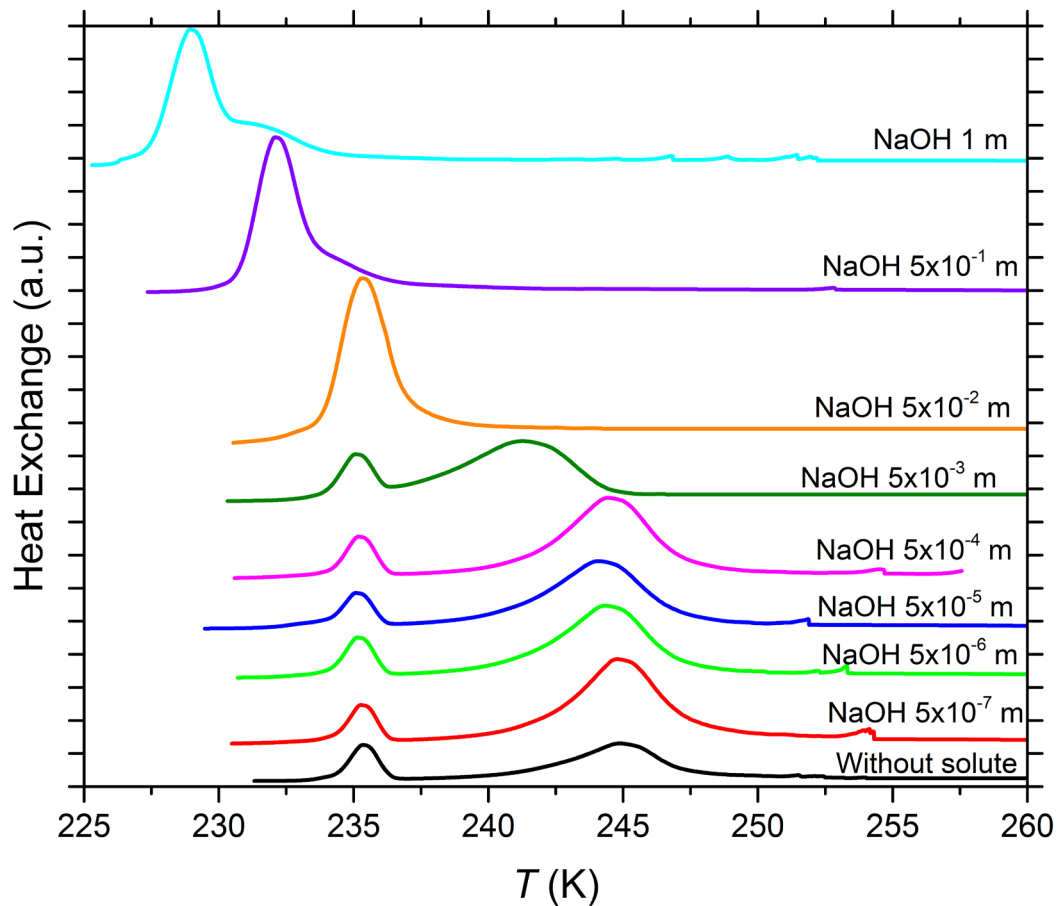
Figure S4. DSC thermograms of 5 wt% SA quartz particles suspended in sodium hydroxide (NaOH) solution droplets of varying concentration. All curves are normalized such that the areas under the heterogeneous and homogeneous freezing curves sum up to the same value. Numbers next to each curve: Solute concentration in molality.
