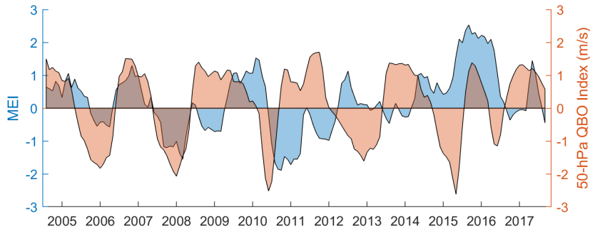
5 Figure 1. Bimonthly multivariate ENSO index (MEI, blue) and monthly 50-hPa QBO index ( u_{50} , m\ s^{-1} , orange) based on standardized anomaly of monthly zonal mean zonal wind at the Equator and 50-hPa both from NOAA at the period from August 2004 to September 2017. Positive MEI values indicate warm ENSO (El Niño) phases while negative MEI values indicate cold ENSO (La Niña) phases. Positive u_{50} values denote westerly QBO phases while negative u_{50} values denote easterly QBO phases.
