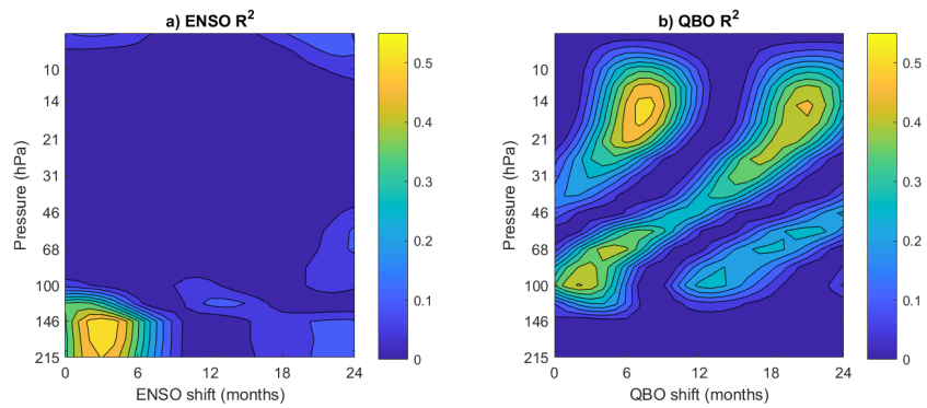
Figure 3. R-squared values for the linear regressions between the interannual tropical water vapor anomalies from MLS and the ENSO or QBO index at each pressure level with time lag shifts from 0-24 months. Figure 3a (left) is for ENSO ( WV = X_0 + X_1 \times \text{ENSO} ) and Fig. 3b (right) is for QBO ( WV = X_0 + X_1 \times \text{QBO} ). The time lag shift indicates the number of months that interannual tropical water vapor anomalies lag the ENSO or QBO index.
