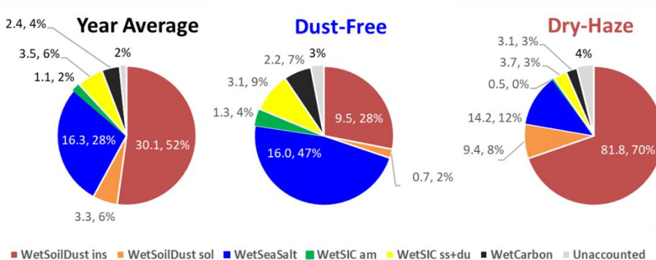
5 Figure 5: IMB obtained by attributing the calculated water content to the respective source classes, for the entire campaign and the Dust-Free and Dry-Haze seasons. Values are in \mu\text{g}\cdot\text{m}^{-3} and percentage of measured total mass.
