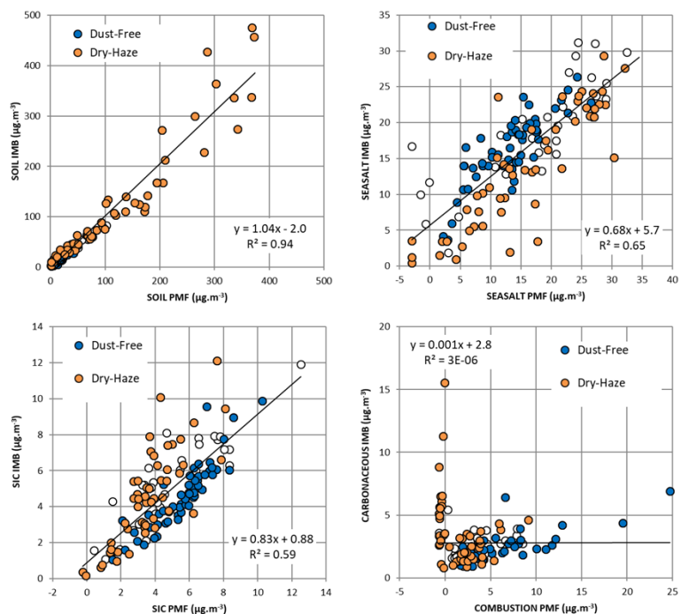
5 Figure 7: Comparison between the apportionment of individual samples using IMB and PMF, for four source classes. Circles filled in white represent periods with intermittent dust intrusions. Linear best fits are presented for the total sampling campaign.
