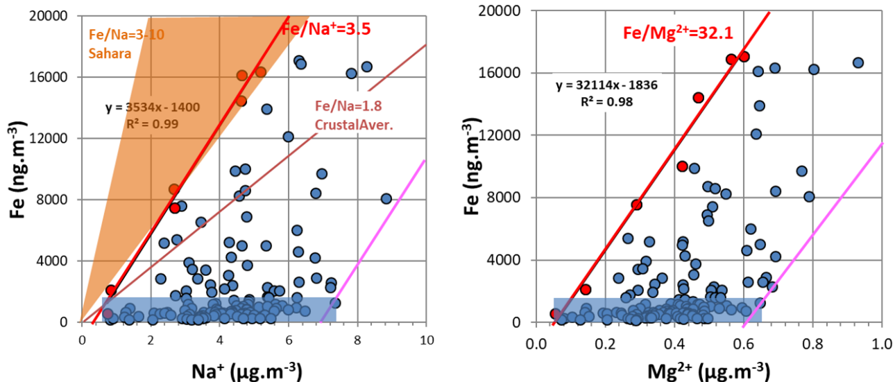
Figure 2: Edge lines (in red) for Fe versus \text{Na}^+ and Fe versus \text{Mg}^{2+} inter-comparisons. The blue rectangle represents periods without significant dust intrusions. The pink lines are parallels to the red edge lines in the maximum ion concentration regions. Also shown Fe/Na ratio ranges in Sahara and global soils, for total sodium, taken from Moreno et al., (2006), and Manson and Moore, (1982). Edge lines are best-fit linear lines traced through points in red.
