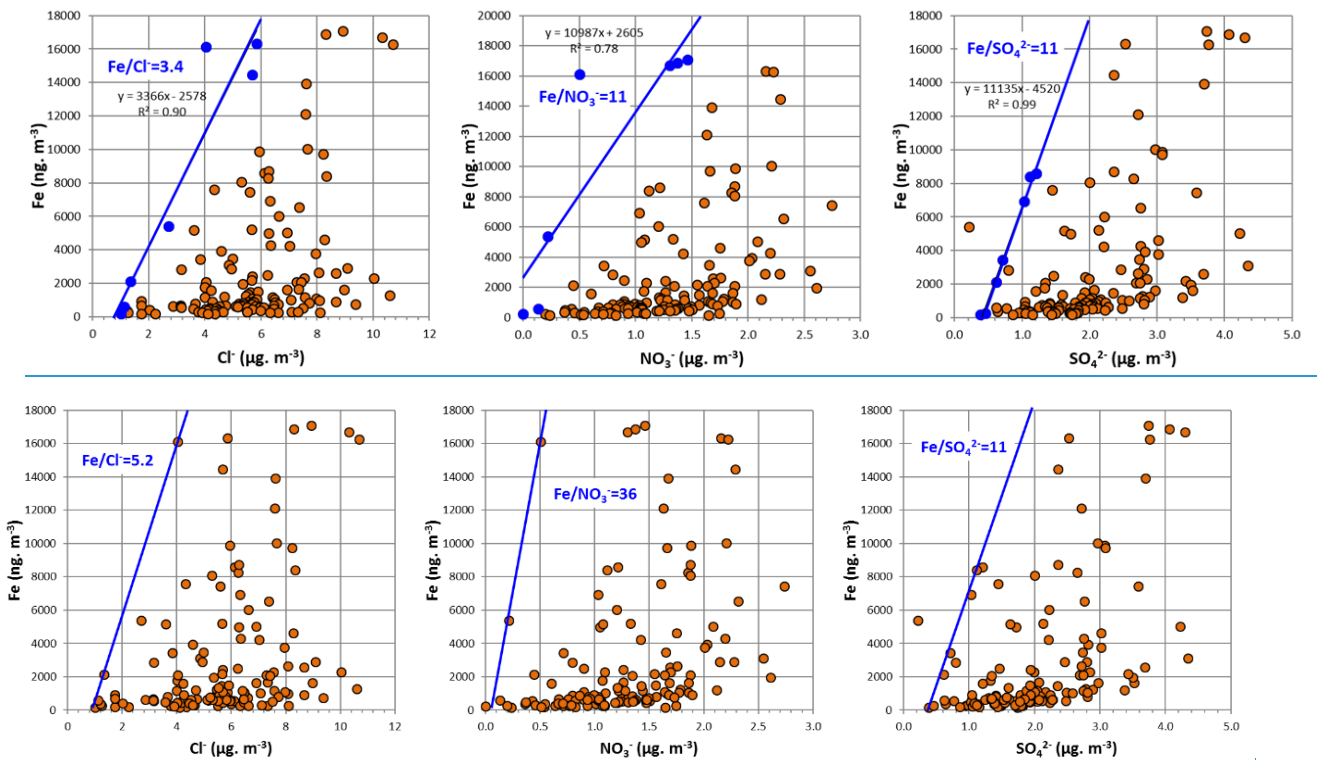
Figure A4: Relation between Fe and PM 10 concentrations. The blue line is the low edge representing, approximately, the amount of dust in PM 10 . Edge lines are best-fit linear lines traced through points in blue.
