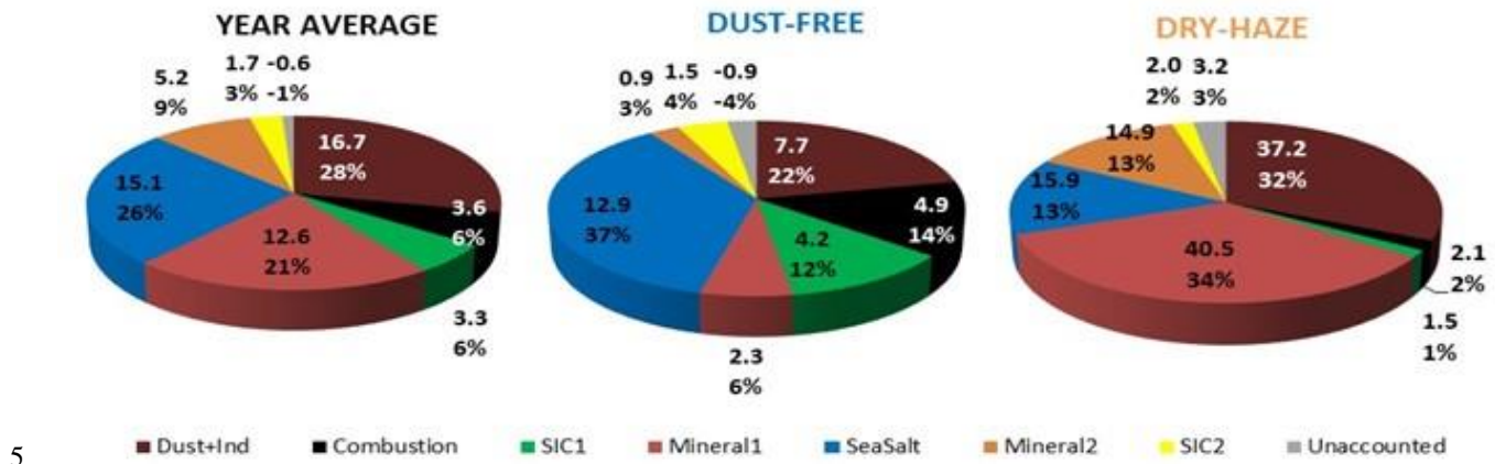
Figure 6: PMF source apportionment results, for the total campaign and during the two pollution seasons. Values are in µg.m -3 and percentage of measured total mass.
