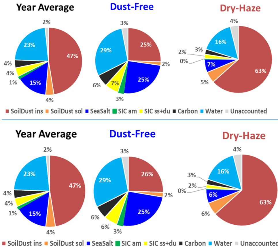
Figure 4: Inclusion of estimated water in the IMB, for the total sampling campaign and for the Dust-Free and Dry-Haze seasons.
