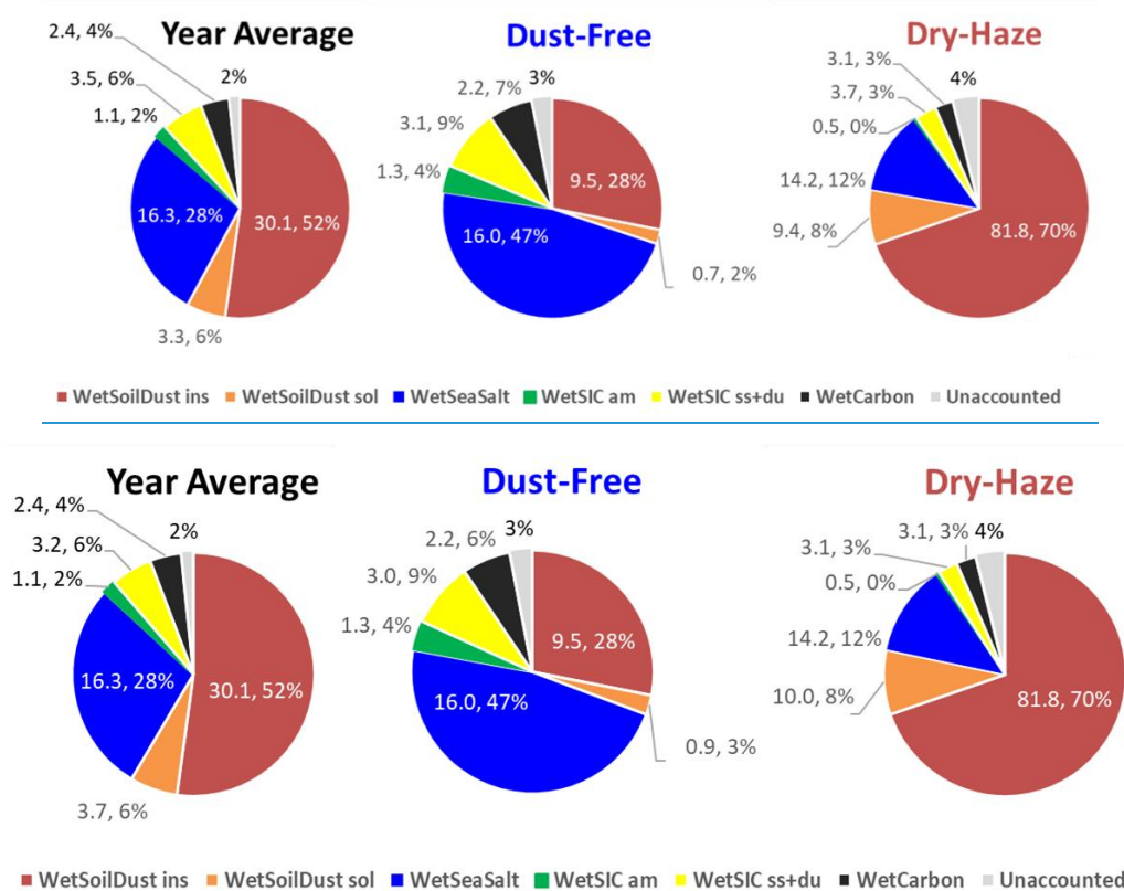
Figure 5: IMB obtained by attributing the calculated water content to the respective source classes, for the entire campaign and the Dust-Free and Dry-Haze seasons. Values are in \mu\text{g.m}^{-3} and percentage of measured total mass.
