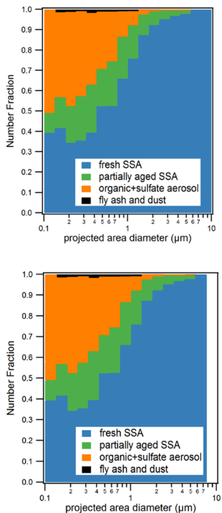
Figure 2: Size-resolved CCSEM-EDX number fraction distributions of observed particle types for all samples. Particles were sorted into 16 bins (logarithmic) from 0.1 to 10.0 μm projected area diameter (8 bins per decade).
