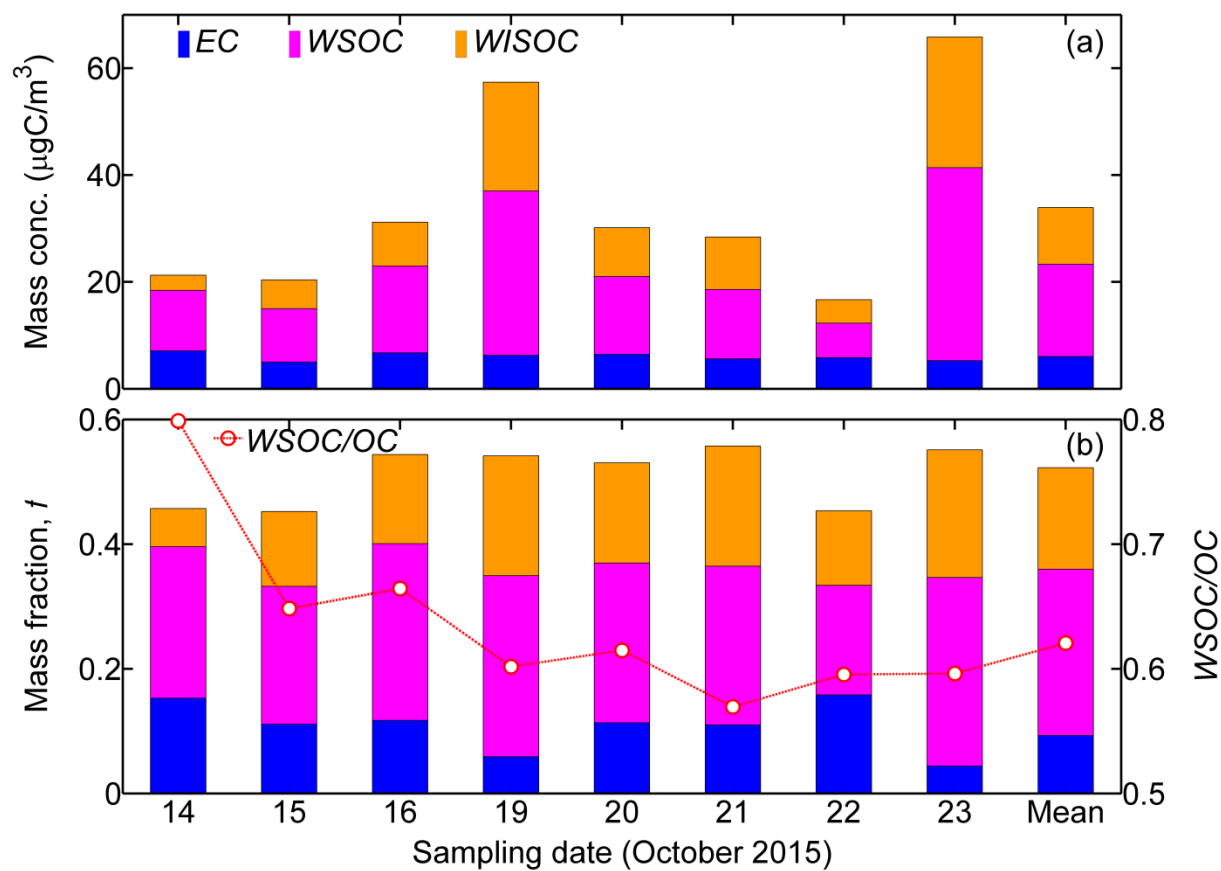
Fig. 4 (a) Mass concentration (Mass conc., \mu\text{gC}/\text{m}^3 ) and (b) corresponding mass fraction, f , of the carbon contents including EC , WSOC , and water-insoluble OC ( WISOC ) in PM_{2.5} filter samples. The WSOC/OC ratio is also displayed by the scattered dots in panel (b). All the corresponding temporal mean results are shown as “Mean”.
