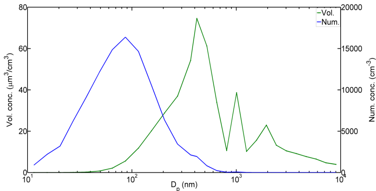
Fig. S2 Mean particle number (Num.) and volume (Vol.) size distributions over the entire wildfire haze observation period. Submicron particles with 200 \text{ nm} < D_p < 1 \text{ }\mu\text{m} dominate the particle volume concentration, while 30–200 nm particles are the major contributor to the particle number concentration.
