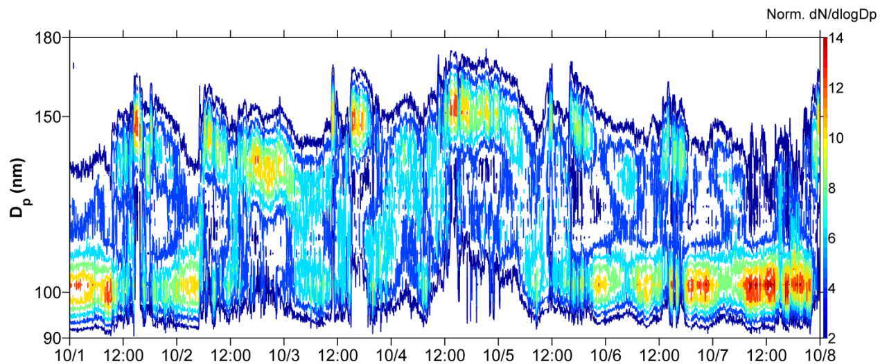
Fig. S3 An example (1–7 Oct 2015) of the HTDMA data at RH = 85% for D_0 = 100 nm particles. Temporal variation of normalized particle number size distributions (i.e., Norm. dN/dlog D_p ) is shown, with every 12 hours interval.
