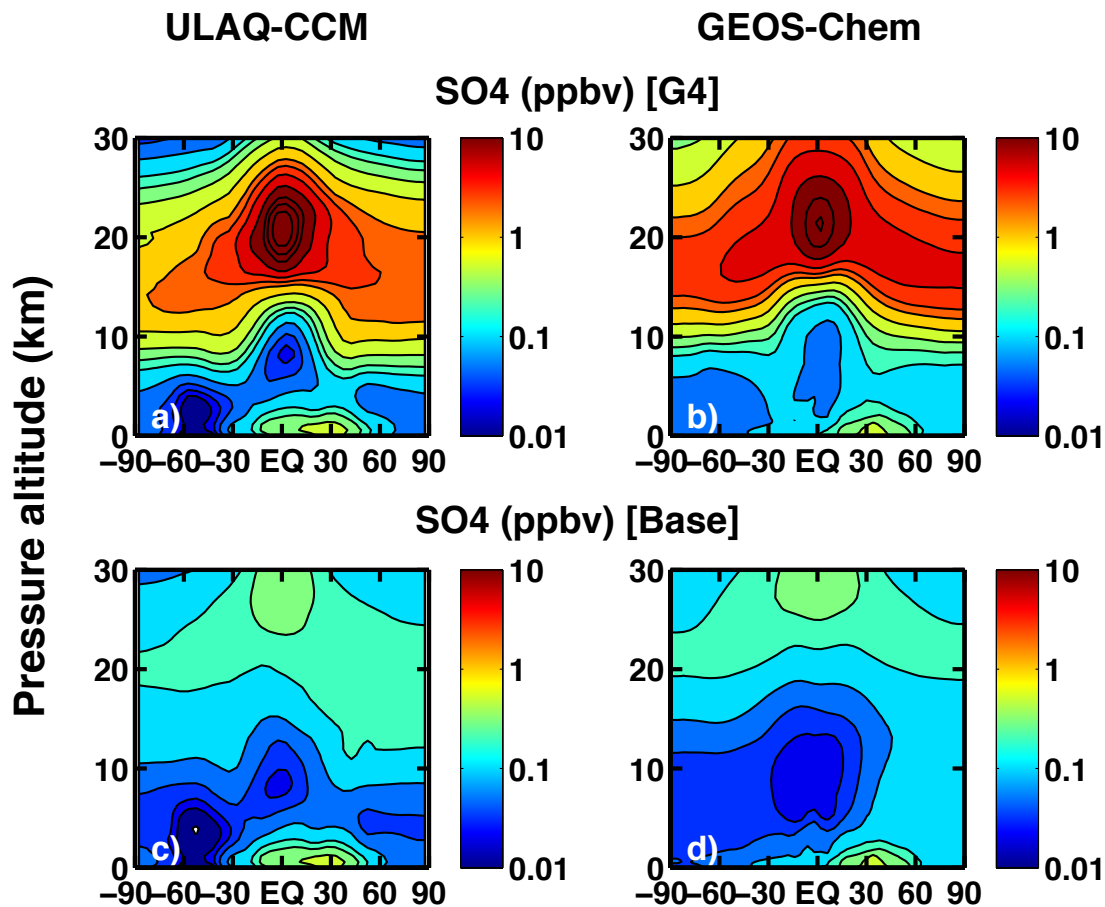
Figure 1. \text{SO}_4 mixing ratios (ppbv) averaged from 2030 to 2039 for ULAQ-CCM (panels a,c) and from 2000 to 2005 for GEOS-Chem (panels b,d). Panels (a,b) are for the G4 experiment; panels (c,d) are for the Base experiment. The contour line increment is logarithmic, with three lines per decade.
