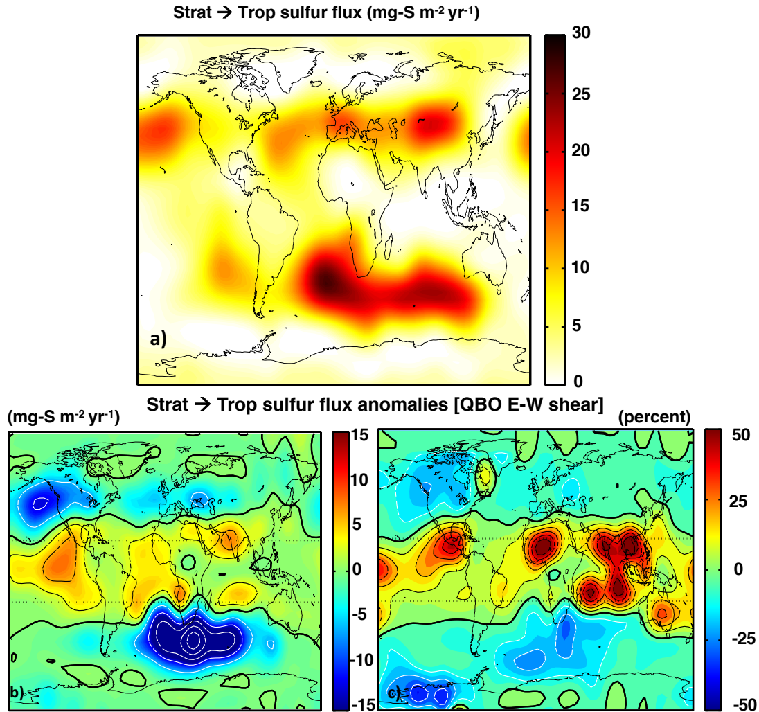
Figure 13. Panel (a): downward cross-tropopause sulfur flux changes (G4-Base) in ULAQ-CCM, as a function of latitude and longitude and averaged over years 2030-2039 ( \text{mg-S m}^{-2} \text{ yr}^{-1} ). Panels (b,c): as in (a), but showing differences between years with QBO easterly shear and years with QBO westerly shear; panel (b) shows the difference in absolute units ( \text{mg-S m}^{-2} \text{ yr}^{-1} ), whereas panel (c) shows the difference in percent of the decadal averaged flux changes presented in panel (a). Positive and negative anomalies are separated by the thick black curve (zero contour line); thin black/white curves show positive/negative contours with step of 5 \text{ mg-S m}^{-2} \text{ yr}^{-1} in panel (b) and 10\% in panel (c); dotted lines highlight the subtropical barriers at 25\text{N} and 25\text{S} . Integrated S-flux anomalies (QBO E-W shear) are as follows; tropics: +0.61 \text{ Tg-S/yr} ( +42\% ); NH: -0.51 \text{ Tg-S/yr} ( -31\% ); SH: -0.35 \text{ Tg-S/yr} ( -39\% ); global: -0.25 \text{ Tg-S/yr} ( -6\% )
