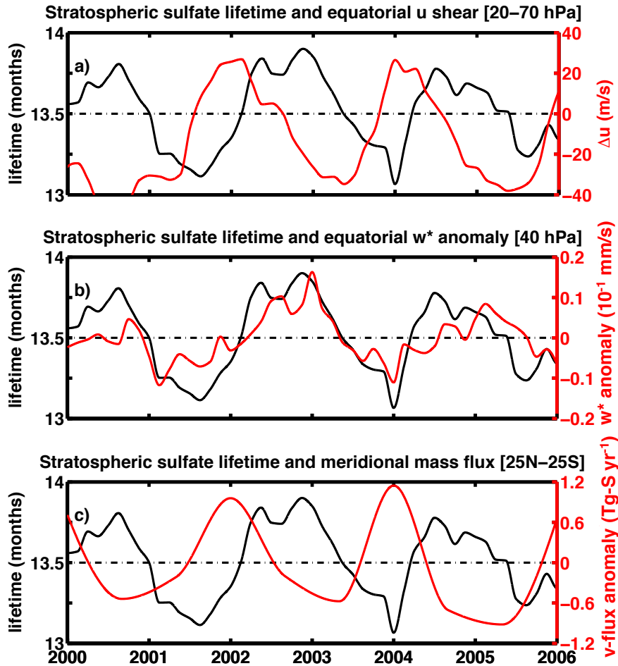
Figure 6. As in Fig. 5, but for GEOS-Chem for years 2000-2005. The calculated average lifetime of stratospheric sulfate from geoengineering sulfur injection of 8 \text{ Tg-SO}_2/\text{yr} is 13.5 \pm 0.3 months in GEOS-Chem (equatorial residual vertical velocity w^* = 0.14 \pm 0.06 \text{ mm/s} , as a time average between 20 and 70 hPa; net poleward meridional sulfate flux out the tropical pipe \Phi_V = 2.31 \pm 0.38 \text{ Tg-S/yr} , as a time average at 25S and 25N latitude above the tropopause). The monthly variability of the sulfate lifetime (0.3 months) is smaller than in ULAQ-CCM (1.2 months), but closer to the latter when the ULAQ model is operated in CTM mode (0.6 months), i.e., using the Base circulation for the G4 case, without including the aerosol radiative feedback on dynamics (see text).
