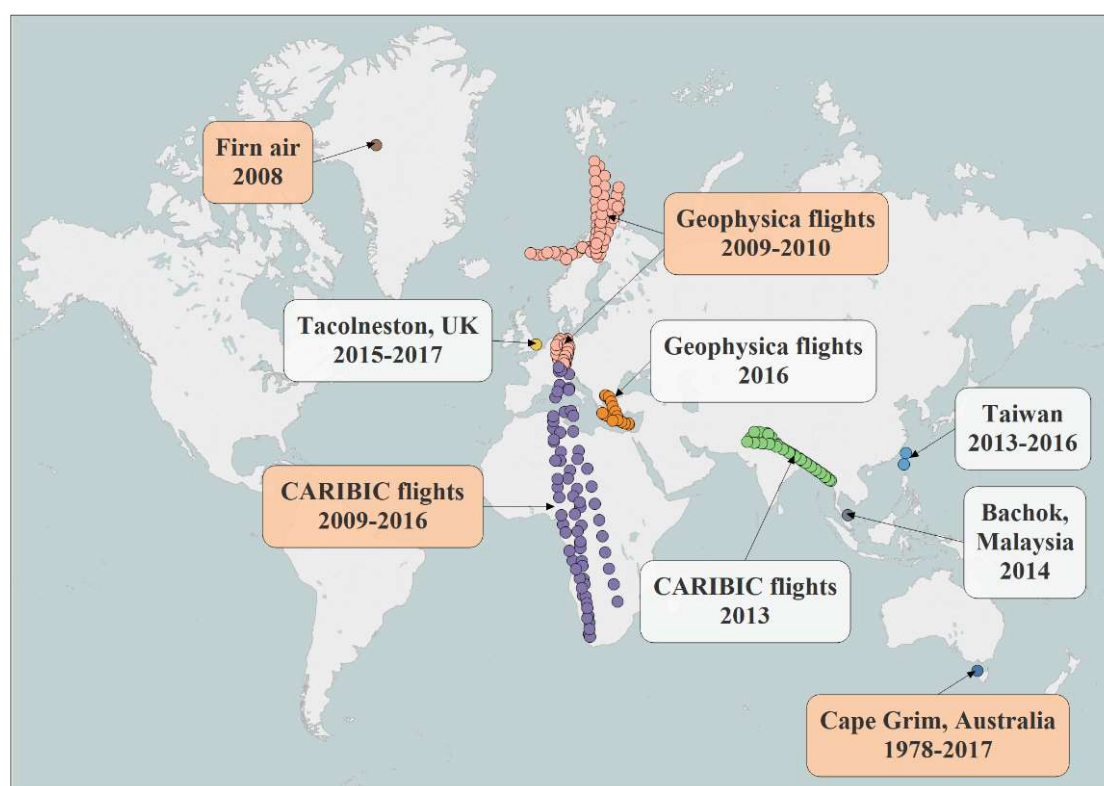
Figure 1. Sampling locations used in this study. Those locations that have been added since Laube et al. (2014) are in white. Those shaded orange featured in, or have been extended since, the Laube et al. paper.
