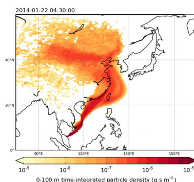
Figure 9. NAME footprint derived from 12-day backward simulation and showing the time integrated density of particles below 100 m altitude on 22-Jan-2014 during a period of elevated CFC-113a mixing ratios at Bachok, Malaysia.
