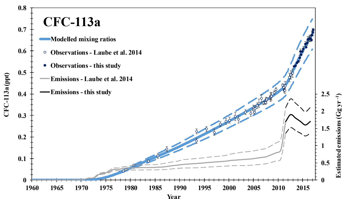
Figure 3. CFC-113a modelled and observed mixing ratios at Cape Grim 1960-2017 and estimated global annual emissions of CFC-113a. The observations are from July 1978-February 2017 with 1\sigma standard deviations as error bars. Data prior to 04-Dec-2012 is from Laube et al. (2014). The blue solid line represents the modelled mixing ratios with uncertainties (dashed blue line). The dashed black and grey lines represent the modelled 'best fit'
