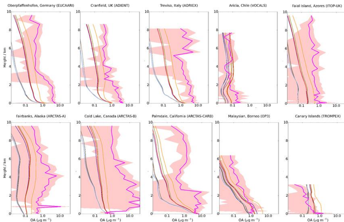
Figure 14 – Mean vertical profile of OA ( \mu\text{g m}^{-3} ) for 10 field campaigns (pink) with the mean UKCA for the simulations described in Table 2. The standard deviation of the binned observations at each model layer are shown (peach envelope).
