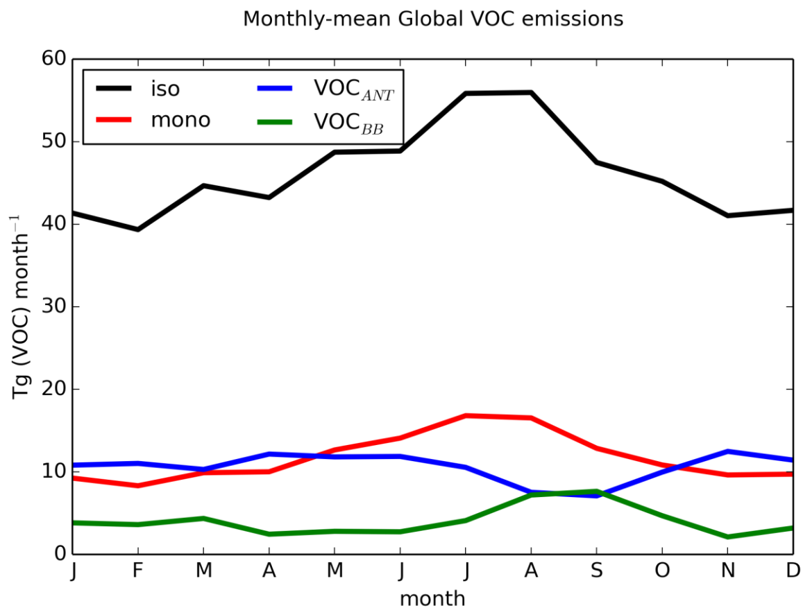
Figure 2 – Seasonality of global SOA precursor emissions from the different VOC sources: monoterpane (red), isoprene (black), VOC ANT (blue) and VOC BB (green) (Tg (VOC) month -1 ).
