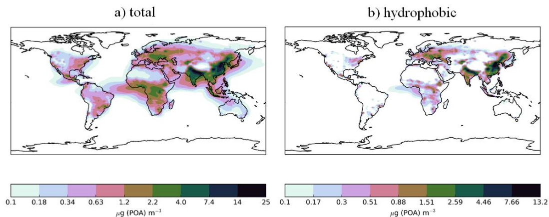
Figure 8 – Annual-average surface (a) total (hydrophilic and hydrophobic), and (b) hydrophobic only, POA concentrations ( \mu\text{g m}^{-3} ) for the Control simulation. Within UKCA, all POA is emitted into the hydrophobic modes and re-distributed into the hydrophilic modes through condensation-ageing.
