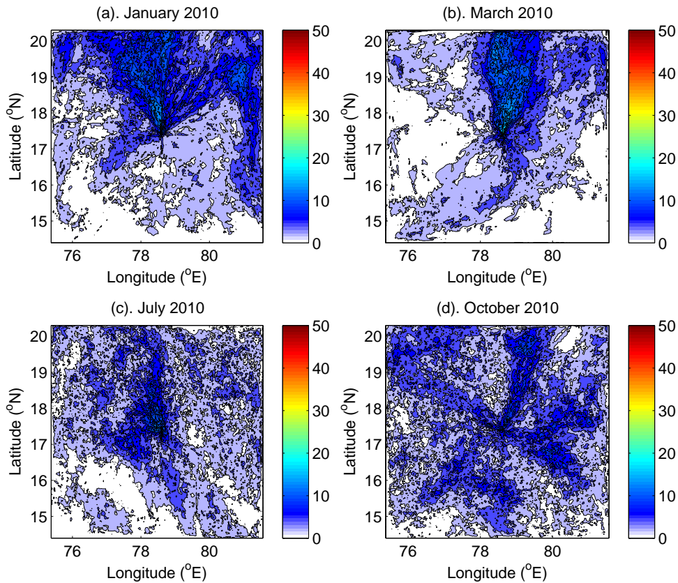
Figure 8. Spatial plot of probability (%) of epaturing-capturing capturing a peak in simulated BC within 4-5km 4-5 km for the model simulations carried out during a). January 2010, b). March 2010, c). July, 2010 and d). October 2010
