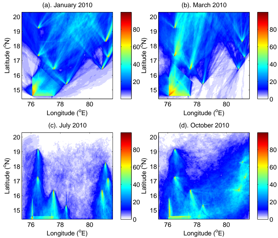
Figure 6. Spatial plot of probability (%) of capturing a peak in simulated BC within 9-11 km 9-11 km for the model simulations carried out during a). January 2010, b). March 2010, c). July, 2010 and d). October 2010
