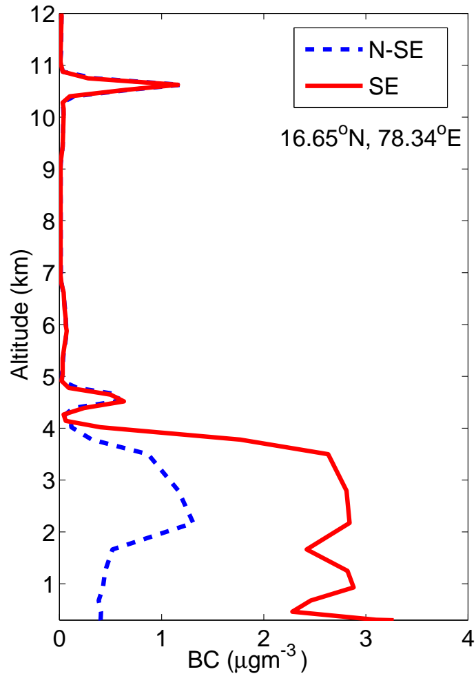
Figure 5. Model simulated vertical profile of BC during 17 th March 2010 for (a). N-SE runs (model simulations without prescription of surface level anthropogenic BC emissions) (b). SE runs (model simulations with prescription of surface level anthropogenic BC emissions).
