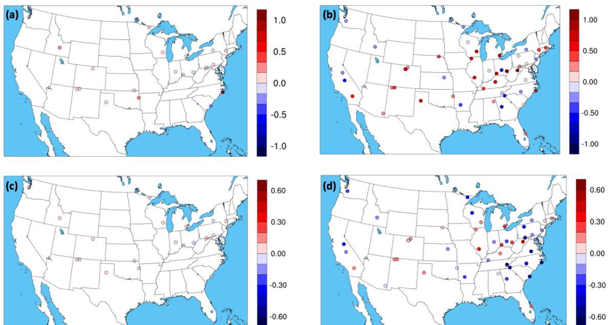
Figure S6. Difference of NH 3 Mean Fractional Error at AMoN sites between the base case, and (a) \gamma=10^{-3} for winter period, (b) \gamma=10^{-3} for summer period, (c) \gamma=10^{-4} for winter period, (d) \gamma=10^{-4} for summer period. Difference for \gamma=10^{-5} are not presented as they are very small. Red values indicate a deterioration of model performance and blue values indicate an improvement of model performance.
