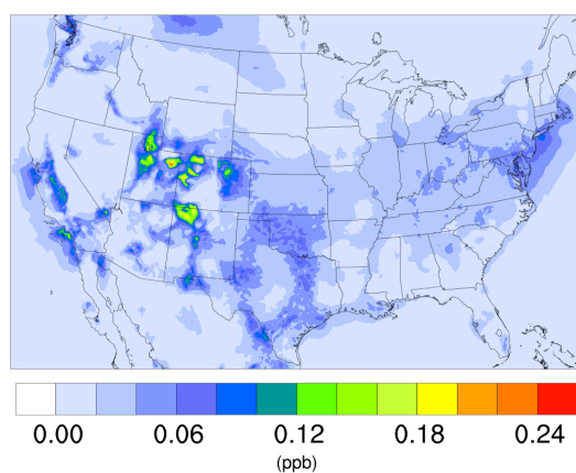
Figure S24. Spatial distribution of averaged N 2 O 5 concentration for winter period of the base case.
