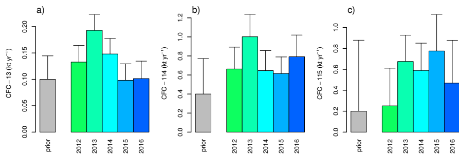
Figure 7. Total Chinese emissions of CFC-13 (a), \Sigma CFC-114 (b), and CFC-115 (c), estimated by the regional inversion. Uncertainties represent 1- \sigma range.
