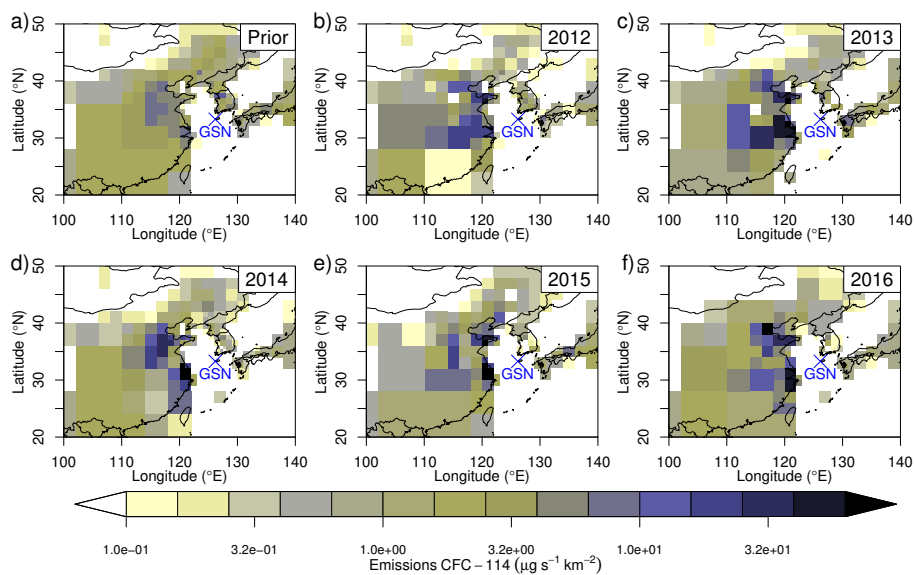
Figure 8. Emissions of \Sigma CFC-114 from north-eastern Asia as estimated by inverse modeling using the \Sigma CFC-114 observations at Gosan (marked with a blue cross). a) common prior distribution, b-f) posterior distribution for the years 2012 to 2016.
