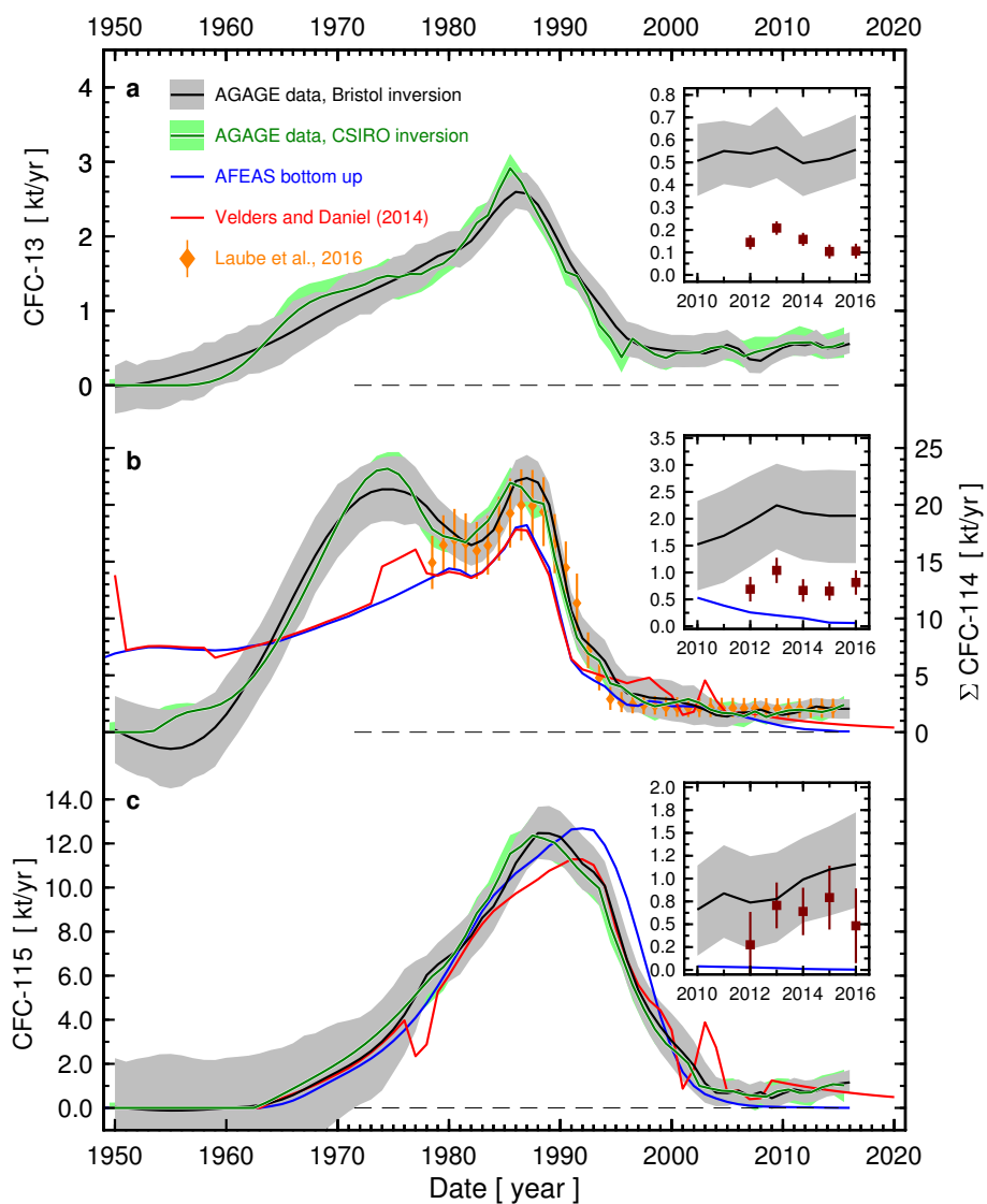
Figure 6. Global emissions of the chlorofluorocarbons CFC-13 (a), \Sigma CFC-114 (b), and CFC-115 (c) from atmospheric observations. Black lines and grey shaded areas are for the 'Bristol' inversion and green lines and green shaded areas for the 'CSIRO' inversion (see text). Emissions from Laube et al. (2016) are the sum of the emissions of both C_2Cl_2F_4 isomers. In the insets, our observation-based global emissions and the expanded AFEAS bottom-up emissions are compared to the East Asian emissions (maroon diamonds).
