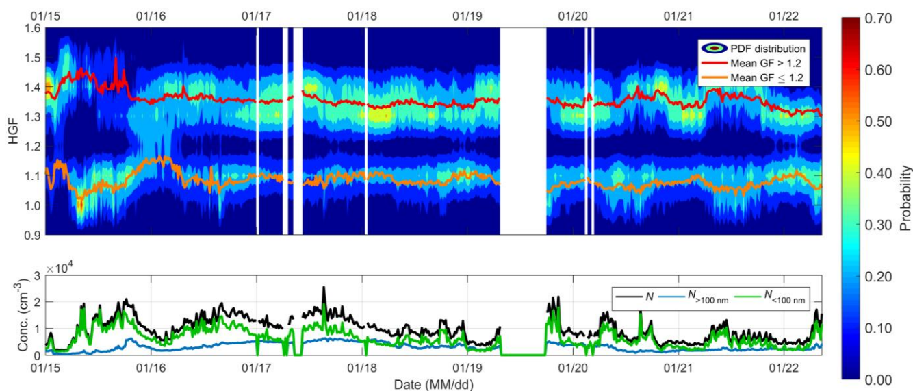
Figure 1. Temporal variability of the hygroscopic diameter growth factor probability density function (HGF-PDF) (upper panel) at RH=90% for particles with a dry diameter of 145 nm from 15 to 22 January 2015. The orange line displays the mean HGF of the nearly hydrophobic mode (HGF NH ), while the red line shows the mean HGF of the less hygroscopic mode (HGF LH ). Total particle number concentration ( N , black line), and concentrations of N_{<100} (green line) and N_{>100} (blue line) are also shown on the lower panel.
