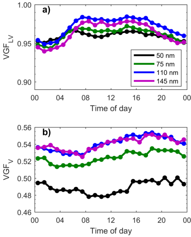
Figure 5. Mean diurnal variation of the volatility diameter growth factors for the less volatile mode (VGF LV ; panel a) and volatile mode (VGF V ; panel b) for different particle diameters. The panels have shared legends.
