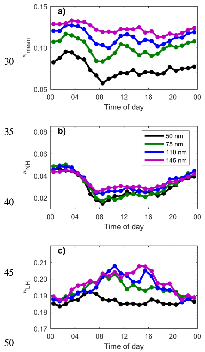
Figure 4. Mean diurnal variation of the hygroscopicity parameter \kappa for all data ( \kappa_{mean} ; panel a), separately for the nearly hydrophobic mode ( \kappa_{NH} ; panel b) and less hygroscopic mode ( \kappa_{LH} ; panel c) for different particle diameters. The panels have shared legends.
