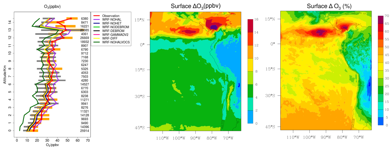
Figure 13. On the left, mean vertical profile of O_3 (ppbv) over the domain area using 13 flights from the TORERO campaign (red line) are compared to the 6-7 different WRF-Chem simulations: WRF-NOHAL (purple line), WRF-NOHET (blue line), WRF-NODEBROM (light green line), WRF-DEBROM (black line), WRF-GAMMADV2 (pink line), WRF-DIFF (yellow line) and WRF-NOHALVOCS (dark green line). Orange and grey horizontal bars indicate the 25th-75th quartile interval for the observations of the TORERO campaign and WRF-DEBROM simulation, respectively. Values are considered in 0.5 km bins and the numbers of aircraft measurement points for each altitude are given on the right side of each plot. On the middle and right, mean O_3 difference between the simulation with no halogen chemistry (WRF-NOHAL) and with halogen chemistry (WRF-DEBROM) for January and February 2012. Surface mean bias (ppbv) is shown in the left panel and surface relative mean bias (%) in the right panel. Relative mean bias (%) is calculated as (WRF-NOHAL - WRF-DEBROM)/WRF-NOHAL \times 100 .
