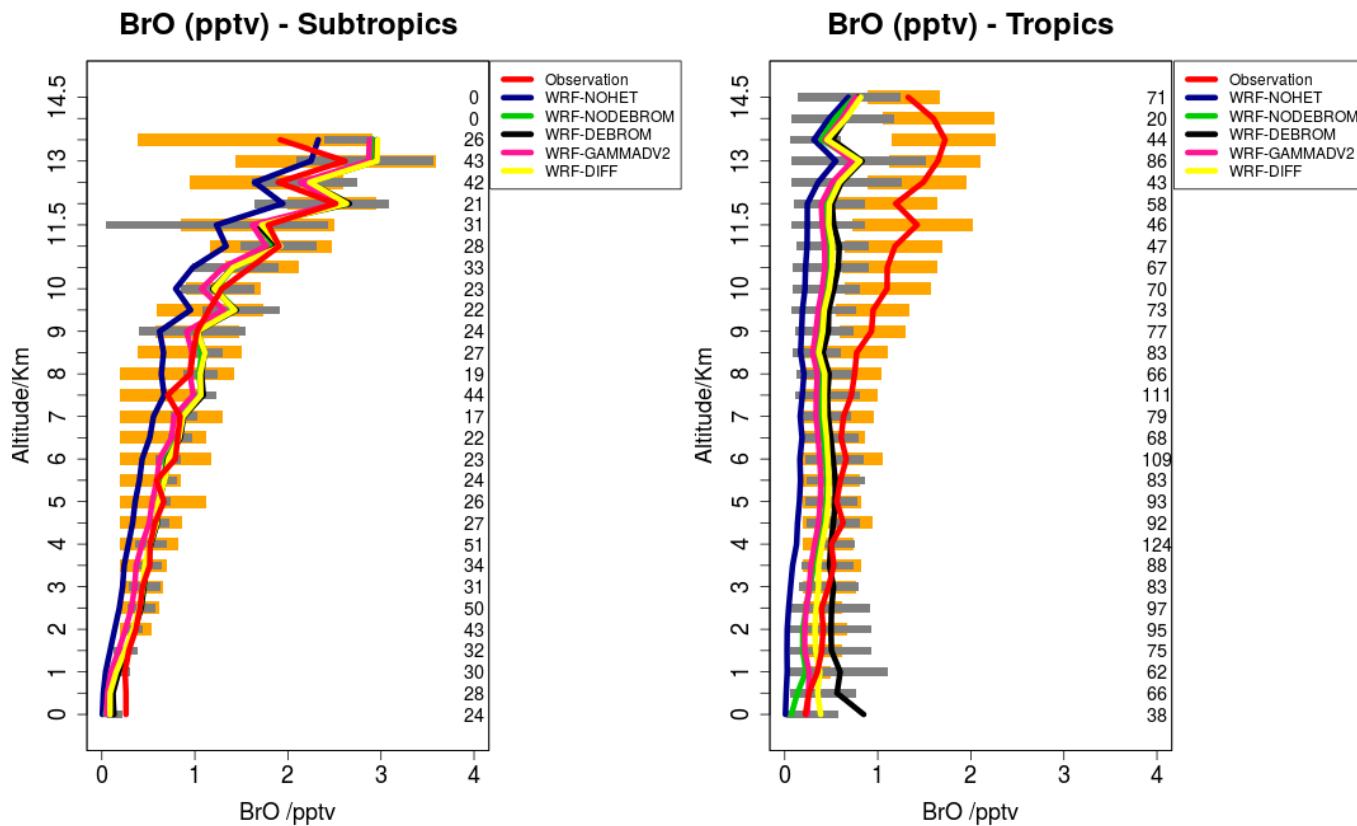
Figure 7. Mean vertical profile of BrO (pptv) over the subtropics (left) and tropics (right). An average over 16 flights of the TORERO campaign (red line) are compared to the 4-5 different WRF-Chem simulations: WRF-NOHET (blue line), WRF-NODEBROM (green line), WRF-DEBROM (black line) and WRF-GAMMADV2 (pink line) and WRF-DIFF (yellow line). Orange and grey horizontal bars indicate the 25th-75th quartile interval for the observations of the TORERO campaign and WRF-DEBROM simulation, respectively. Values are considered in 0.5 km bins and the number of aircraft measurement points for each altitude are given on the right side of each plot.
