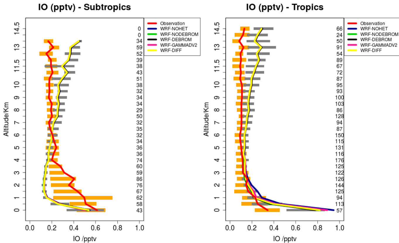
Figure 9. Mean vertical profile of IO (pptv) over the subtropics (left) and tropics (right). An average over 16 flights of the TORERO campaign (red line) are compared to the 4-5 different WRF-Chem simulations: WRF-NOHET (blue line), WRF-NODEBROM (green line), WRF-DEBROM (black line) and WRF-GAMMADV2 (pink line) and WRF-DIFF (yellow line). Orange and grey horizontal bars indicate the 25th-75th quartile interval for the observations of the TORERO campaign and WRF-DEBROM simulation, respectively. Values are considered in 0.5 km bins and the number of aircraft measurement points for each altitude are given on the right side of each plot.
