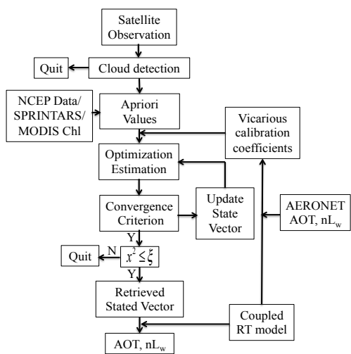
Figure 1: Flow chart of retrieval algorithm.
