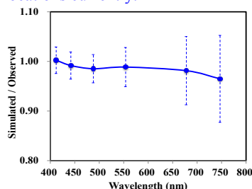
Figure: Averaged vicarious calibration coefficient for each channel.
