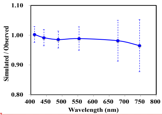
Figure 4: Averaged vicarious calibration coefficient for each channel.
