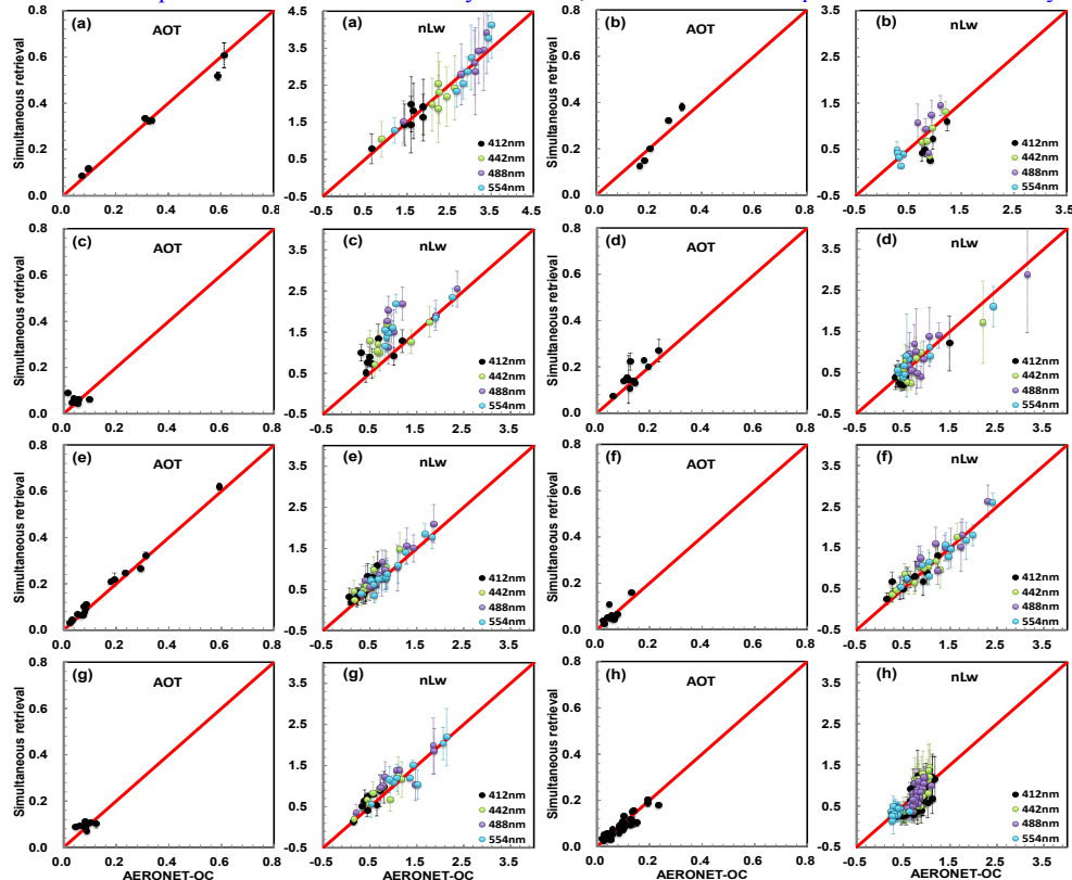
10 Figure: Comparison of satellite simultaneously retrieved AOT at 550 nm and nL w (mw sr -1 cm -2 μm -1 ) with AERONET-OC observations. Red line represents the 1:1 line (a: Ieodo_Station; b: GOT_Seaprisim; c: Lucinda; d: Abu_Al_Bukhoosh; e: Galata_Platform; f: COVE_SEAPRISM; g: Thornton_C-power; h: USC_SEAPRISM).
