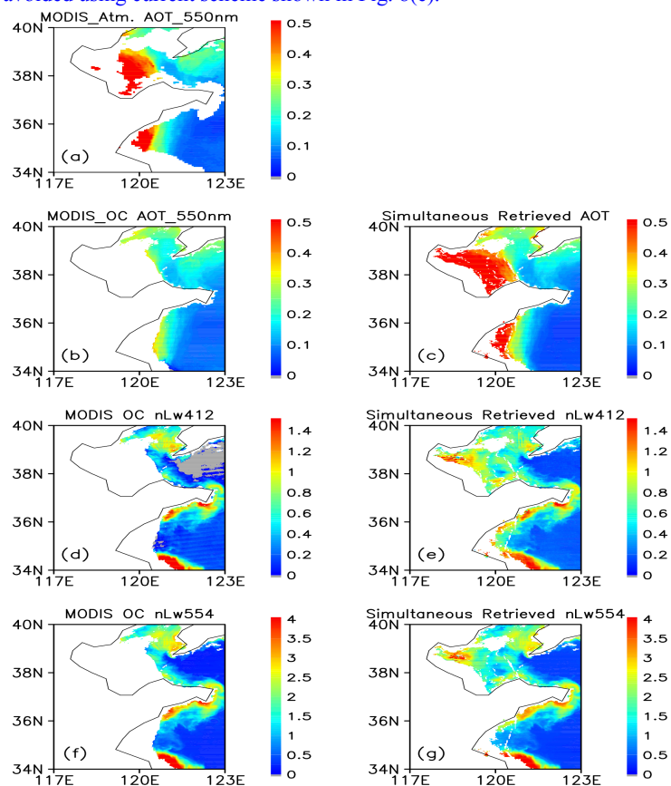
Figure 8: Comparison of satellite simultaneously retrieved AOT at 550 nm and nL_w ( mw\ sr^{-1}\ cm^{-2}\ \mu m^{-1} ) at 412 nm and 554 nm with MODIS operational products over East China Sea on 18 th Oct. 2011. (a) MODIS Aerosol AOT products; (b), (d), (f) MODIS Ocean Color AOT and nL_w products; (c), (e), (g): Simultaneously retrieved AOT and nL_w in this study.
