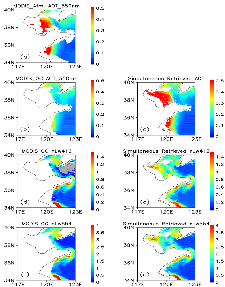
Figure 8: Comparison of satellite simultaneously retrieved AOT at 550 nm and nL_w ( \text{mw sr}^{-1} \text{cm}^{-2} \mu\text{m}^{-1} ) at 412 nm and 554 nm with MODIS operational products over East China Sea on 18 th Oct. 2011. (a) MODIS Aerosol AOT products; (b), (d), (f) MODIS Ocean Color AOT and nL_w products; (c), (e), (g): Simultaneously retrieved AOT and nL_w in this study
