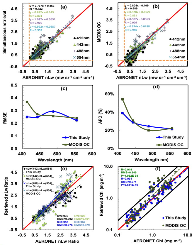
Figure 7: Comparison of jointly retrieved nL_w at 412, 442, 488 and 554 nm from simultaneous retrieval algorithm (a) and MODIS OC products (b) using measurements out of sun glint with AERONET in situ observation; Statistical values of RMSE (c), APD (d), band ratios of nL_w(442)/nL_w(554) and nL_w(488)/nL_w(554) (e), and Chl (f) results retrieved by the two approaches compared with AERONET-OC products. The upper and lower black lines of (f) are 1:2 and 2:1, respectively. The dashed lines are denoted as regression lines, which are corresponding to the retrieved results with same colors.
