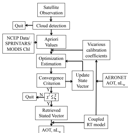
Figure1. Flow chart of retrieval algorithm
