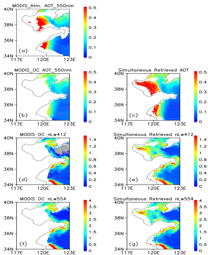
Figure8: Comparison of satellite simultaneously retrieved AOT at 550 nm and nL_w ( mw\ sr^{-1}\ cm^{-2}\ \mu m^{-1} ) at 412 nm and 554 nm with MODIS operational products over East China Sea on 18 th Oct. 2011. (a) MODIS Aerosol AOT products; (b), (d), (f) MODIS Ocean Color AOT and nL_w products; (c), (e), (g): Simultaneously retrieved AOT and nL_w in this study
