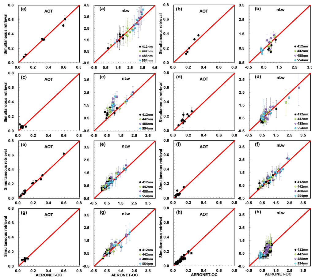
Figure 5: Comparison of satellite simultaneously retrieved AOT at 550 nm and nL_w ( mw\ sr^{-1}\ cm^{-2}\ \mu m^{-1} ) with AERONET-OC observations. Red line represents the 1:1 line (a: Ieodo_Station; b: GOT_SeaprisM; c: Lucinda; d: Abu_Al_Bukhoosh; e: Galata_Platform; f: COVE_SEAPRISM; g: Thornton_C-power; h: USC_SEAPRISM).
