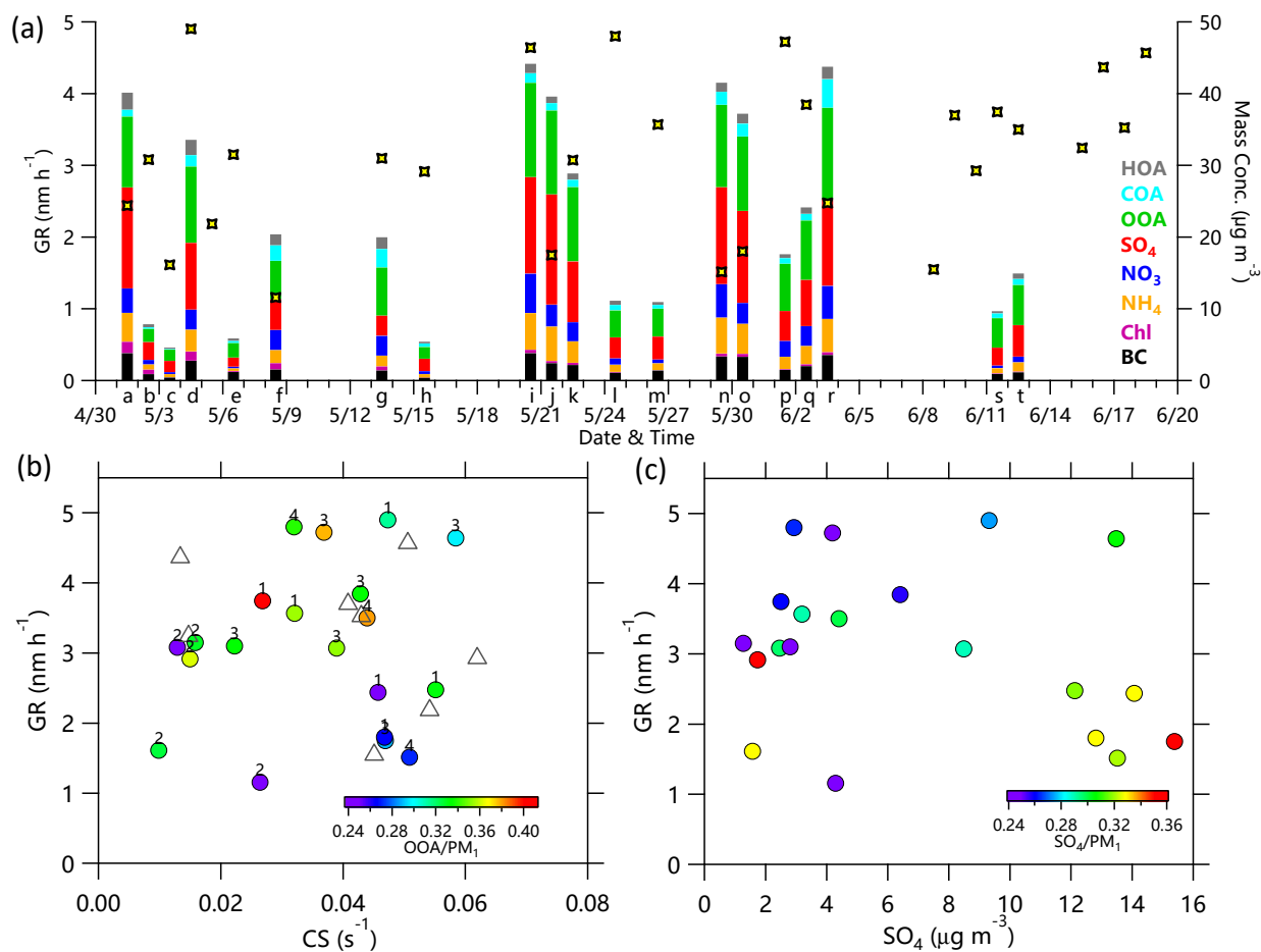
Figure 10: (a) Particle growth rates (GR) and the corresponding aerosol composition during the growth period, (b) the relationship between GR and CS, color-coded by OOA/PM 1 , and (c) the relationship between GR and sulfate concentration, color-coded by SO 4 /PM 1 . The numbers over the circles in (b) represent different source regions (Fig. 11) and the triangles represent data without information about composition.
