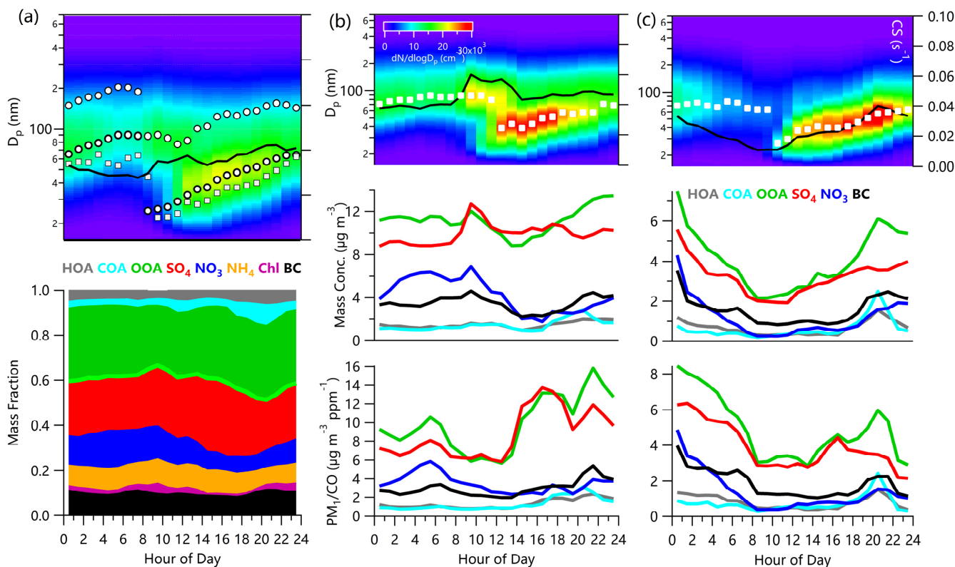
525 Figure 9: Average diurnal evolution of particle number size distributions and aerosol composition for new particle growth events during (a) the entire study, (b) polluted events, and (c) clean periods. The black solid lines in the top three panels show the diurnal cycles of CS. The circles and squares show the GMD from the log-normal fitting from this study and in Beijing (Du et al., 2017), respectively. The average diurnal cycles of aerosol species and CO-normalized aerosol species during polluted events and clean periods are shown in (b) and (c).
