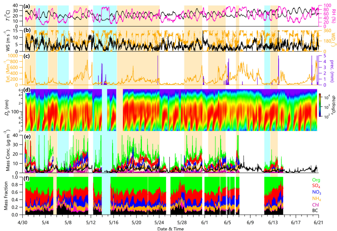
495 Figure 3: Time series of (a) temperature ( T , in black) and relative humidity (RH, in magenta), (b) wind direction (WD, in orange) and wind speed (WS, in black), (c) particle extinction coefficient (Ext., in orange) and precipitation (Precip., in purple), (d) particle number size distribution, (e) mass concentrations of Org, \text{NO}_3 , \text{SO}_4 , \text{NH}_4 , Chl, and BC, and (f) mass fractional contribution of chemical species to total \text{PM}_{10} . Polluted events (PE) and clean periods (CP) are marked as shaded orange and blue areas, respectively.
