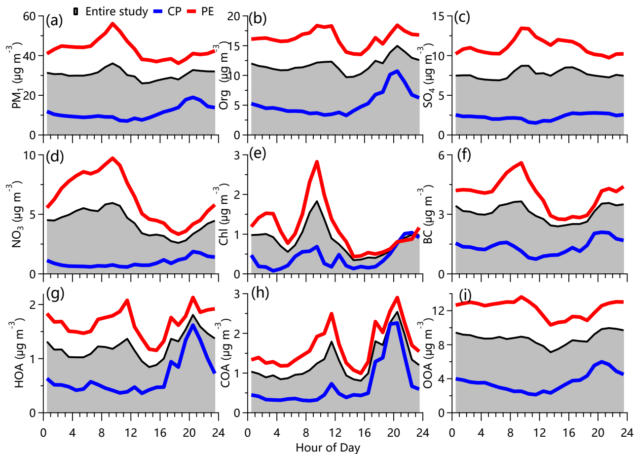
Figure 4. Average diurnal cycles of chemical species of \text{PM}_1 and OA factors during the entire study period, polluted events (PE) and clean periods (CP).
