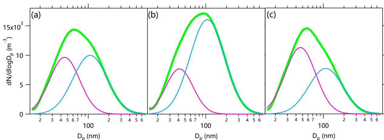
520 Figure 8: Average particle number size distributions during (a) the entire study, (b) polluted events, and (c) clean periods.
