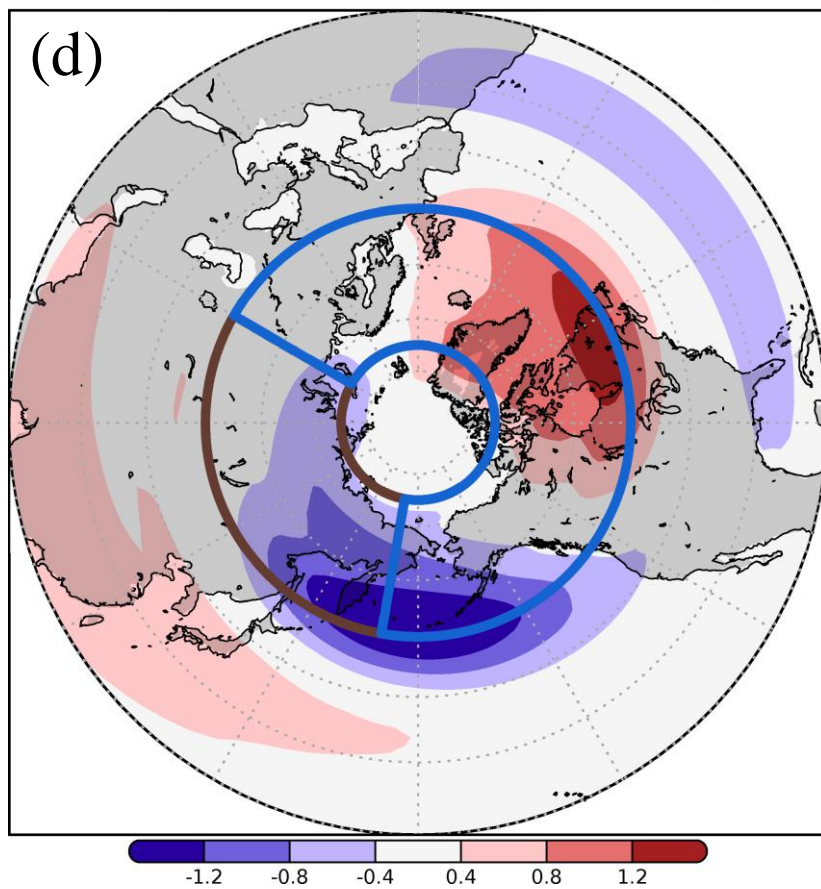
Figure A6. Same as Fig. A5, but for air temperature at 850 hPa ( ^{\circ}\text{C} ).
