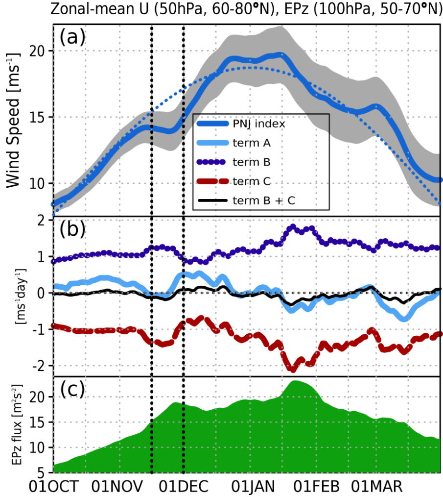
Figure 2. Time series of climatological 15-day running means of the (a) PNJ index (m s -1 , dark blue) (same as Fig. 1b); the sinusoidal regression expression of the PNJ index ( \hat{f}(t) = 10.36 \sin(2\pi t/365 + 1.54) + 7.52 ( t=1 : 01JAN), dark blue dotted line); the standard error of the PNJ index (gray shading); (b) the temporal tendency of the PNJ (i.e., zonal acceleration [m s -1 day -1 ]; Term A in equation (A3), light blue line), the Coriolis force acting on the residual mean meridional circulation and the meridional advection of zonal momentum (m s -1 day -1 , Term B in equation (3), purple line) at 50 hPa, and the EP flux divergence (m s -1 day -1 , Term C in equation (3), red line) at 50 hPa averaged over latitudes 60–80°N; the sum of Term B and Term C (black line); and (c) the vertical component of EP flux ( F^z ) at 100 hPa (m 2 s -2 ) averaged over latitudes 50–70°N from 1 October through 31 March. The vertical black dotted lines indicate the period of the late November short break.
