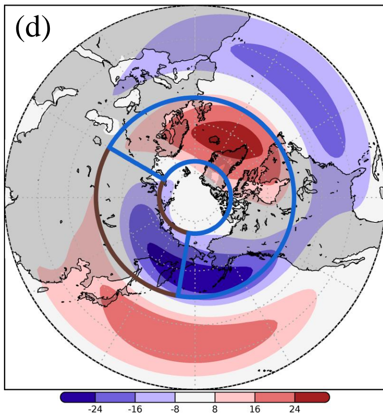
Figure A5. Zonal anomalies of climatological geopotential height at 500 hPa (m) during (a) early November, (b) late November, and (c) early December. (d) Late November deviations calculated by equation (4) (see Section 3.3) with wavenumber decomposition; only planetary-scale components, wavenumbers 1 to 2, were used. The brown (60–170°E, 50–75°N) and blue (170°E–60°W, 50–75°N) boxes indicate the averaging areas used for calculating the fields shown in Fig. 5.
