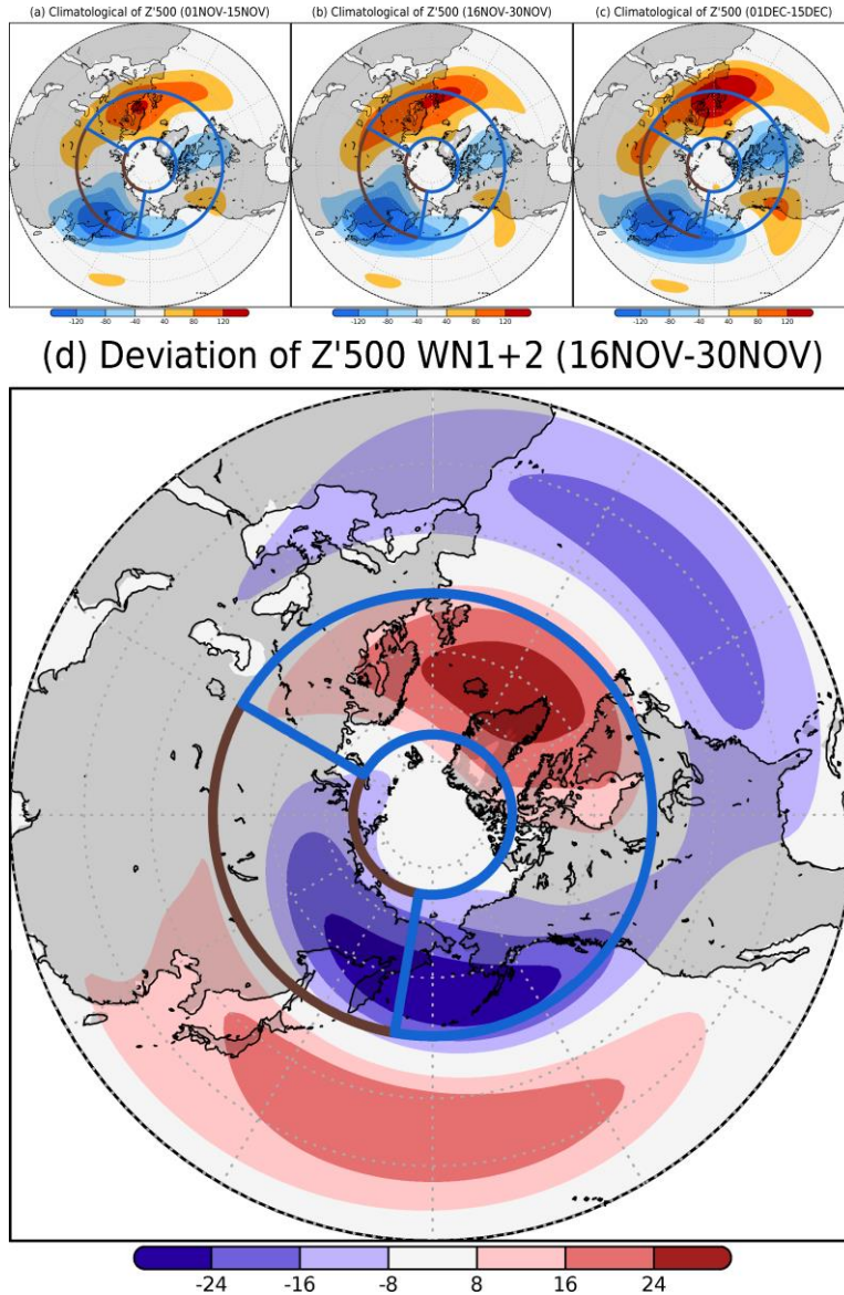
Figure A5D5. Zonal anomalies of climatological geopotential height at 500 hPa (m) during (a) early November, (b) late November, and (c) early December. (d) Late November deviations calculated by equation (4) (see Section 3.3) with wavenumber decomposition; only planetary-scale components, wavenumbers 1 to 2, were used. The brown (60–170°E, 50–75°N) and blue (170°E–60°W, 50–75°N) boxes indicate the averaging areas used for calculating the fields shown in Fig. 5.
