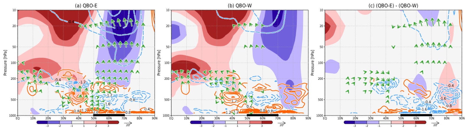
Figure B2E2. Same as Fig. A1d, but (a) for QBO-E, (b) for QBO-W, and (c) difference of (QBO-E) – (QBO-W).
