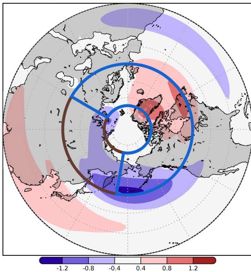
Figure A6D6. Same as Fig. A5D5, but for air temperature at 850 hPa (°C).
