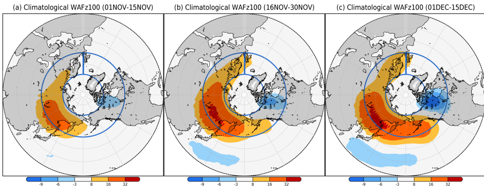
Figure A2D2. Vertical component of the climatological wave activity flux (Plumb, 1985) at 100 hPa ( 10^{-3} \text{ m}^2 \text{ s}^{-2} ) during (a) early November, (b) late November, and (c) early December. The box outlined in blue (0–360°E, 50–70°N) indicates the averaging area used for calculating the fields shown in Fig. A3D3.
