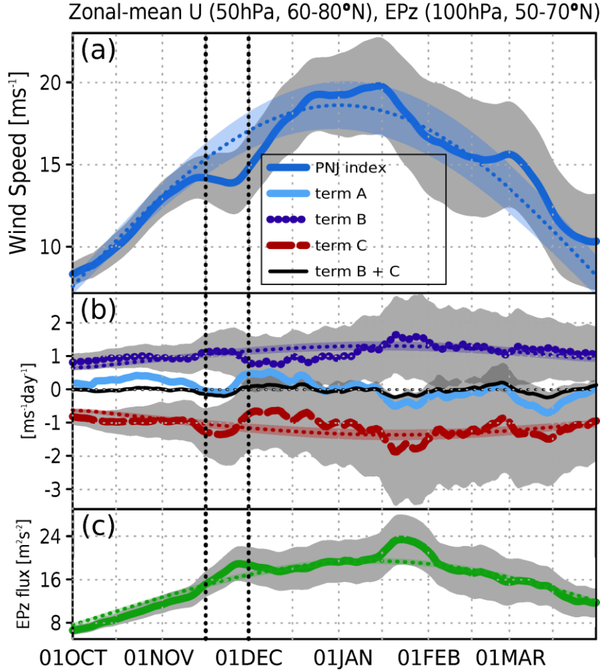
Figure 2. Time series of climatological 15-day running means of the (a) PNJ index ( \text{m s}^{-1} , dark blue) (same as Fig. 1b); the sinusoidal regression expression of the PNJ index ( \hat{f}(t) = 10.36 \sin(2\pi t/365 + 1.54) + 7.52 (t=1:01\text{JAN}) , dark blue dotted line); the standard error 95% confidence interval of the PNJ index (gray shading); (b) the temporal tendency of the PNJ (i.e., zonal acceleration [ \text{m s}^{-1} \text{ day}^{-1} ]; Term A in equation (A33), light blue line), the Coriolis force acting on the residual mean meridional circulation and the meridional advection of zonal momentum ( \text{m s}^{-1} \text{ day}^{-1} , Term B in equation (3), purple line) at 50 hPa, and the EP flux divergence ( \text{m s}^{-1} \text{ day}^{-1} , Term C in equation (3), red line) at 50 hPa averaged over latitudes 60–80°N; the sum of Term B and Term C (black line); the sinusoidal term B (purple dotted line), the sinusoidal term C (red dotted line); the 95% confidence interval of them (color shading); and (c) the vertical component of EP flux ( F^Z ), the sinusoidal of that (green dotted line), the 95% confidence interval of them (color shading) at 100 hPa ( \text{m}^2 \text{ s}^{-2} ) averaged over latitudes 50–70°N from 1 October through 31 March. The vertical black dotted lines indicate the period of the late November short break.
