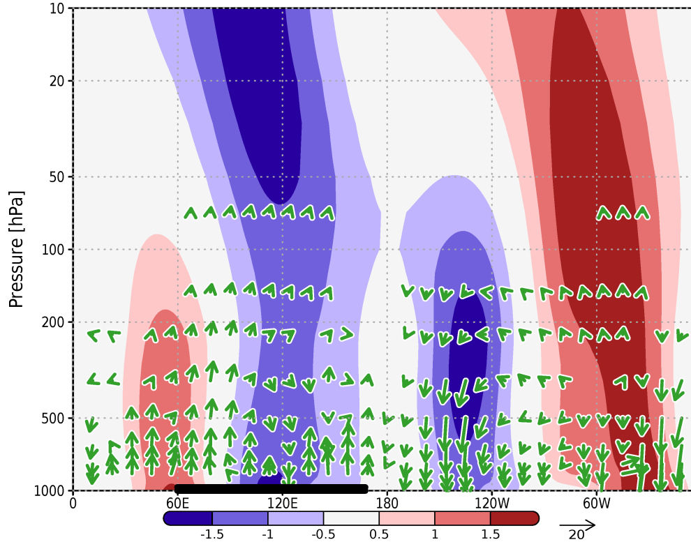
Figure A3D3. Zonal anomalies of climatological geopotential height (m, color shading) and zonal and vertical components of WAF ( 10^{-3} \text{ m}^2 \text{ s}^{-2} , vectors), averaged over latitude 50\text{--}70^\circ\text{N} (inside the blue box in Fig. A2) during (a) early November, (b) late November, and (c) early December. (d) Late late November field deviations calculated by equation (4) (see Section 3.3). The geopotential height is normalized by the standard deviation at each height. The WAF magnitude is standardized by pressure ( p \text{ p}_s^{-1} , p_s is a standard sea-level pressure) and the square of the radius of the Earth ( 6.37 \times 10^6 \text{ m} ). The vertical components of the vectors are multiplied by a factor of 500. The black line indicates the latitudinal range for Siberia ( 60\text{--}170^\circ\text{E} ).
