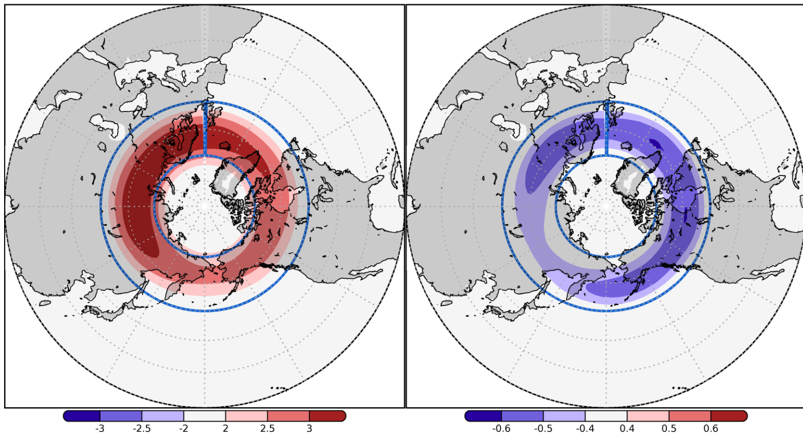
Figure A7D7. Same as Fig. 4, but with wavenumber decomposition; (a) wavenumber 1 and (b) wavenumber 2.
