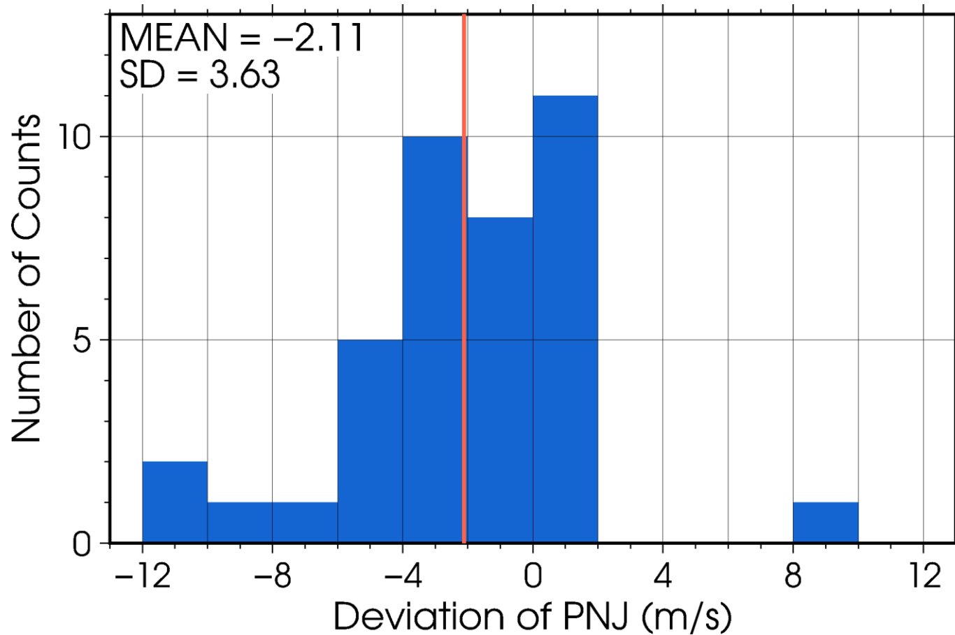
Figure C1. Histogram of the deviation Appendix C. Histogram of the short break of the PNJ in late November
