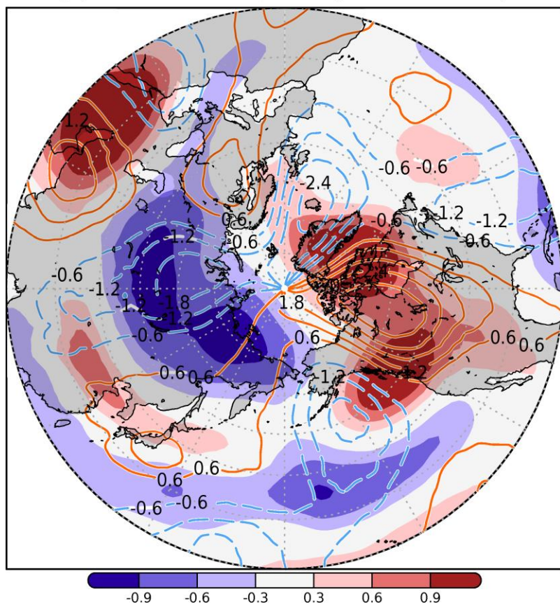
Figure A4D4. Zonal anomalies of climatological meridional wind ( \text{m s}^{-1} , contours) and air temperature ( ^{\circ}\text{C} , color shading) at 100 hPa during (a) early November, (b) late November, and (c) early December. (d) Late late November deviations calculated by equation (4) (see Section 3.3).
