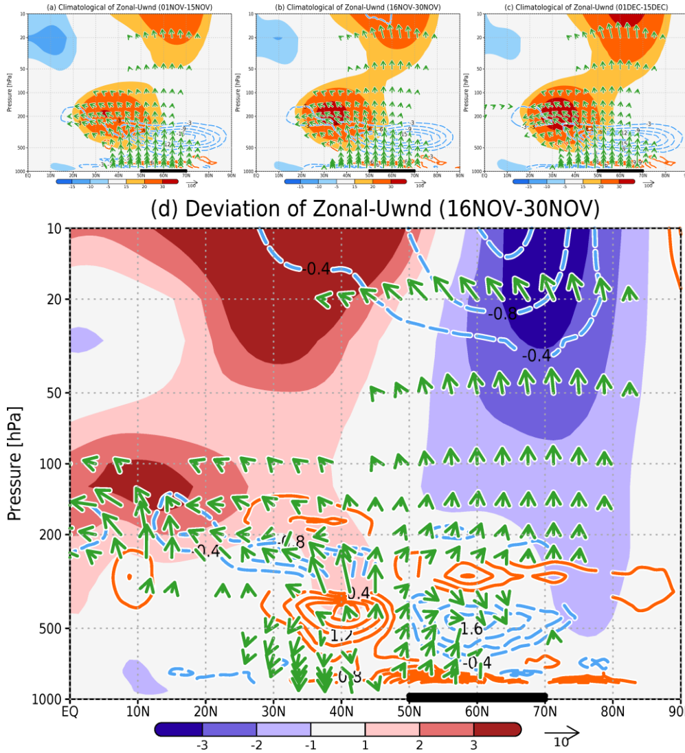
Figure A4D1. Climatological zonal-mean zonal wind speed ( \text{m s}^{-1} , color shading), EP flux ( \text{m}^2 \text{s}^{-2} , vectors), and the flux divergence ( \text{m s}^{-1} \text{day}^{-1} , contours) during (a) early November (1–15 November), (b) late November (16–30 November), and (c) early December (1–15 December). (d) Late late November deviations (late November deviations from the expected sinusoidal regression expression calculated with equation (4); see Section 3.3). The EP flux is standardized by density ( 1.225 \text{ kg m}^{-3} ) and the radius of the Earth ( 6.37 \times 10^6 \text{ m} ). The vertical component of the vectors is multiplied by a factor of 250. The bold black line indicates the longitudinal range for Siberia ( 50\text{--}70^\circ\text{N} ).
