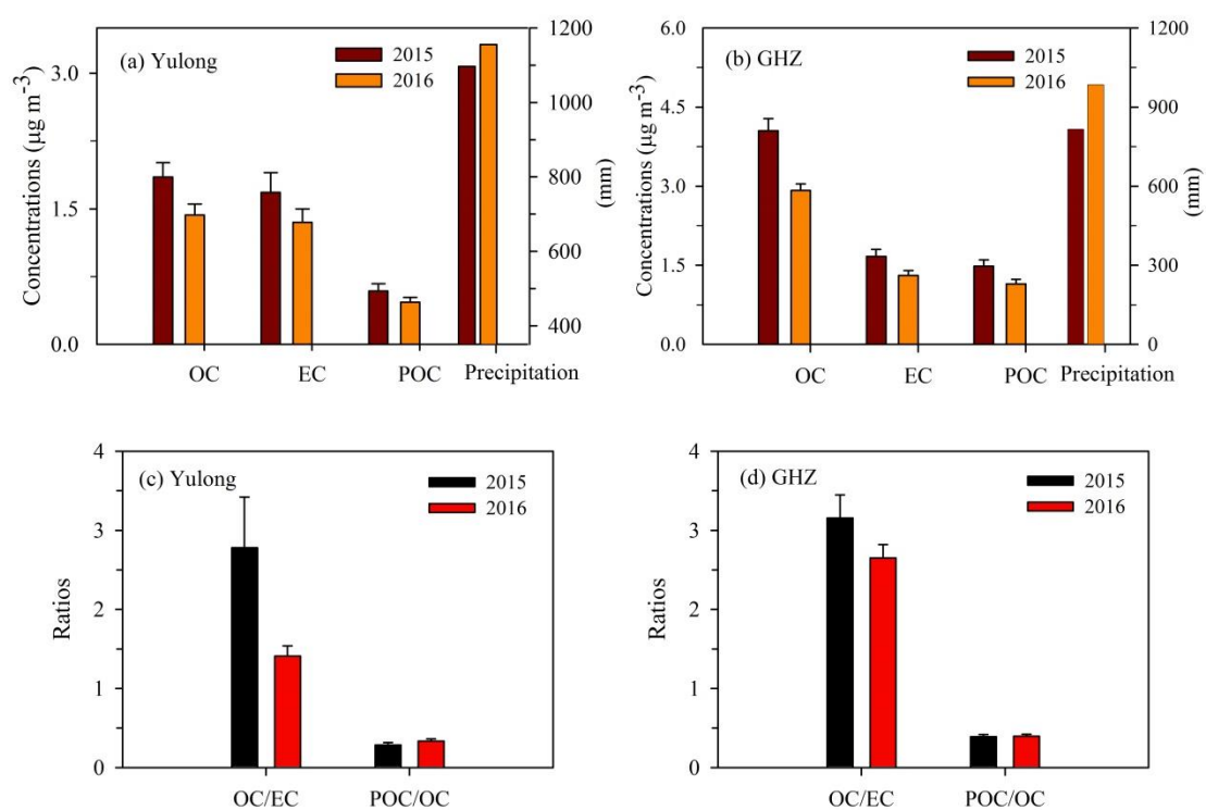
Fig. 11 Inter-annual differences of OC, EC, and POC concentrations at (a) Yulong and (b) GHZ site. Precipitation at Mt. Yulong and GHZ sites in different years was also plotted in (a) and (b). The OC/EC, and POC/OC ratios are shown in (c, d).
