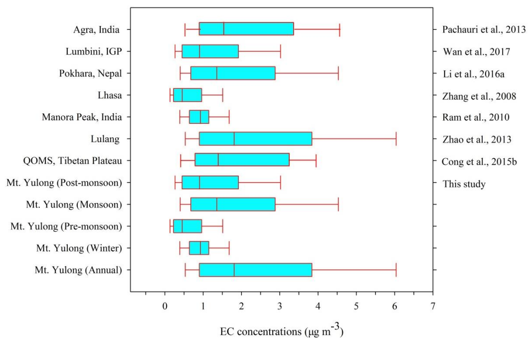
Fig. 12 1 Comparison of EC concentrations in aerosols from Mt. Yulong and other areas of interest.
