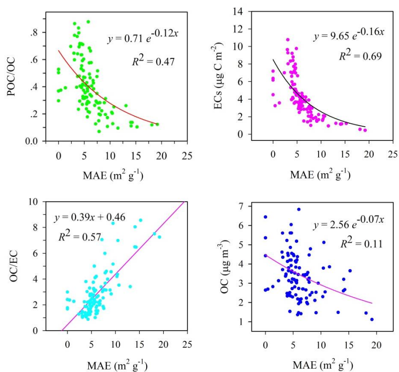
Fig. 10 Regression analysis for scatter plot between EC MAE and POC/OC, OC/EC ratios, and EC s , OC concentrations for aerosols sampled at GHZ.
