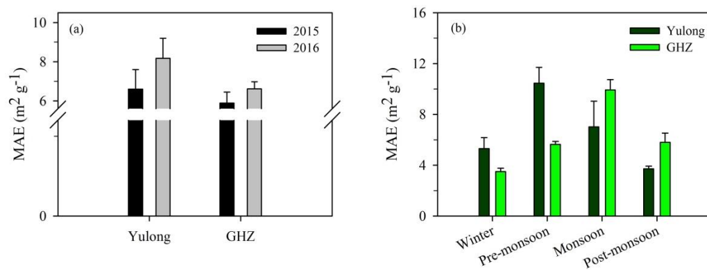
Fig. 8 Histogram of (a) annual mean and (b) seasonal mean MAE values of atmospheric EC from Mt. Yulong and GHZ sampling sites during December 2014-December 2016.
