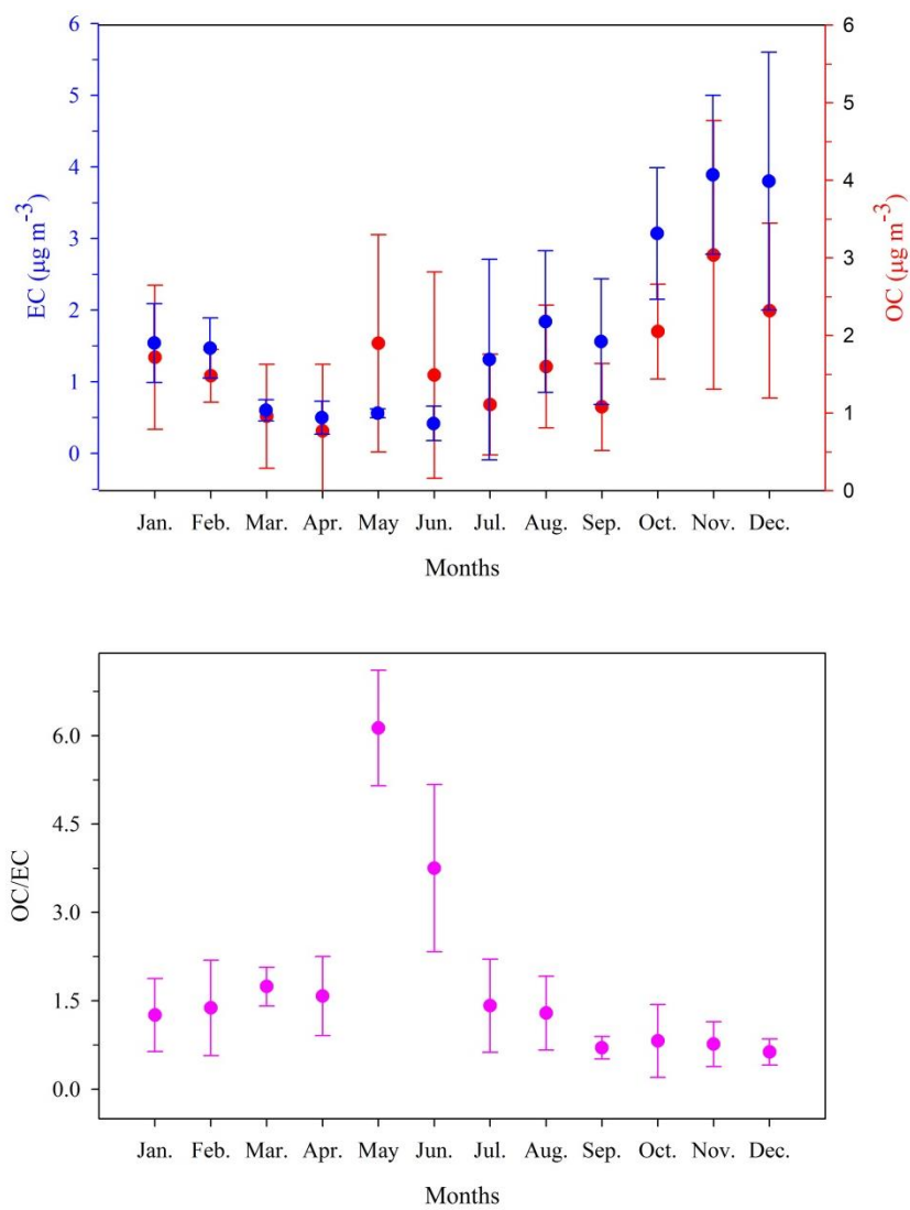
Fig. 6 Monthly averaged EC, OC concentrations and OC/EC ratios from Mt. Yulong.
