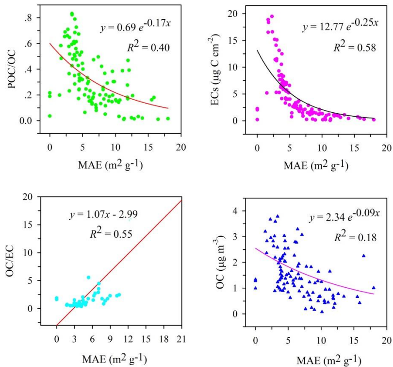
Fig. 9 Regression analysis for scatter plot between EC MAE and POC/OC, OC/EC ratios, and EC s , OC concentrations for aerosols sampled at Mt. Yulong.
