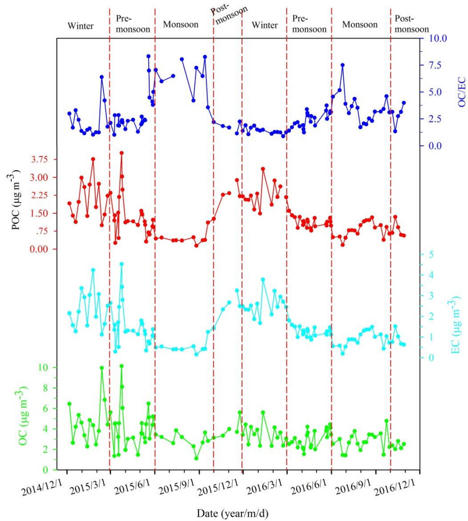
Fig. 5 Seasonal variations of EC, OC, and POC concentrations and OC/EC ratio from GHZ basin during Dec. 2014-Dec. 2016.
