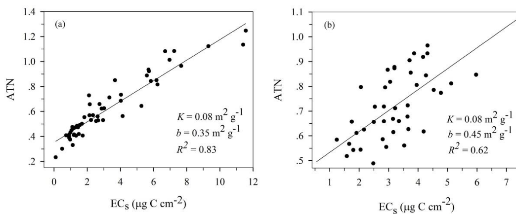
Fig. 3 Dependence of optical attenuation (ATN) detected at 632 nm on the EC loading ( EC_s ) for (a) the Mt. Yulong sampling site and (b) the GHZ sampling site. Results of linear regression are displayed with K as the slope and b as the intercept.
