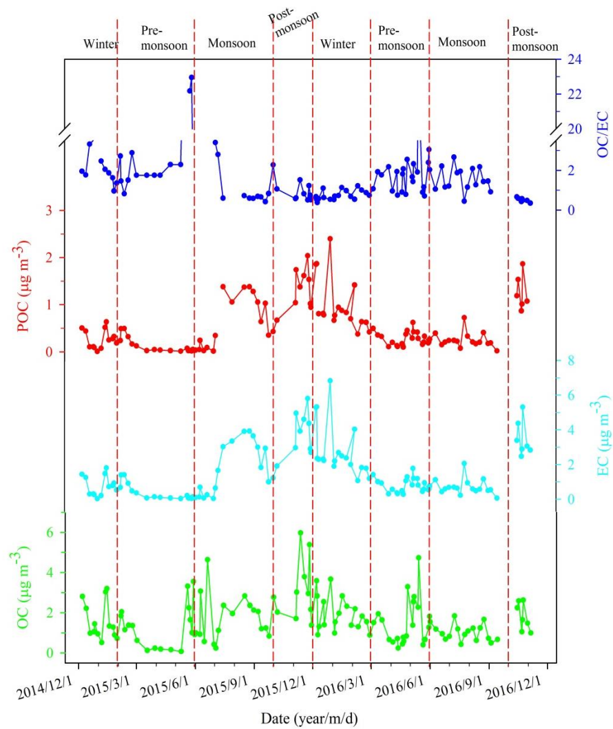
Fig. 4 Seasonal variations of EC, OC, and POC concentrations and OC/EC ratio from Mt. Yulong during Dec. 2014-Dec. 2016.
