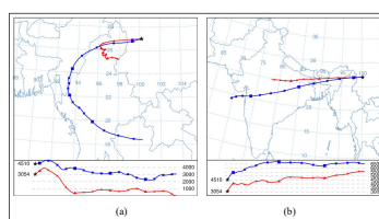
Fig. 7 Seven-day backward trajectory analysis with HYSPLIT model (a) in the monsoon and (b) post monsoon seasons during the study period (Source ★ at 27.01 N, 100.20 E). The trajectories of air mass in the plot were the average of a few episodes. The two heights are the elevation of Mt. Yulong and GHZ, respectively.
