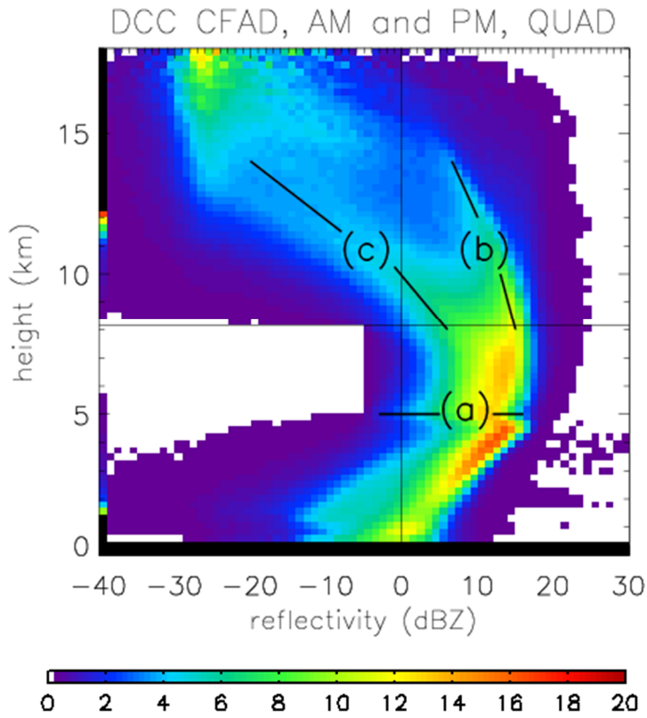
Figure 3. The Contoured Frequency by Altitude Diagrams (CFADs) of reflectivity for DCCs in Amazonia. The colors represent the probability density function (PDF, as percentage) of radar reflectivity at each 240 m-tall layer observed by CloudSat. The vertical (horizontal) black line indicates 0 dBZ (8 km). Three distinct features of the CFAD, discussed in the text, are labelled on the figure. (a) indicates the dark band, with the horizontal line segments showing the mean altitude. (b) and (c) mark the locations of the high and low reflectivity arcs, respectively. The diagonal line segments show the orientation of each arc, and the rough values of the PDF modes.
