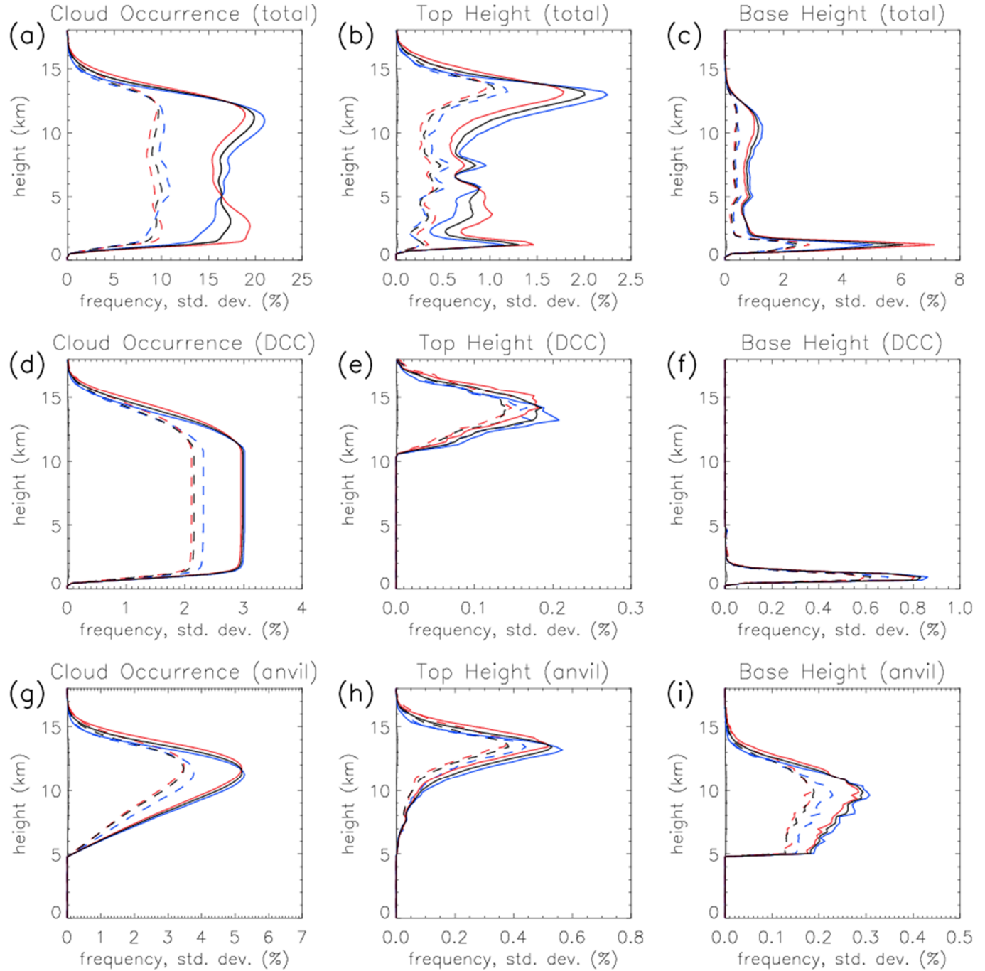
Figure 2. (Top) Vertical frequency profiles of (a) cloud occurrence, (b) cloud top heights (center), and (c) cloud base heights. Black lines are for day/night, and red (blue) is for day-only (night-only). Solid (dashed) line is the mean (standard deviation)
