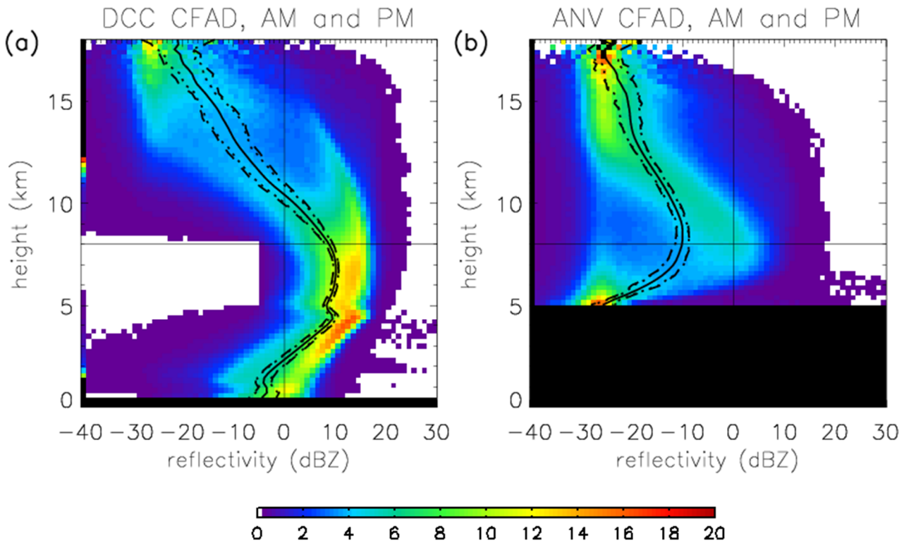
Figure 4. (a) The CFAD for DCCs, same as Fig. 3. The black curves near the center of the data are the average reflectivity profiles. Dashed lines are the standard deviation bounds. (b) Same as (a), but for anvils.
