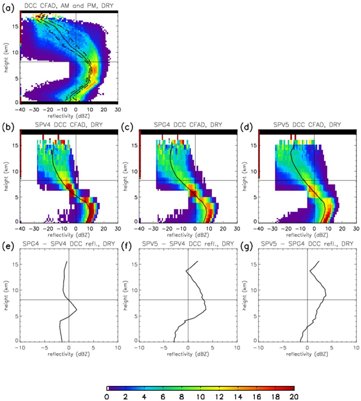
Figure 6. (a,b,c,d) CFADs of dry season DCC reflectivity in Amazonia from (a) CloudSat, (b) SPV4, (c) SPG4 (i.e. SPV4 with diagnosed graupel included), and (d) SPV5, as in Fig. 4.
