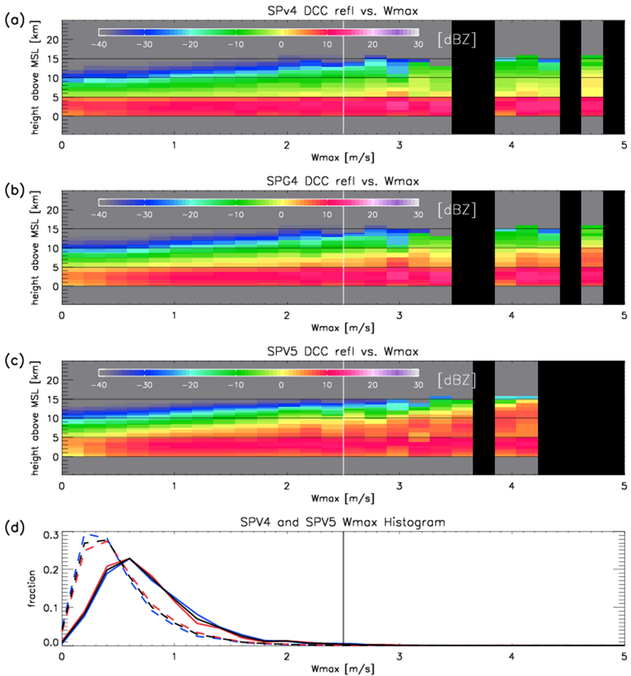
600 Figure 8. (a) Mean vertical profiles of simulated DCC radar reflectivity in SPV4 sorted by maximum updraft velocity. The vertical lines at 2.5 \text{ m s}^{-1} represent the maximum cut off W_{max} value for statistical calculations. Vertical black stripes are updraft values with no DCC occurrences.
