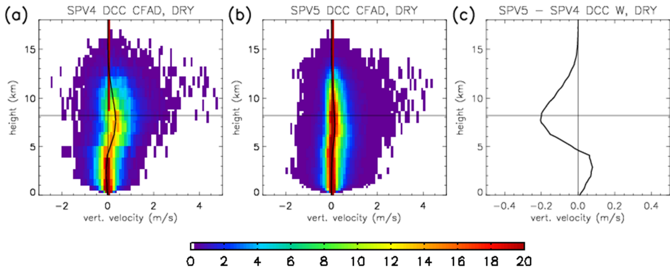
Figure 7. (a,b) CFADs of DCC vertical updraft velocity from (a) SPV4 and (b) SPV5. The format is the same as for the reflectivity CFADs. Note that SPV4 and SPG4 vertical velocities (not shown) are identical. (c) The difference between SPV4 and SPV5 mean vertical velocity profiles.
