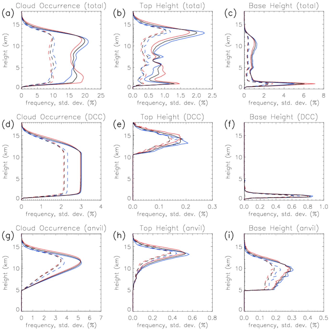
Figure 2. (Top) Vertical frequency profiles of (a) cloud occurrence frequency ( COF ), (b) cloud top height ( CTH ) frequency heights (center), and (c) cloud base height ( CBH ) frequency heights . Black lines are for day/night, and red (blue) is for day-only (night-only). Solid (dashed) line is the mean (standard deviation)
