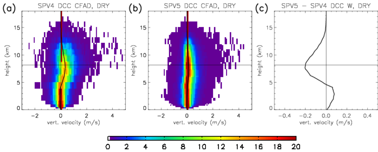
715 | Figure 7. (a,b) CFADs of DCC vertical updraft velocity from (a) SP-CAM version-4SPV4 and (b) SP-CAM version-5SPV5 . The format is the same as for the reflectivity CFADs. Note that SPV4 and SPG4 vertical velocities (not shown) are identical. (c) The difference between the version-4SPV4 and version-5SPV5 mean vertical velocity profiles.
