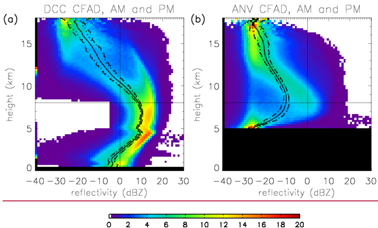
695 Figure 4. (a) The CFAD for DCCs, same as Fig. 3. The black curves near the center of the data are the average reflectivity profiles. Dashed lines are the standard deviation bounds. (b) Same as (a), but for anvils.
