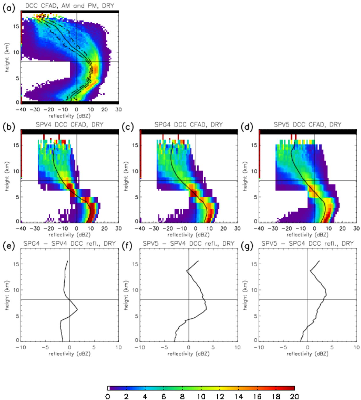
Figure 6. (a,b,c,d) CFADs of dry season DCC reflectivity in Amazonia from (a) CloudSat, (b) SP-CAM version 4-SPV4 , (c) SP-CAM version 4-SPG4 (i.e. SPV4 with diagnosed graupel included), and (d) SP-CAM version 5-SPV5 , as in Fig. 4.
