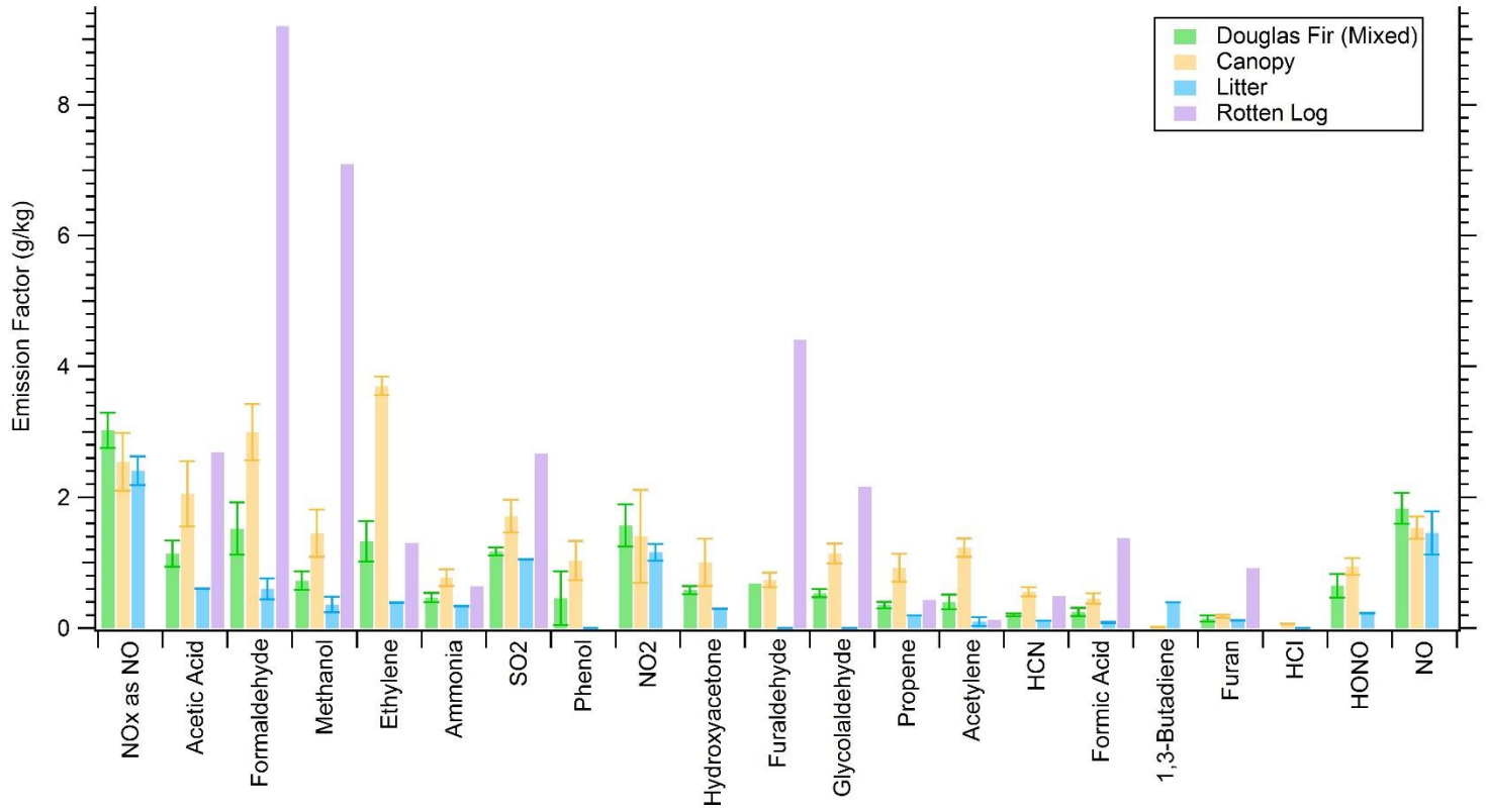
Figure 4. Trace gas emissions from mixed Douglas fir ecosystem (including sound, dead wood, but rotten log not included) and pure components. Sound dead wood was not burned separately except as untreated lumber.
