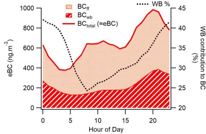
Figure 5: Diurnal cycle of BC_{wb} , BC_{ff} , BC_{total} and wood burning contribution to total BC (WB, defined as BC_{wb}/BC_{total} \times 100 ) at DEM station.
