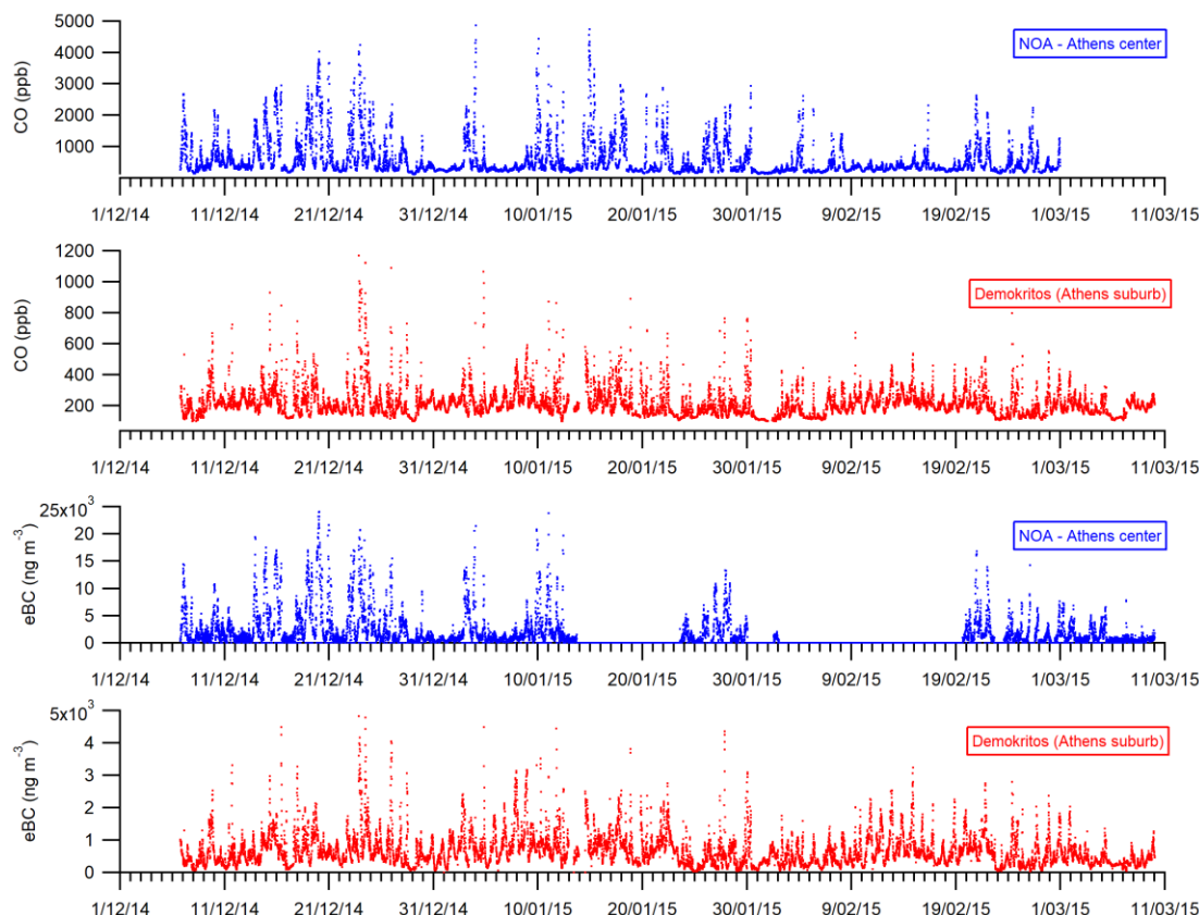
Figure 2: Time series of 10-minutes averaged CO and eBC concentrations measured at NOA (in blue) and DEM (red) monitoring stations from 6th December 2014 until 10th march 2015.
