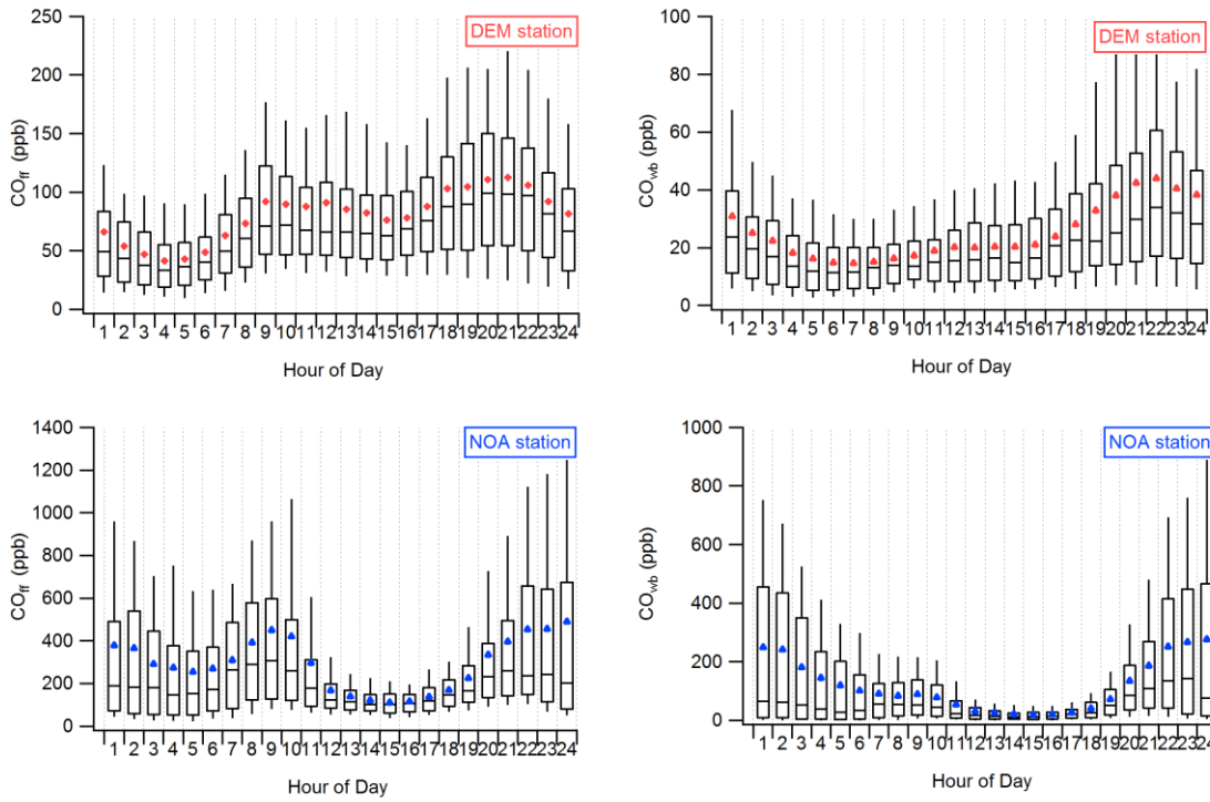
Figure 10: Diurnal variations of CO_{fr} (left) and CO_{wb} (right) at DEM (top) and NOA (bottom) stations. Data are presented as box and whisker plots, where boxes encompass values between the 25th and 75th percentiles, horizontal lines represent median values, and 'whiskers' give the 80% range of the values, whereas colored markers represent the mean values.
