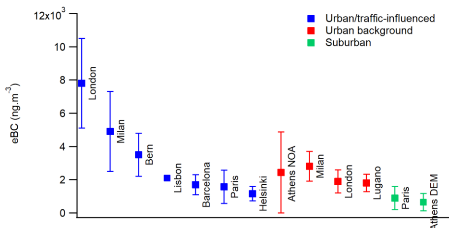
Figure 3: Levels of black carbon (mean±stdv) reported for various European cities, (blue) in traffic-influenced sites, such as London (year 2009, Reche et al., 2011), Milan (Summer 2010, Lisbon (June 2000, Alves et al., 2002), Barcelona (year 2009, Reche et al., 2011), Paris (summer 2009, Zhang et al., 2013) and Helsinki (winter 2000, Hitzengerger and Tohno, 2001); (red) in urban background/residential areas such as Milan (Summer 2010, Invernizzi et al., 2011), London (year 2009, Reche et al., 2011) and Lugano (year 2009, Reche et al., 2011), (green) a suburban area of Paris (Laborde et al., 2013), along with the results from this study at NOA and DEM stations in winter 2014-2015.
