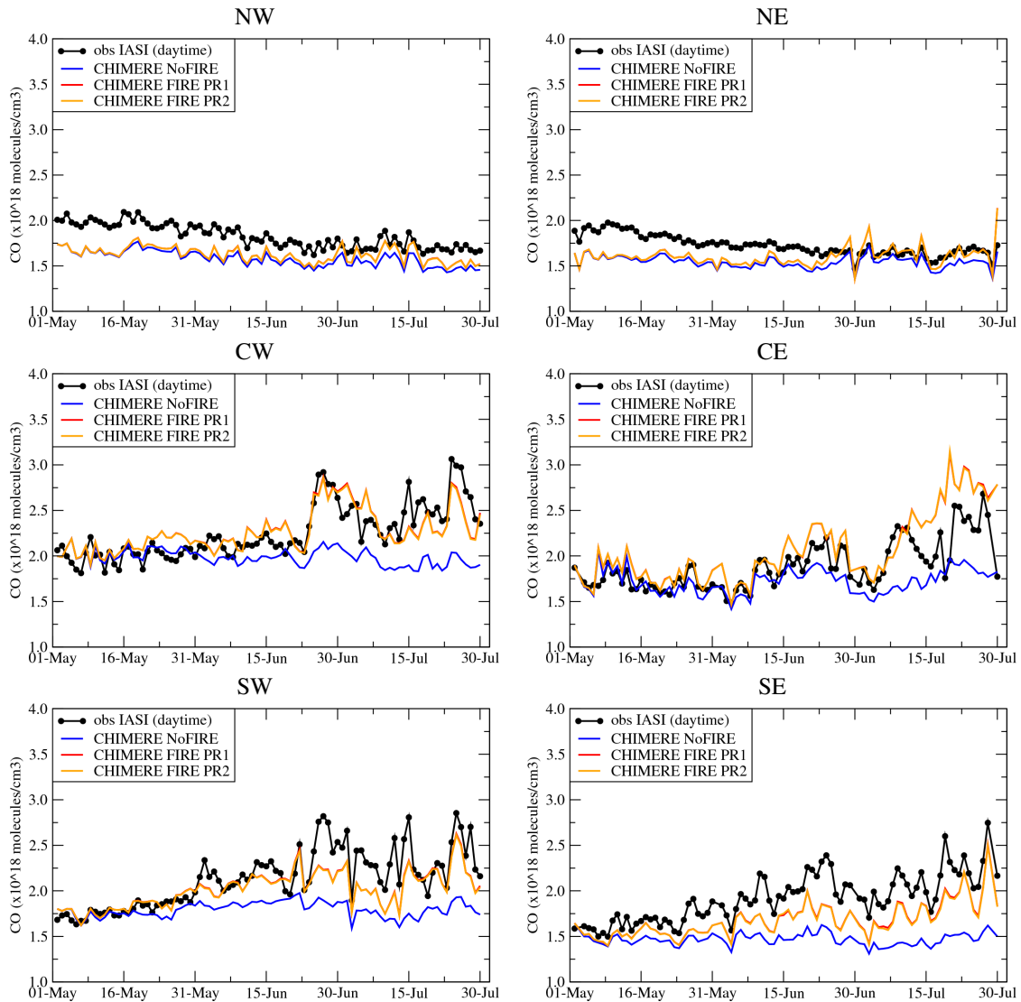
Figure 7. Time series of vertically integrated carbon monoxide ( CO column) in 10^{18} molecules/ cm^2 for IASI and for the simulations with CHIMERE.
