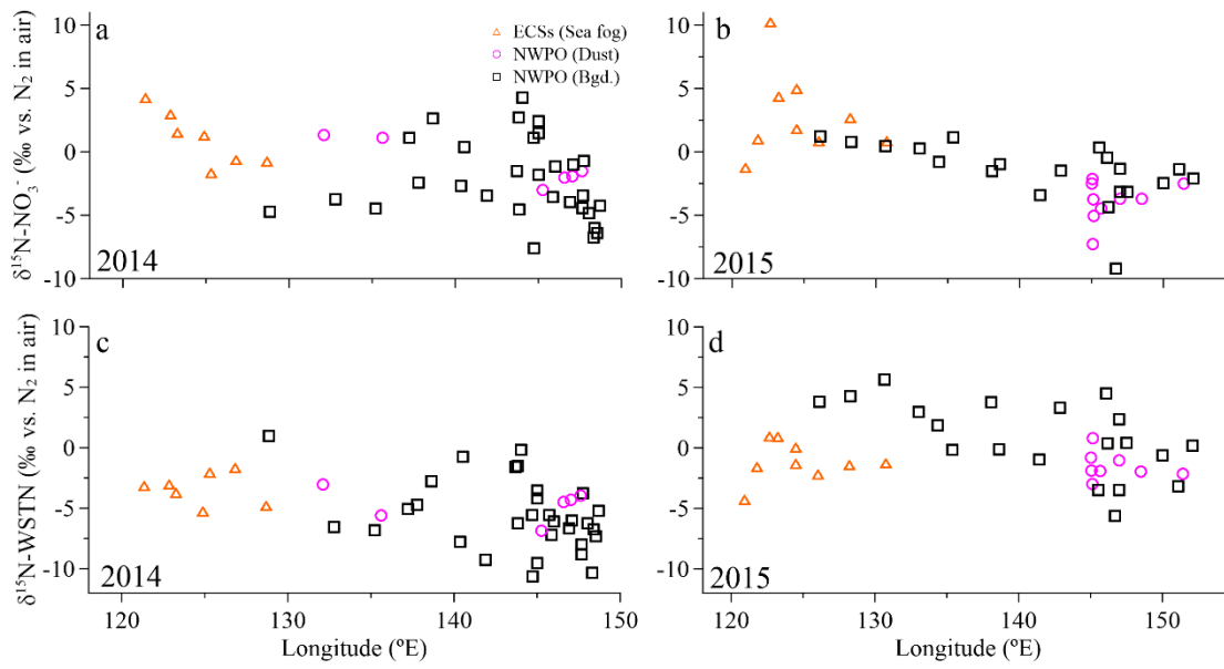
Figure 4. Aerosol \delta^{15}\text{N}-\text{NO}_3^- (a and b) and \delta^{15}\text{N}-\text{WSTN} (c and d) in the ECSs (the orange open triangles denote for sea-fog-modified aerosol), and in the NWPO (the pink open circles denote dust aerosol and the black open squares denote background aerosol) with longitude during the 2014 and 2015 cruise, respectively.
