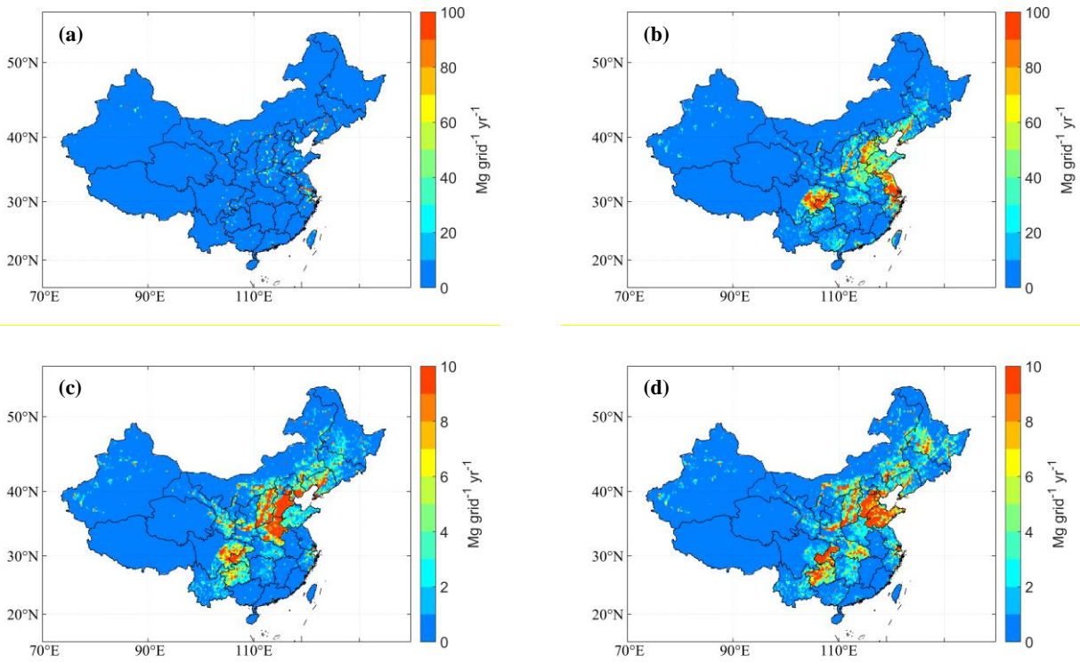
Figure S1 Spatial distribution of hydrogen chloride emissions from coal combustions in four economic sectors: power plant (a), industry (b), residential (c) and other (d).
