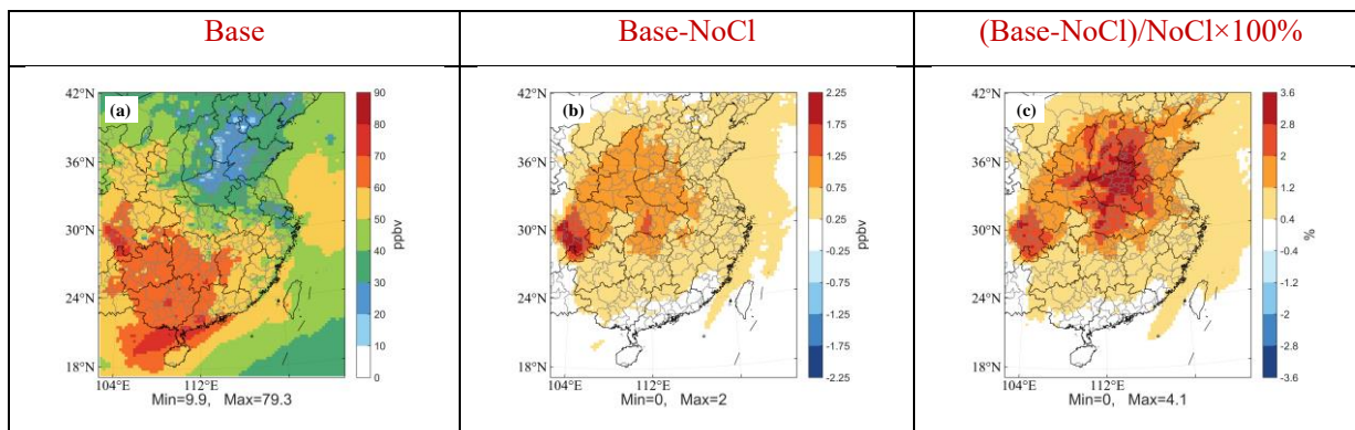
Figure R2 Comparison of the monthly mean concentrations of daily maximum 8-h \text{O}_3 in the Base experiment, the differences (Base minus NoCl), and the percent changes to the NoCl experiment.
