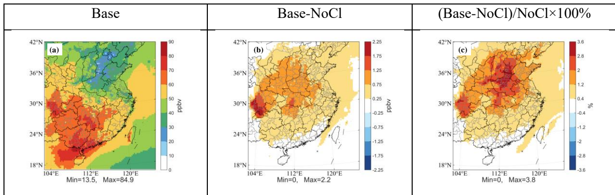
Figure S9 Comparison of the monthly mean concentrations of daily maximum 1-h \text{O}_3 in the Base experiment, the differences (Base minus NoCl), and the percent changes to the NoCl experiment.
