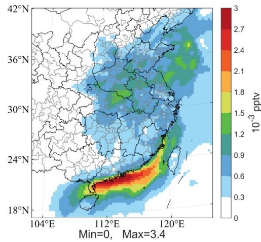
Figure S8 The monthly mean concentrations of \text{Cl}_2 in the NoCl experiment.
