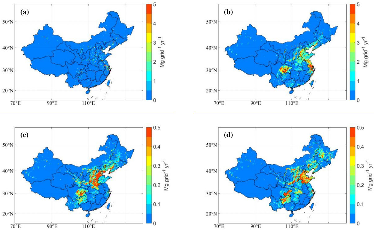
Figure S2 Spatial distribution of molecular chlorine emissions from coal combustions in four economic sectors: power plant (a), industry (b), residential (c) and other (d).
