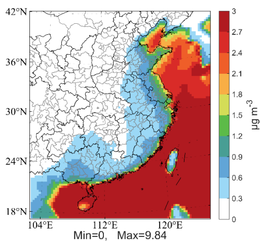
Figure S5 Spatial distribution of the monthly mean concentration of coarse particulate \text{Na}^+ . Coarse particulate \text{Na}^+ is the important composition in sea salt aerosol and is considered to be inactive.
