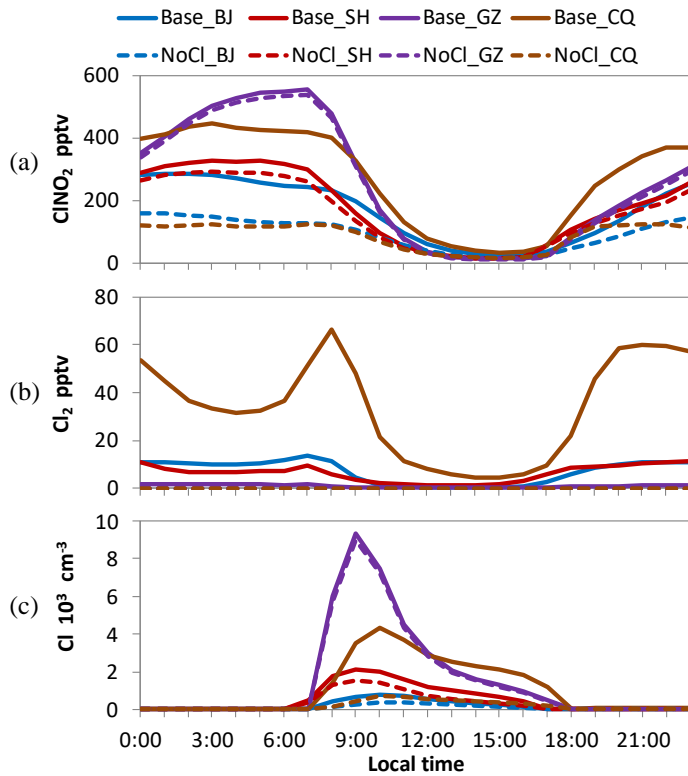
Figure 7: Diurnal variations of monthly mean concentrations of \text{ClNO}_2 (a), \text{Cl}_2 (b) and \text{Cl} radical (c) in Beijing, Shanghai, Guangzhou and Chongqing in the Base and NoCl experiments.
