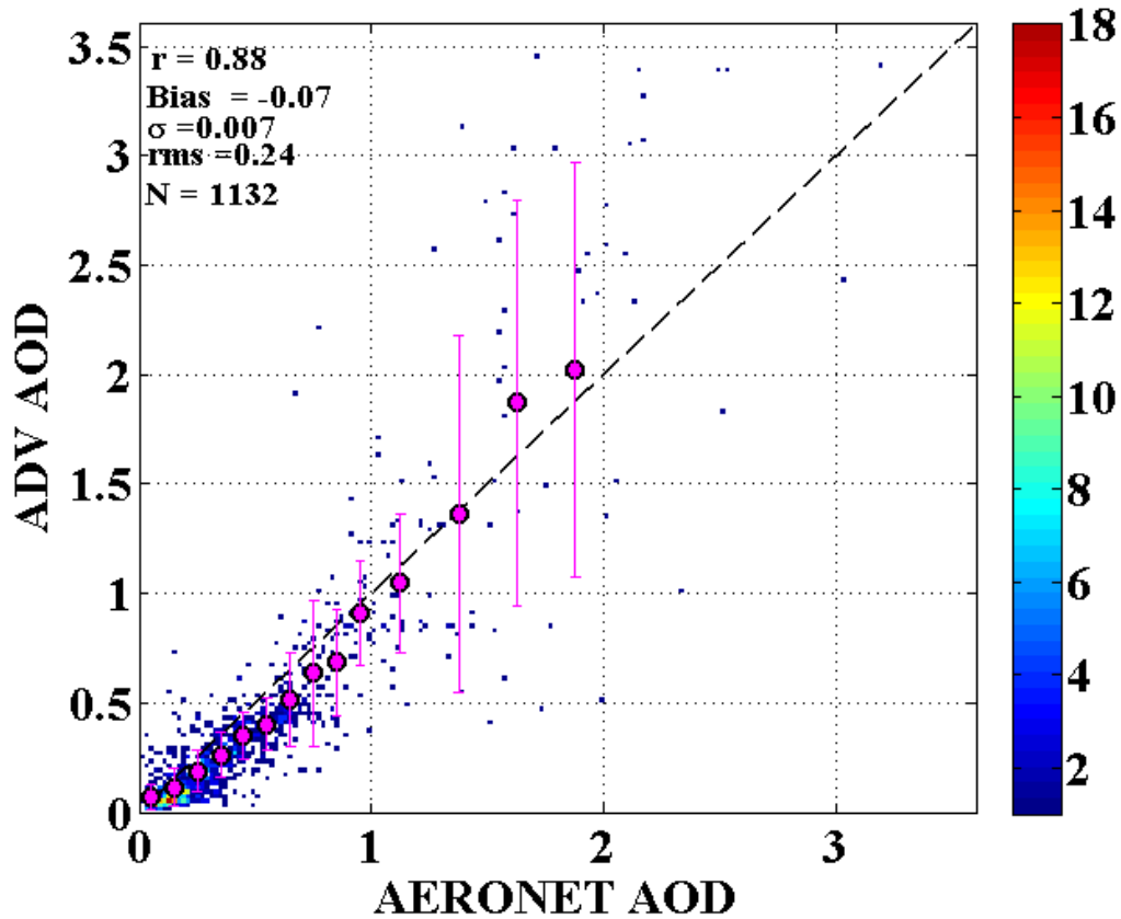
5 Figure 7. Density scatterplot of ATSR-retrieved AOD, using ADV v2.31, over China for the years 2002-2012, versus AOD from AERONET stations in mainland China (cf. Fig. 1 and Table S1). The filled circles are the averaged ATSR AOD binned in 0.1 AERONET AOD intervals (0.2 for AERONET AOD>1.0) and the vertical lines on each circle represent the 1-sigma standard deviation of the fits. Statistics in the upper left corner indicate correlation coefficient r , bias, standard deviation, root mean square (rms) error and number of data points ( N ). The colour bar on the right 10 indicates the number of data points.
