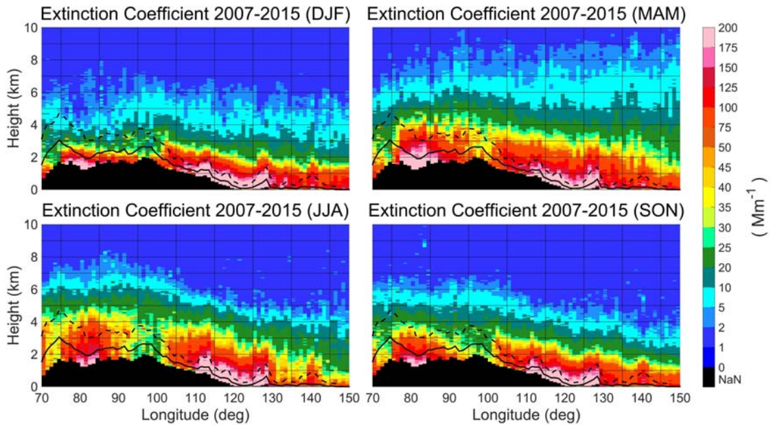
5 Figure 6. Vertical distribution of the climatological extinction coefficient profiles at 532 nm over the area 35°-45° N, 70°-150° E, including the Taklimakan desert and the Beijing-Tianjin-Hebei area, derived from 9 years of CALIOP measurements (2007-2015): winter (DJF), spring (MAM), summer (JJA) and autumn (SON). The solid and broken lines indicate the mean and maximum elevation of the aerosol extinction above the surface.
