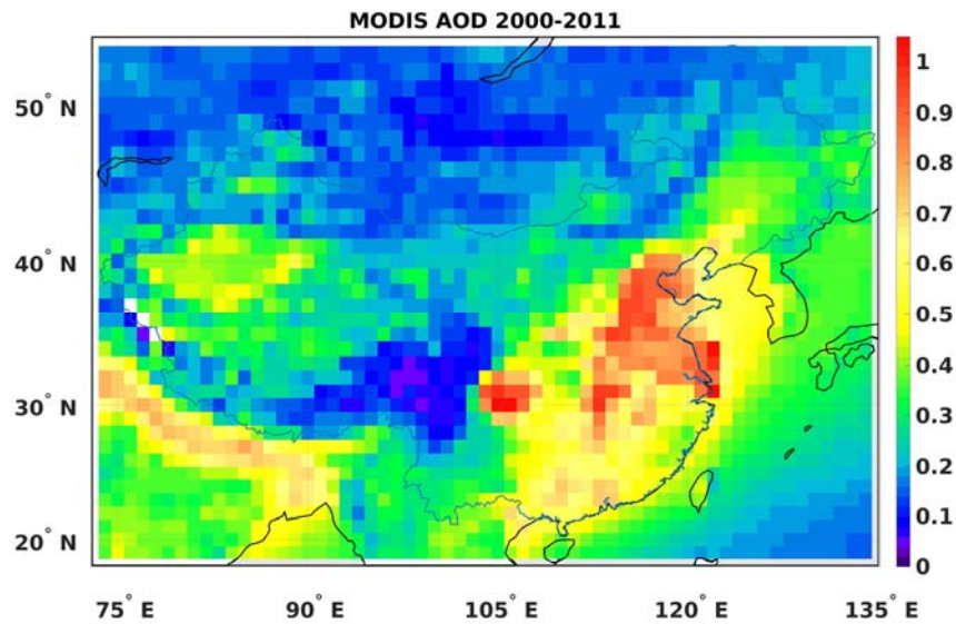
Figure 3. Spatial distribution of the MODIS/Terra C6 DTDB merged AOD over China, aggregated for the full years 2000-2011.
