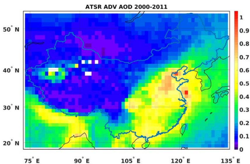
Figure 2. Spatial distribution of the AOD over China, aggregated over the (full) years 2000-2011. The AOD has been retrieved from ATSR-2 and AATSR data, using the ADV algorithm v2.31. The AOD scale is presented in the colour bar to the right of the map. Areas for which no data are available are shown in white.
