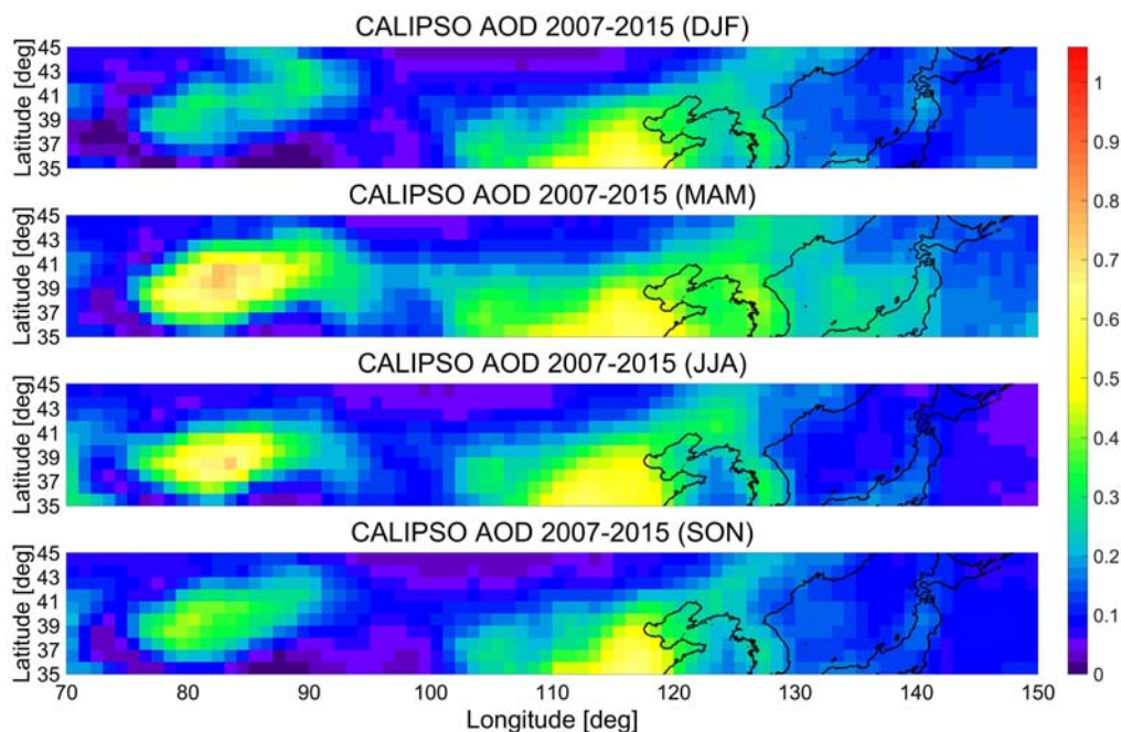
Figure 5. Seasonal maps of AOD at 532 nm derived from CALIOP over the area 35°-45° N, 70°-150° E, including the Taklimakan/Gobi deserts and the Beijing-Tianjin-Hebei area, derived from 9 years of CALIPSO overpasses (2007-2015): winter (DJF), spring (MAM), summer (JJA) and autumn (SON).
