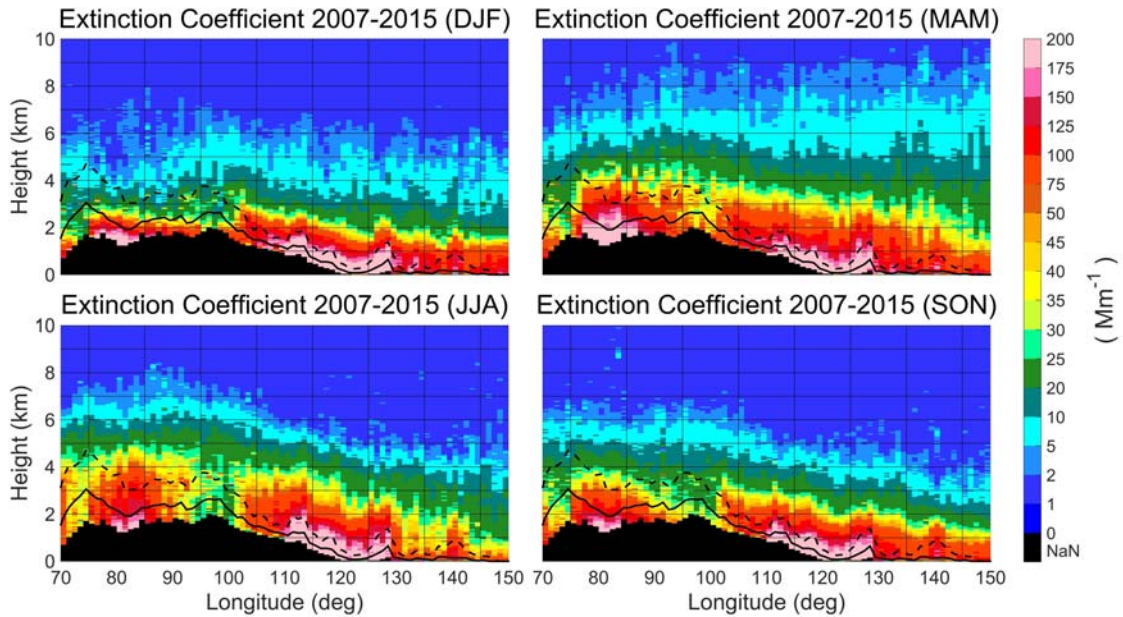
Figure 6. Vertical distribution of the climatological extinction coefficient profiles at 532 nm over the area 35°-45° N, 70°-150° E, including the Taklimakan desert and the Beijing-Tianjin-Hebei area, derived from 9 years of CALIOP measurements (2007-2015): winter (DJF), spring (MAM), summer (JJA) and autumn (SON). The solid and broken lines indicate the mean and maximum elevation of the aerosol extinction above the surface.
