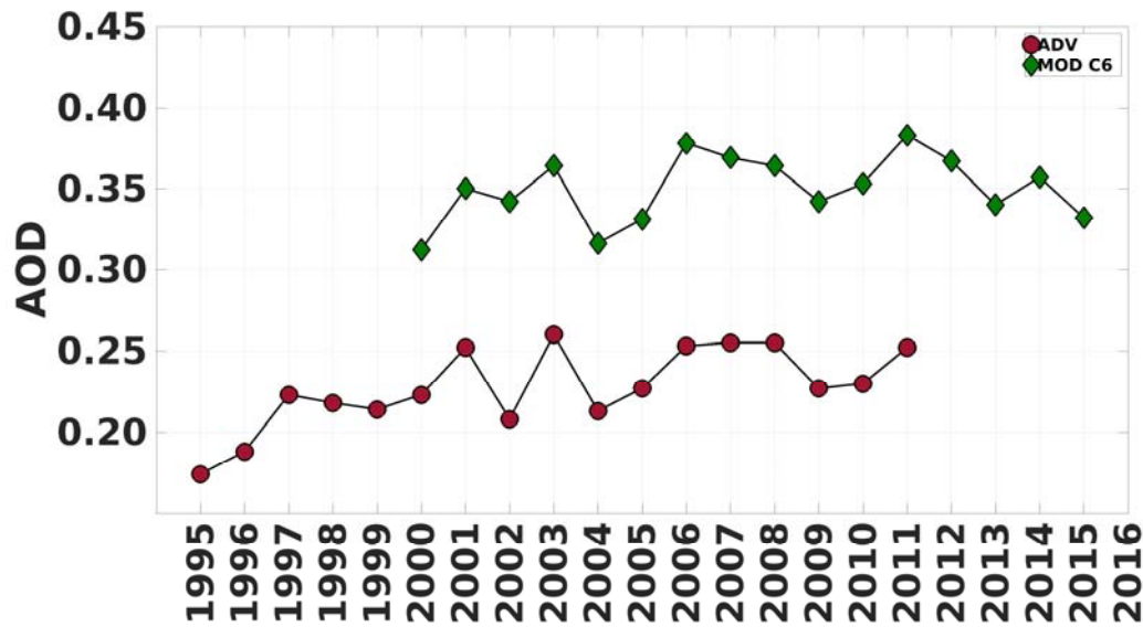
Figure 12. Time series of ATSR and MODIS retrieved AOD over China for two decades: 1995-2015. Note that data are missing in the beginning of the ATSR-2 observation period in 1995, and also MODIS/Terra data are available starting in April 2000; AATSR data start in May 2002. Therefore, the ATSR-2 1995 data point includes data for June-December and for 1996 July-December are included. ATSR-2 was used for 1995-7/2002, for 8/2002-2011 AATSR data were used. AATSR for 2012 is not shown since only 3 months of data are available, mainly in the winter (JFM) with low coverage. The MODIS 2000 data point includes data from April to December.
