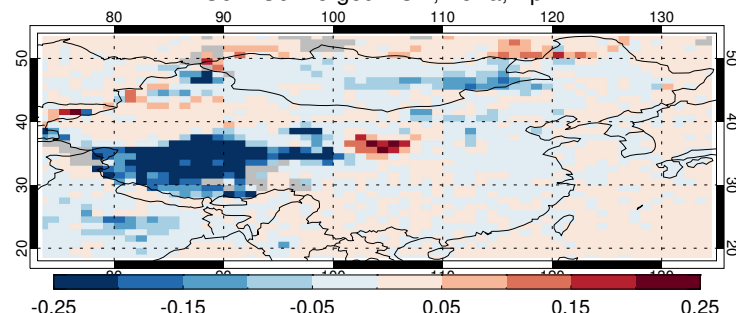
C6.1-C6 merged AOD, Terra, May
