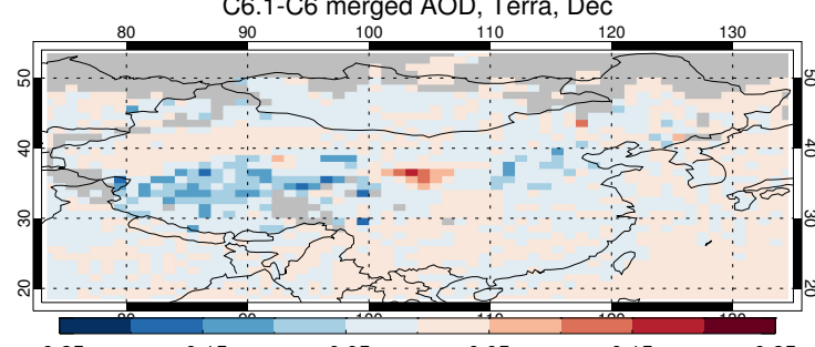
C6.1-C6 merged AOD, Terra, Dec
