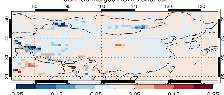
C6.1-C6 merged AOD, Terra, Aug
