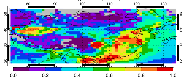
C6.1 merged AOD, Terra, Apr
