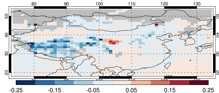
C6.1-C6 merged AOD, Terra, Feb
