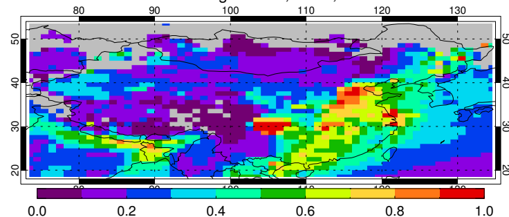
C6.1 merged AOD, Terra, Mar
