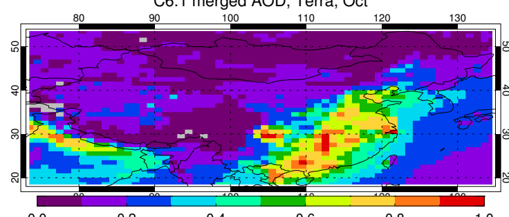
C6.1 merged AOD, Terra, Nov
