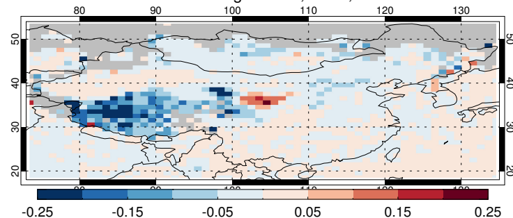
C6.1-C6 merged AOD, Terra, Mar
