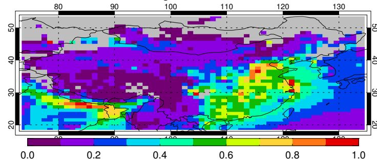
C6.1 merged AOD, Terra, Feb
