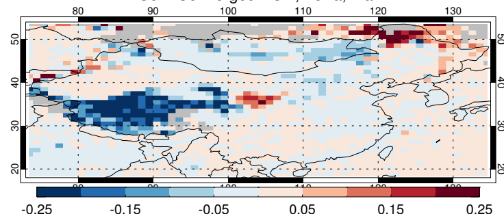
C6.1-C6 merged AOD, Terra, Apr
