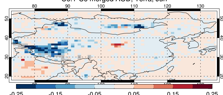
C6.1-C6 merged AOD, Terra, Jul
