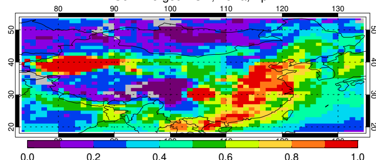
C6.1 merged AOD, Terra, May
