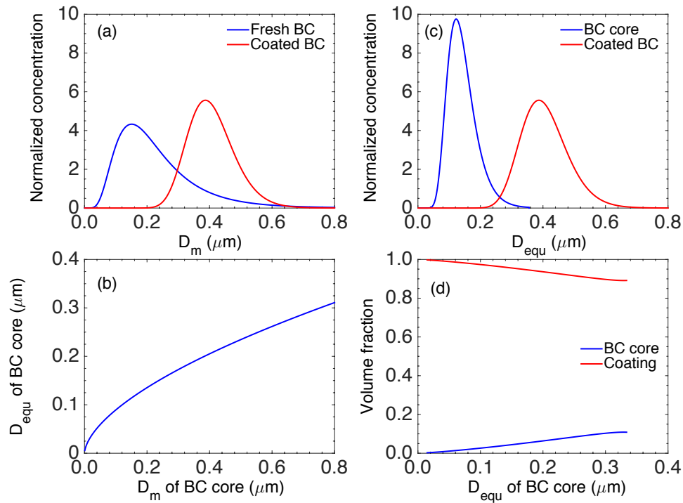
5 Figure 2. (a) Normalized particle number concentration of uncoated (i.e. fresh) and coated (after 24-hour coating) BC, assuming lognormal size distribution and utilizing a laboratory experiment by Schnaiter et al. (2005; see Fig. 5 of their study). (b) Estimated relationship between the diameter of equivalent volume sphere ( D_{\text{equ}} ) and mobility diameter ( D_m ) for Fresh BC aggregates. (c) The size distributions for the diameters of the equivalent volume spheres ( D_{\text{equ}} ) of BC core and Coated BC after 24-hour coating, based on (a) and (b). (d) Estimated volume fractions of BC core and coating material as a function of D_{\text{equ}} of BC core, based on (c).
