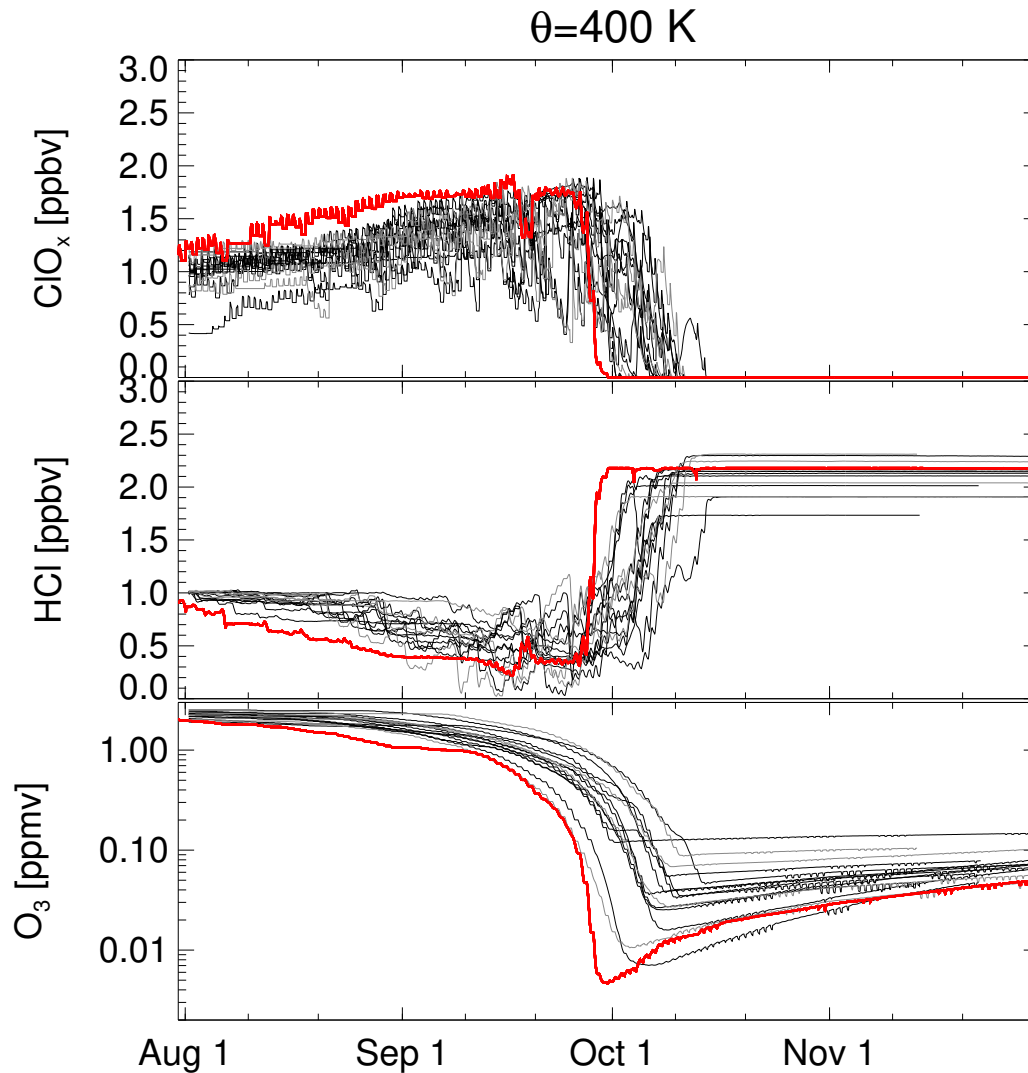
Figure 4. Results from multi-trajectory simulations of CLaMS. Box-model simulations were performed for a set of trajectories passing the South pole at 400 K taken from (Grooß et al., 2011) Grooß et al. (2011) . The box-model simulations cover the time period from 1 August to 30 November 2003. A few trajectories showing very little diabatic descent (and thus much smaller values of total chlorine) were neglected. Initial values were chosen consistently with the reference run (Fig. 1), which is shown here in red . Individual trajectories are shown in different shades of grey to allow them to be distinguished more easily.
