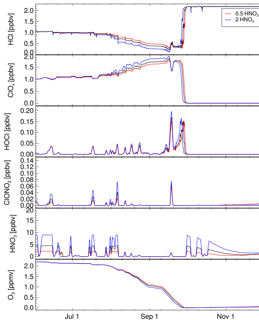
Figure A2. Simulation for the impact of denitrification. The impact of denitrification is tested by initialising the model run with \text{HNO}_3 doubled ( blue line ) and halved ( red line ). Black line shows the results of the reference simulation.
