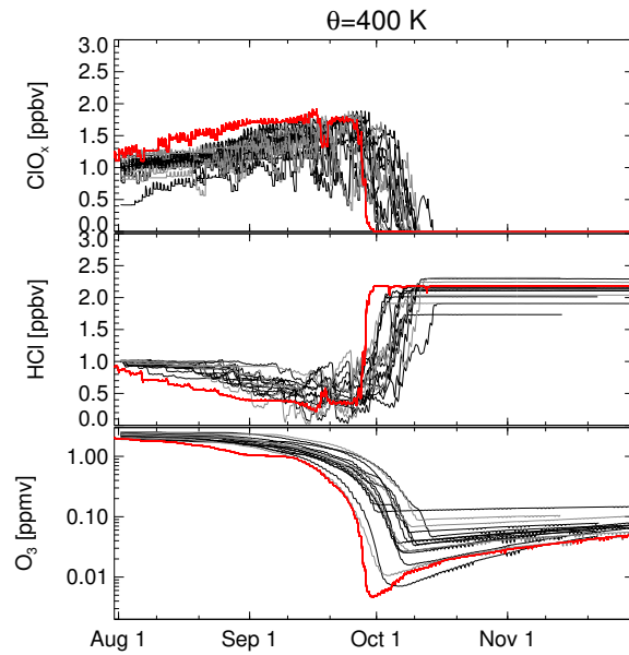
Figure 2: Results from multi-trajectory simulations of CLaMS. Box-model simulations were performed for a set of trajectories passing the South pole at 400 K taken from (Groß et al., 2011). The box-model simulations cover the time period from 1 August to 30 November 2003. A few trajectories showing very little diabatic descent (and thus much smaller values of total chlorine) were neglected. Initial values were chosen consistently with the reference run (Fig. 1), which is shown here in red. Individual trajectories are shown in different shades of grey to allow them to be distinguished more easily.
