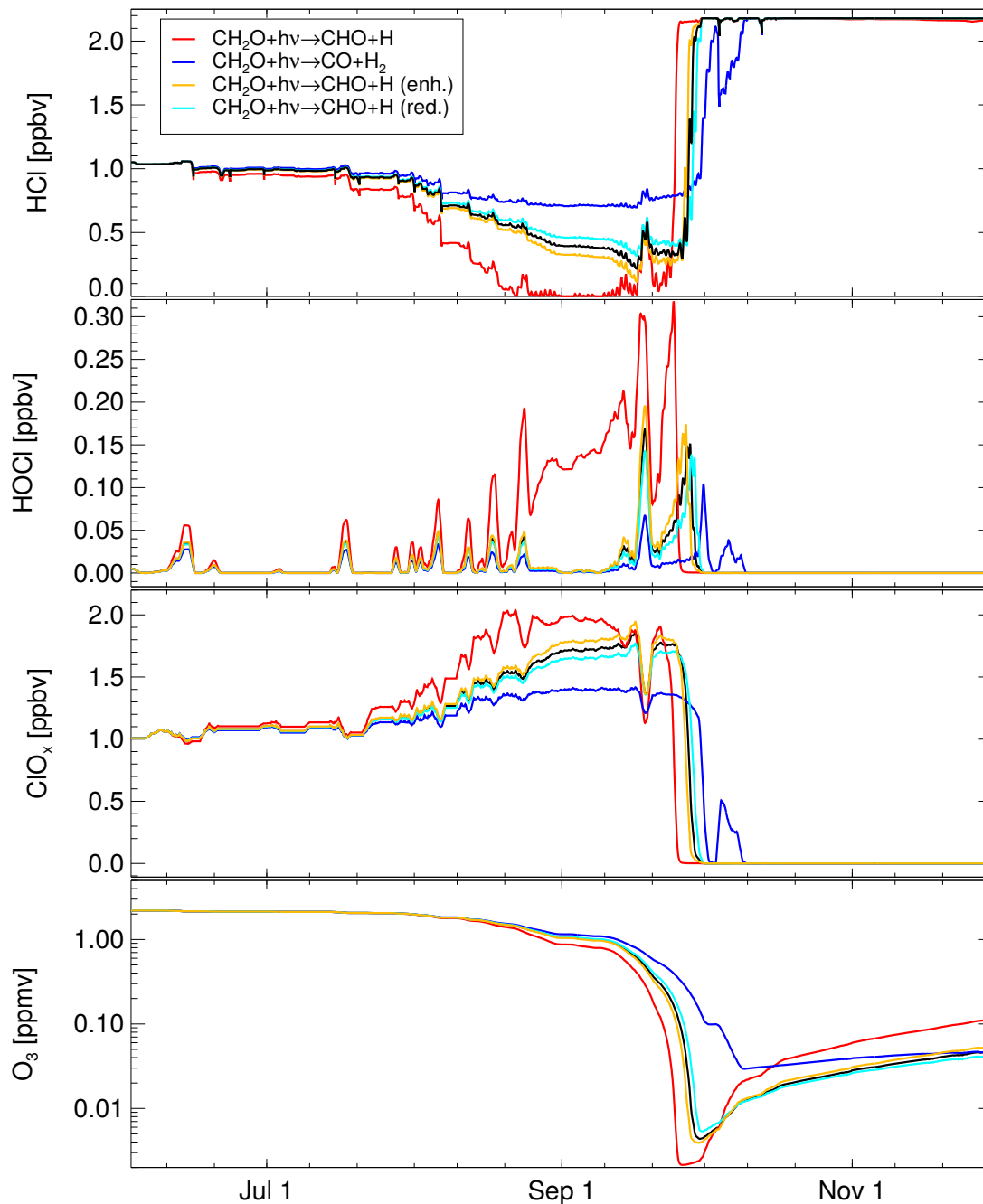
Figure 2. Sensitivity of the ozone hole chemistry on \text{HO}_2 production in the photolysis of \text{CH}_2\text{O} . Black lines show the reference case, red line a case assuming 100% efficiency for \text{HO}_2 production (i.e. for reaction R14), and dark blue line a case assuming no \text{HO}_2 production in the photolysis of \text{CH}_2\text{O} (100% efficiency for reaction R22). The light blue and yellow line show a more realistic estimate of the kinetic uncertainties, namely branching ratio for the radical channel enhanced by 20% (yellow line) and reduced by 20% (light blue line).
