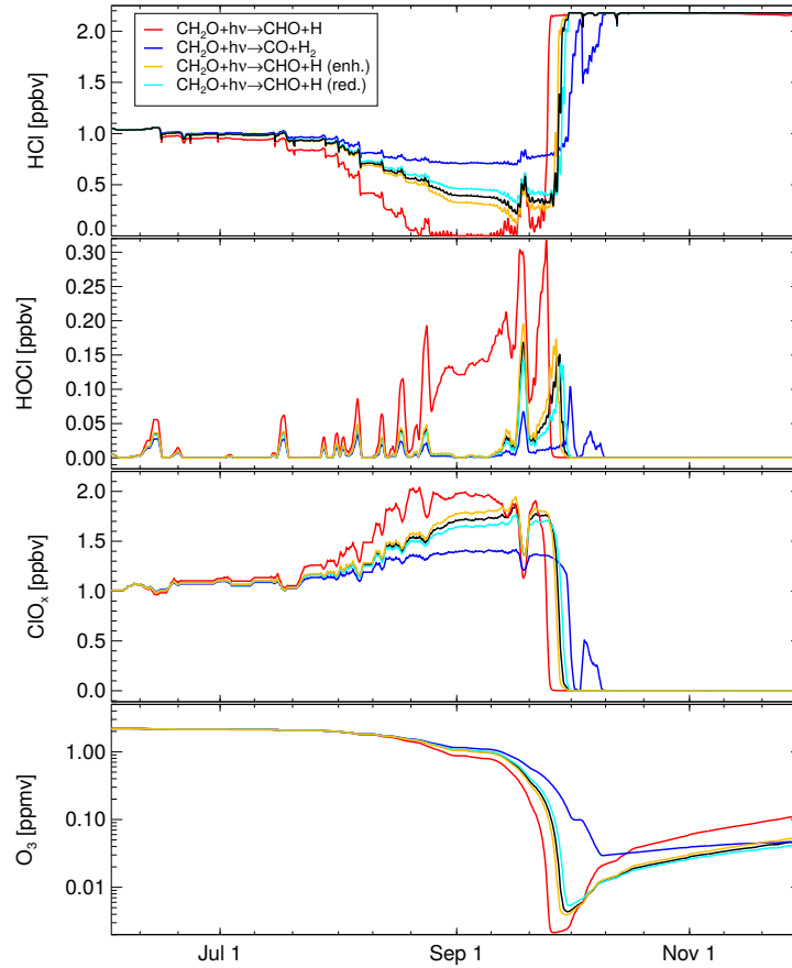
Figure 1: Improved version of Fig. 2 showing the effect of realistic estimates of the uncertainty of the branching ratio of the formaldehyde photolysis (light blue and yellow lines). The original upper and lower limits (red and dark blue lines) are retained. Black line shows the reference case.
