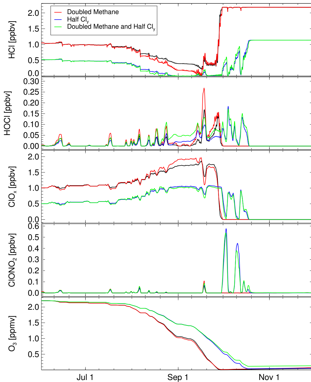
Figure 3. Sensitivity of the ozone hole chemistry on stratospheric methane and chlorine levels. Black lines show the reference case, red line a case assuming initial methane to be doubled, blue line a case assuming initial inorganic chlorine (Cl y ) to be halved, and green line a case for initial methane doubled and Cl y halved.
