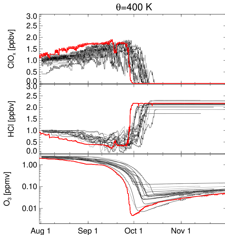
Fig. 2. Results from multi-trajectory simulations of CLaMS. Box-model simulations were performed for a set of trajectories passing the South pole at 400 taken from GroöB, et al. 2011.
