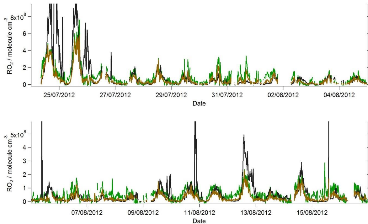
Figure S1: Observed (coloured lines) and MCM-BASE modelled (black lines) \text{RO}_2 during the summer ClearfLo IOP. Brown = [\text{RO}_2]_{\text{CORR}} (see Eqn.11) and dark-green = [\text{RO}_2]_{\text{NON-CORR}} (see Eqn.12). Data time resolution of each data point is 15 minutes.
