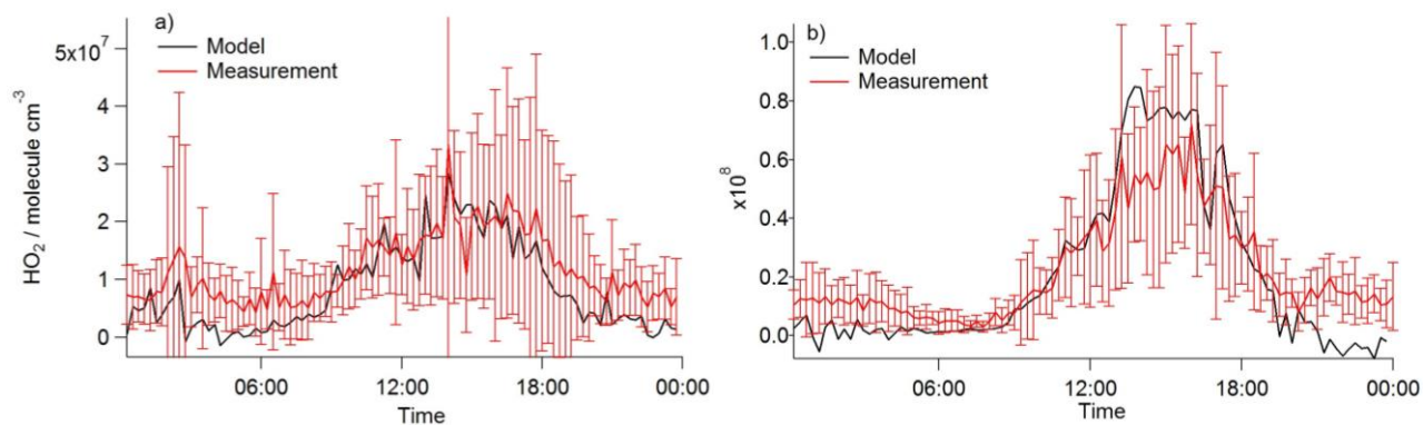
Figure 12: Average diel profiles of HO 2 concentration observed (red line with error bars) under a) south-westerly and b) easterly conditions. Overlaid is HO 2 calculated using the solution to the HO 2 quadratic expression (E7) (represented by the black line) with \alpha equal to 0.15.
