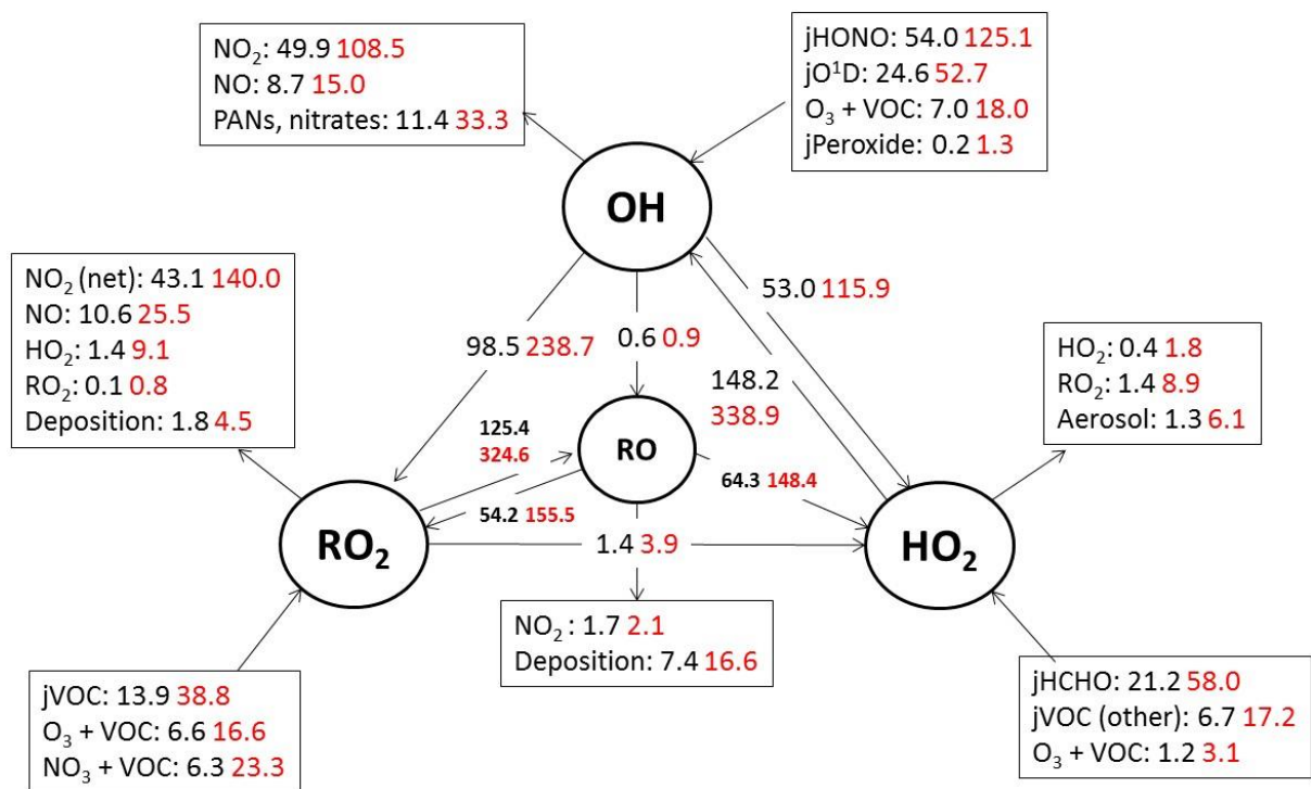
Figure 7: Mean daytime (6am – 9pm) rates of reaction for formation, propagation and termination of radicals in units of 10^5 \text{ molecule cm}^{-3} \text{ s}^{-1} for south westerly (black) and easterly (red) air masses.
