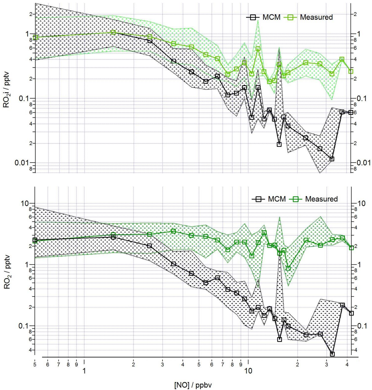
5 Figure 10: Observed and modelled RO x behaviour as a function of NO for the whole campaign period. (a) Median RO 2i measured (green squares), RO 2i modelled (black squares). (b) Median RO 2 measured (green squares), RO 2 modelled (black squares). Patterned areas represents the 25/75 th percentiles. Data are filtered for daytime hours between 6 am and 7 pm and binned by [NO] with a bin width = 1 ppbv for [NO] between 0 – 20 ppbv and bin width = 5 ppbv for [NO] between 20 – 45 ppbv.
