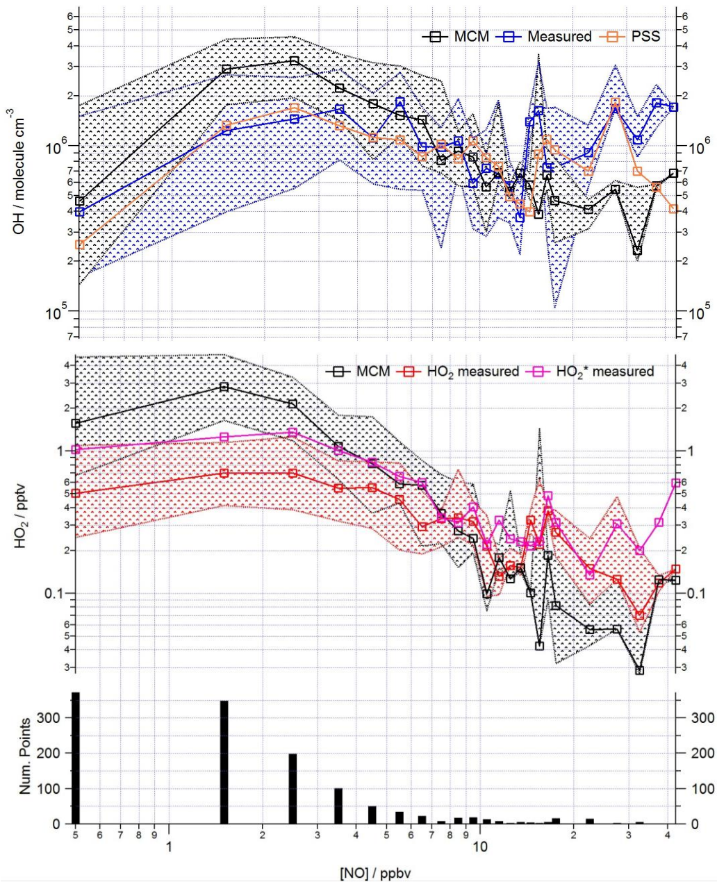
5 Figure 8: Observed and modelled HO x behaviour as a function of NO for the whole campaign period. (a) Median OH measured (blue squares), OH modelled (base MCM model = black squares, steady state calculation = orange squares). (b) Median HO 2 measured (red squares), HO 2 * measured (pink squares), HO 2 modelled (black squares). Patterned areas represents the 25/75 th percentiles. Data are filtered for daytime hours between 6 am and 7 pm and binned by [NO] with a bin width = 1 ppbv for [NO] between 0 – 20 ppbv and bin width = 5 ppbv for [NO] between 20 – 45 ppbv. The number of points in each bin is displayed in the lower panel.
