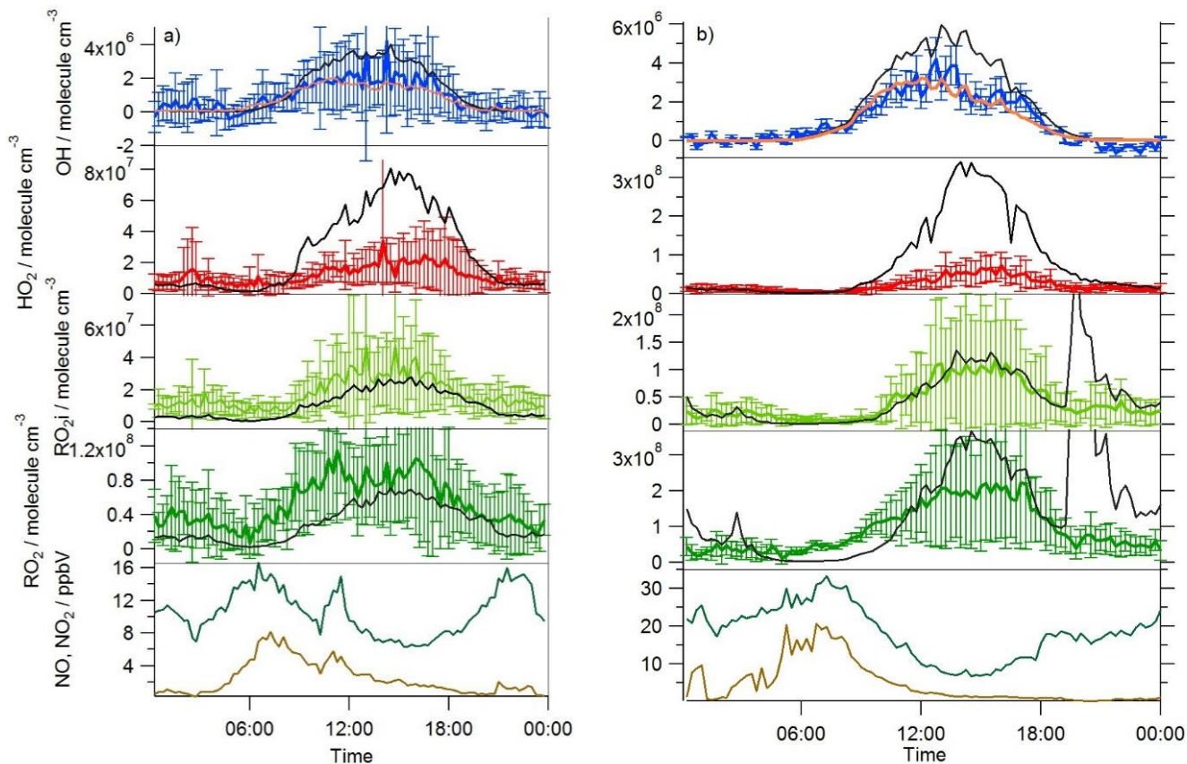
Figure 3: Average diel observed (coloured lines with error bars) and MCM-BASE (black line) OH, HO 2 , RO 2 i and RO 2 profiles during a) south-westerly and b) easterly flows; [OH] PSS is displayed by the orange line. The error bars represent the 1 \sigma variability in the observations. The average diel observed NO (brown line) and NO 2 (green line) are displayed in the bottom panels.
