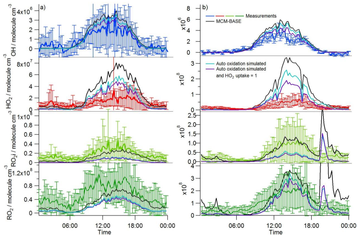
Figure 11: Average diel observed and modelled HO x profiles during a) south-westerly and b) easterly flows. The base model predictions are represented by the black line. The model scenario run with standard VOC species only and missing reactivity represented by converting OH to C 6 H 5 O 2 is represented by the pale blue line; the purple line represents the model scenario run with standard VOC species only and missing reactivity represented by converting OH to C 6 H 5 O 2 and an enhanced heterogeneous loss of HO 2 , \gamma_{HO_2} = 1 .
