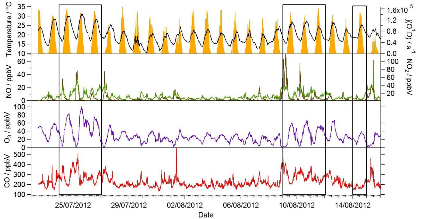
5 Figure 1: Observed temperature (black line), j(\text{O}^1\text{D}) (yellow area), NO (brown line), NO 2 (green line), O 3 (purple line) and CO (red line) mixing ratios during the summer ClearfLo IOP. Data time resolution is 15 minutes. Periods of Easterly flow are highlighted inside the black boxes.
