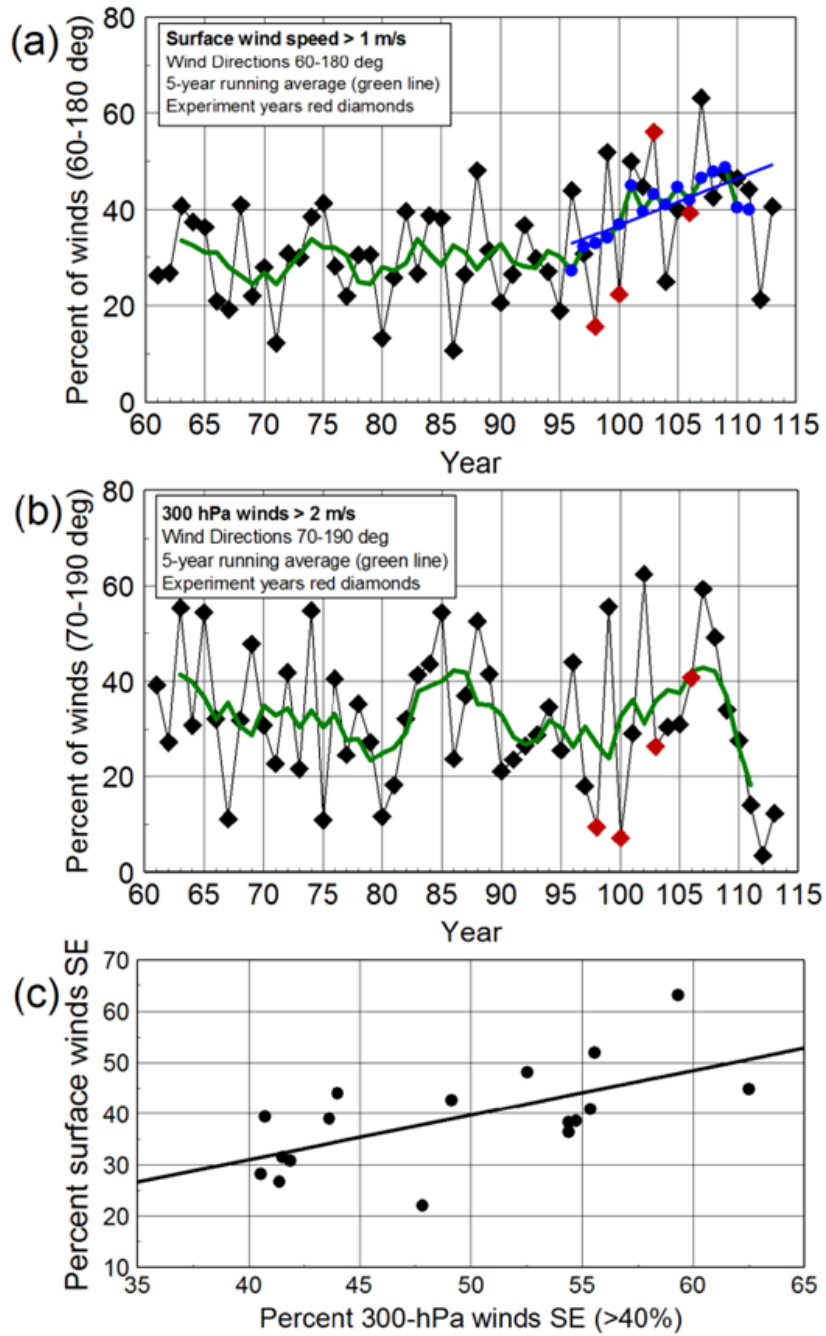
Figure S3. (a) Percent of surface winds from the SE for Late Spring Days 310-340 ( 60^{\circ} - 180^{\circ} corresponding to higher NO in Figure 4 and wind speed > 1\text{ms}^{-1} ). Five-year running average and experiment years are highlighted. The recent trend is highlighted with r^2=0.6 . (b) Same as (a) but for 300-hPa winds. (c) Scatter plot of surface wind percentages for frequency of occurrence of 300-hPa SE wind directions >40\% . Least squares linear regression produces r^2=0.4
