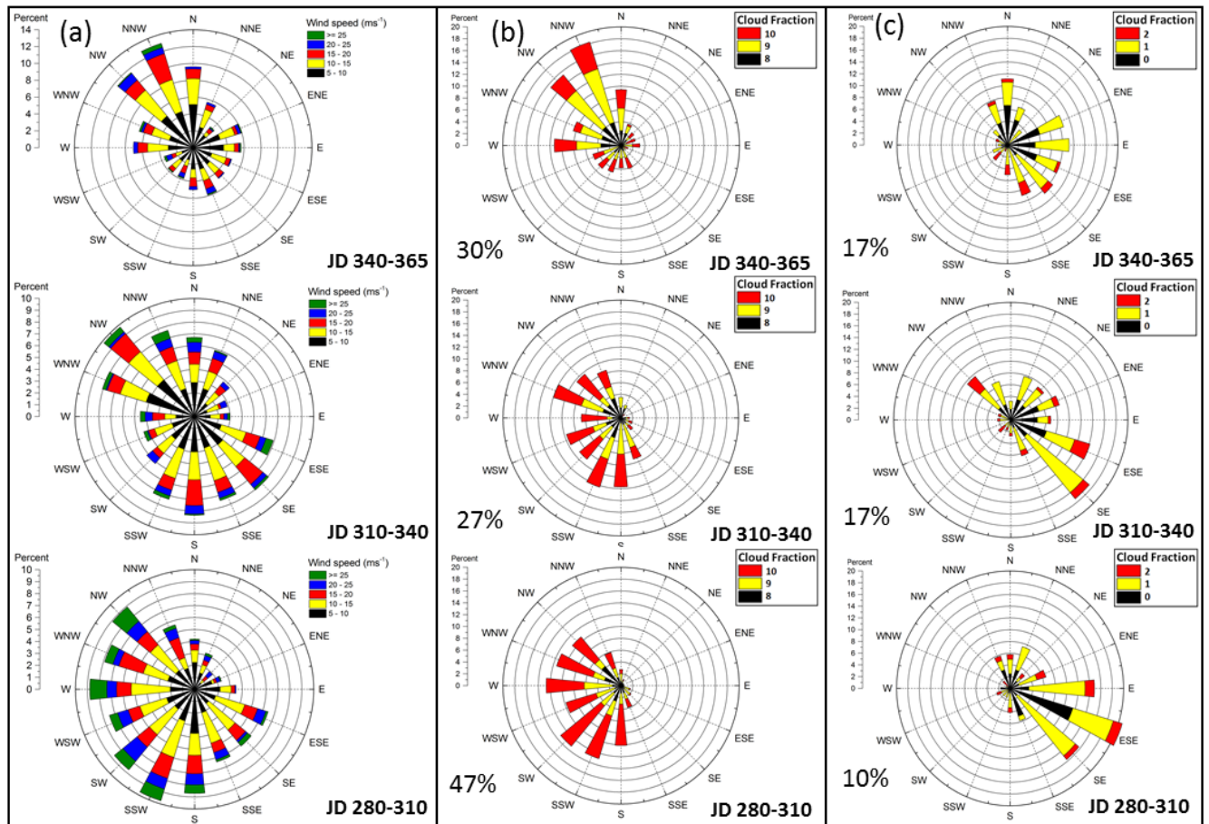
Fig S1. a) Distribution of wind speed and direction at 300 hPa by subseason in 22.5° bins (Note Fig. 2 uses 45° bins), b) Distribution for mostly overcast conditions ( \geq 8/10 ths cloud fraction) by 300 hPa wind direction within each subseason. c) Distribution mostly clear conditions ( \leq 2/10 ths cloud fraction) by 300-hPa wind direction by subseason. Daily observed average cloud fraction was used: For extreme high and low cloud fraction this provides reasonable assurance of the observed cloud fraction persisted for both rawinsonde launches. Wind data were restricted to 300-hPa wind speeds > 5 \text{ ms}^{-1} . Period of data was 1991-2013. The period October-December generally had twice-a-day rawinsondes. Percentages are based on the total number of observations in each ~30-day interval.
