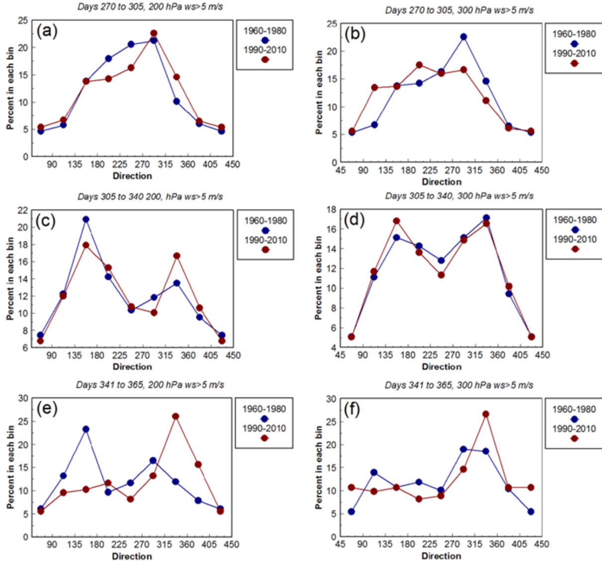
Figure S7. Wind direction distributions at 200 hPa (left) and 300hPa (right) for years 1960-1980 and 1990-2010 and within seasons: Days 270-305 (top: a,b), Days 305-340 (middle: c,d) and Days 341-365(bottom: e,f). Wind speeds > 5 \text{ ms}^{-1} only were used. Note that slightly different periods were used compared to those in Figure 2. Note the major difference in distributions for early summer, Days 341-365 at 200 hPa. As noted in Neff (1999), the early period is dominated by a strong thermal tropopause above 300 hPa that could decouple winds between 300 and 200 hPa.
