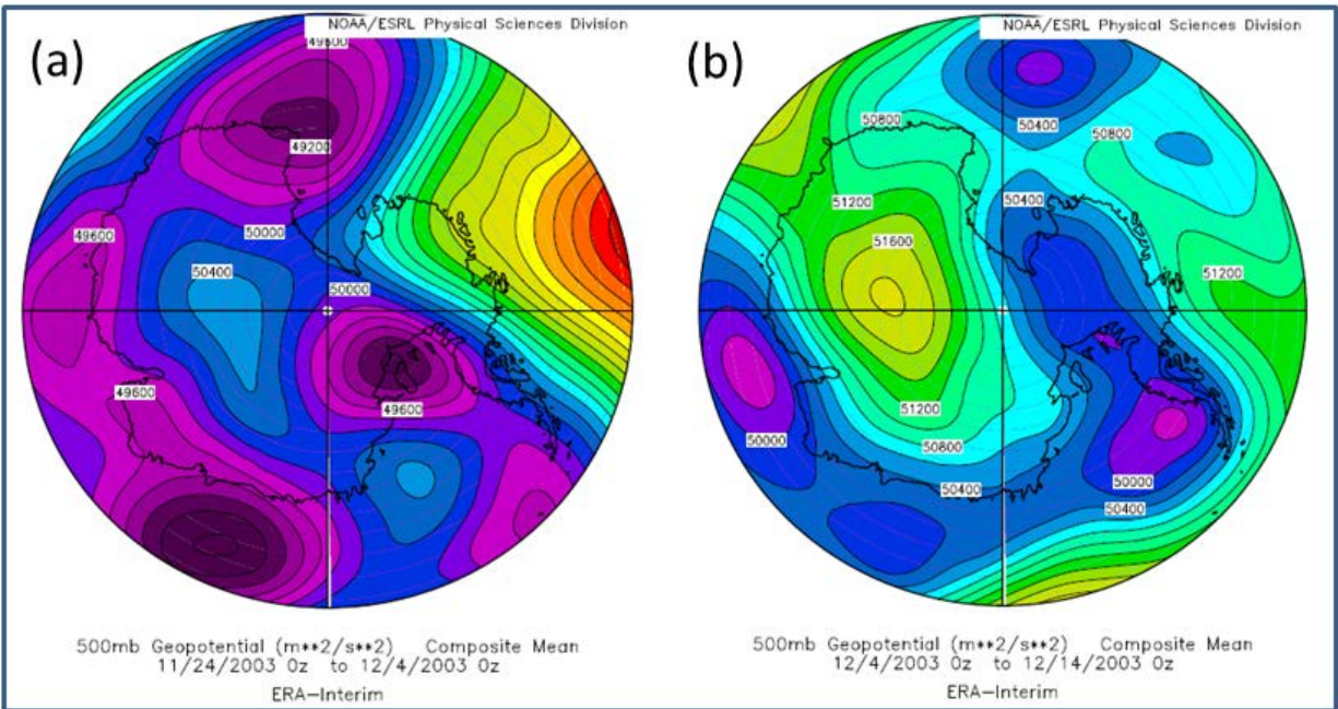
Figure S11. 500 hPa geopotential field for the ten days (a) before and (b) after 12/4/2003. The pattern on the right corresponds to the circulation highlighted by (Arimoto et al. 2008) that emphasizes the counterclockwise circulation dominating the high plateau and conducive to transport from maritime regions.
