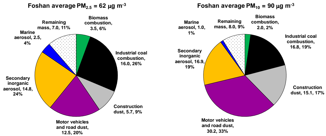
Figure 4. Source contributions to PM at Foshan showing the average concentrations of PM_{2.5} , PM_{10} (in \mu g m^{-3} ) during the monitoring period.
