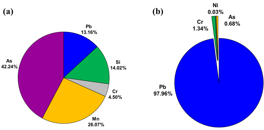
Figure 9. (a) average contribution percentage of selected trace elements to Hazard Index (HI) and (b) average contribution percentage of selected trace elements to total carcinogenic risk (CR).
