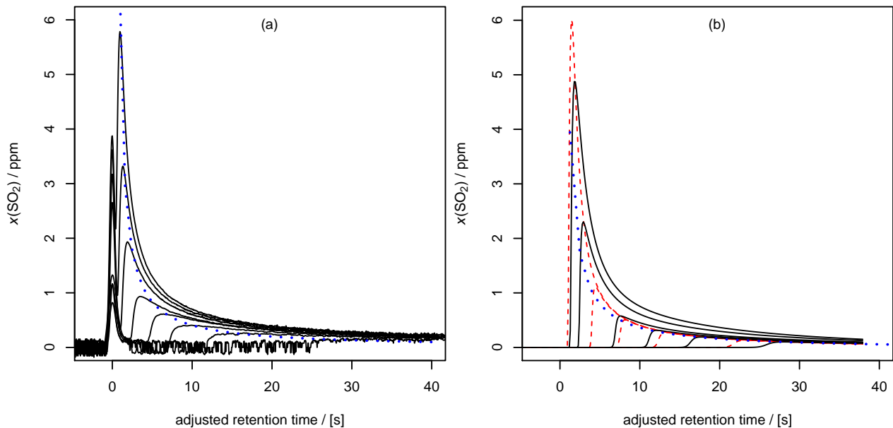
Figure 2. (a) Chromatograms from injection of various amounts of a SF 6 /SO 2 mixture at 247 K and 2 μm ice film thickness. (b) Simulated SO 2 chromatograms using the Temkin isotherm with \zeta = 4.3 \times 10^{-9} \text{ mol m}^{-2} , K_T = 10^{-6} \text{ mol m}^{-2} \text{ Pa}^{-1} , K_H = 2.8 \times 10^{-9} \text{ mol m}^{-2} \text{ Pa}^{-1} using 100 cells in axial direction. Dashed lines: simulation without absorption/diffusion into the solid phase. Solid lines: simulation including diffusion into the solid phase with H = 50 , D_s = 2 \times 10^{-13} \text{ m}^2 \text{ s}^{-1} using 30 cells in radial direction. The dotted lines are calculated with Eq. (1). They represent the locations of the experimental peak maxima.
