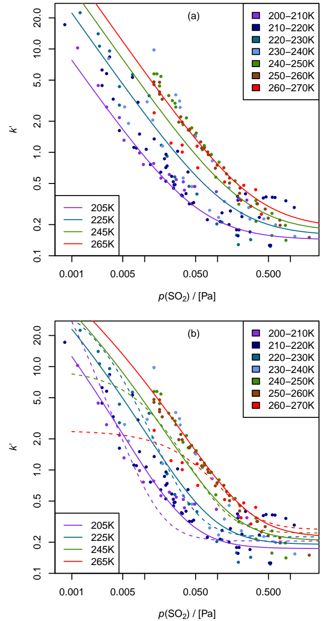
Figure 3. Double logarithmic plot of k' vs. p(\text{SO}_2) at peak maximum for experiments with ice film thickness h > 4 \text{ μm} and without ice aging. (a) Fit with Temkin adsorption isotherm according to Eq. (7). (b) Fit with simple Langmuir model (dashed lines) according to Eq. (10) and with the dissociative Langmuir model (solid curves) according to Eq. (16).
