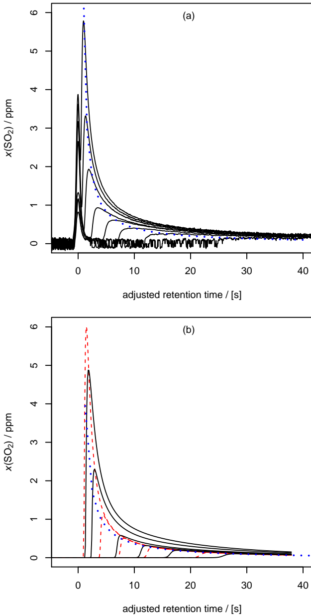
Figure 2. (a) Chromatograms from injection of various amounts of a SF 6 /SO 2 mixture at 247 K and 2 μm ice film thickness. (b) Simulated SO 2 chromatograms using the Temkin isotherm with \zeta = 4.3 \times 10^{-9} \text{ mol m}^{-2} , K_T = 10^{-6} \text{ mol m}^{-2} \text{ Pa}^{-1} , K_H = 2.8 \times 10^{-9} \text{ mol m}^{-2} \text{ Pa}^{-1} using 100 cells in axial direction. Dashed lines: simulation without absorption/diffusion into the solid phase. Solid lines: simulation including diffusion into the solid phase with H = 50 , D_s = 2 \times 10^{-13} \text{ m}^2 \text{ s}^{-1} using 30 cells in radial direction. The dotted lines are calculated with Eq. (1). They represent the locations of the experimental peak maxima.
